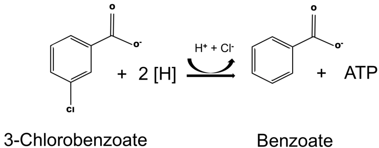
Figure 2.4. Reductive dechlorination of 3-chlorobenzoate (3-CB) by Desulfomonile tiedjei .
