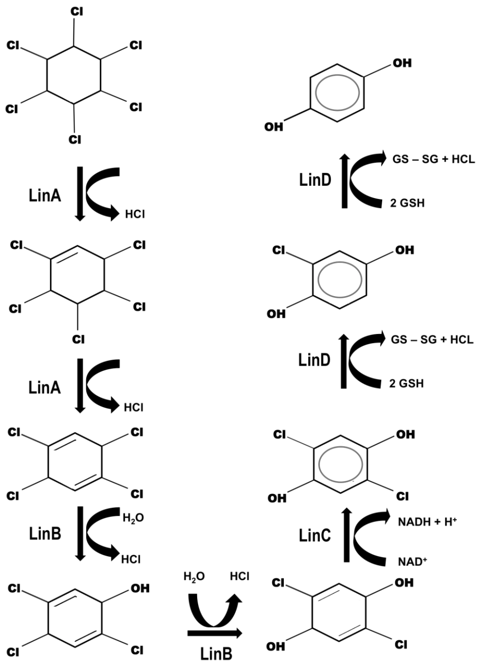
Figure 2.3 \gamma -hexachlorocyclohexane dechlorination in Sphingomonas paucimobilis UT26.
