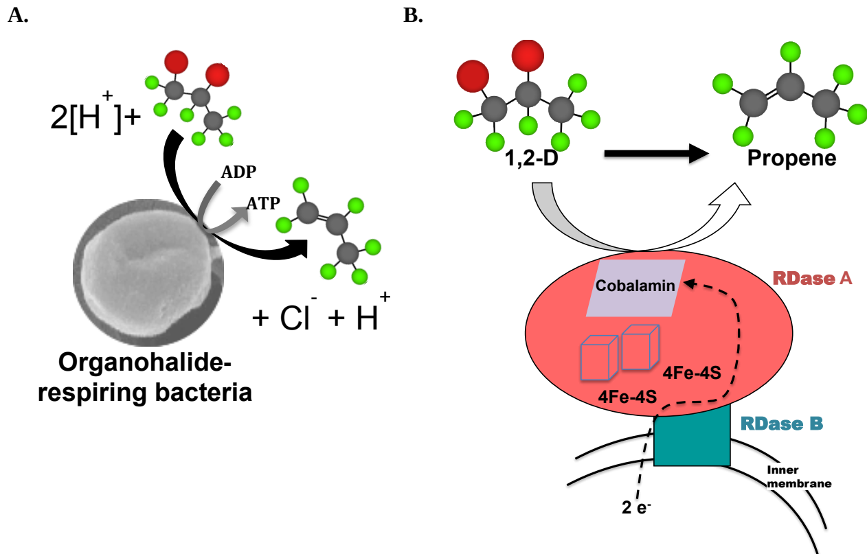
Figure 2.2. Physiology of organohalide respiration
