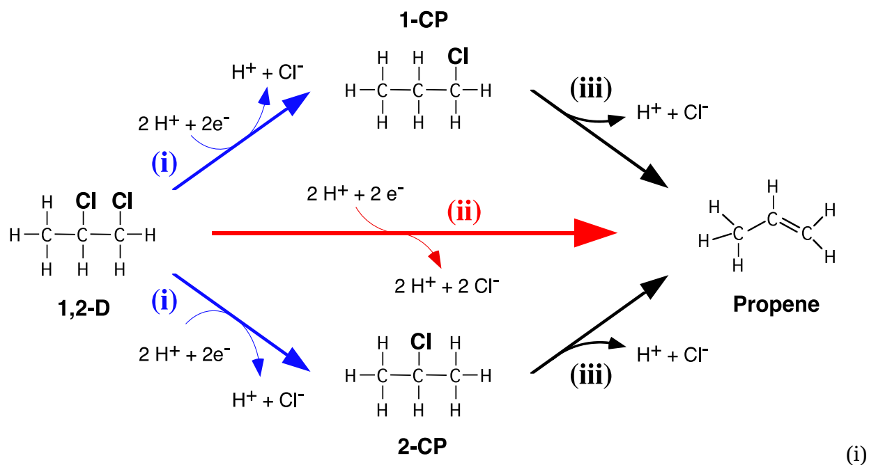
Figure 2.6. Anaerobic dechlorination pathway of 1,2-D in microcosms and enrichments as described by (F E Löffler, Champine, Ritalahti, Sprague, & Tiedje, 1997). Figure from Loeffler et al. (1997). (i) Hydrogenolysis of 1,2-D leading to monochlorinated propanes followed by (iii) Dehydrochlorination resulting in the formation of propene, and (ii) dichloroelimination. Hydrogenolysis and dehydrochlorination were only detected in microcosm with sediment material. In sediment-free cultures, 1,2-D was dechlorinated to propene without the intermediate formation of monochlorinated propanes (dichloroelimination). In the RC ad KS cultures only dichloroelimination is observed.
