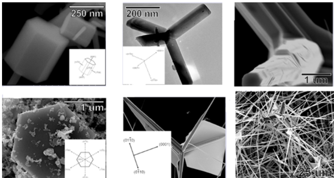
Figure 1.7: This figure illustrates some of the possible habitats or "morphologies" of zinc oxide nanoparticles ranging from 200 nm to > 2 micron.
