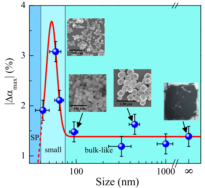
FIG. 2. Full field color contrast, |\Delta\alpha_{\max}| = |\frac{\alpha(35\text{ T}) - \alpha(0\text{ T})}{\alpha(0\text{ T})}| \times 100\% , evaluated at 11\,600\text{ cm}^{-1} (which corresponds to the maximum of the d -to- d absorption) at 4.2 K. A photo of the single crystal and scanning electron microscope images of select nanoparticles are included. The three different size regimes [bulklike, small size, and superparamagnetic (SP)] are indicated. The red line guides the eye, with the dashed region approximating what may happen at smaller sizes.
