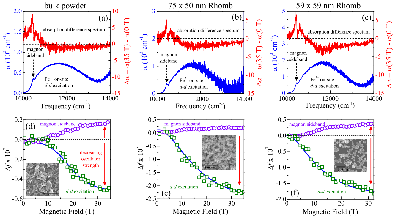
FIG. 1. (a)–(c) 4.2-K absorption spectrum of polycrystalline hematite and selected nanorhombohedral particles beneath the full field absorption difference spectrum, \Delta\alpha = \alpha(35 \text{ T}) - \alpha(0 \text{ T}) , for comparison. The full data set is available in Ref. [46]. (d)–(f) Change in oscillator strength ( \Delta f ) of the d -to- d on-site excitation (green squares) and magnon sideband (violet circles) vs magnetic field for these materials. Blue lines guide the eye.
