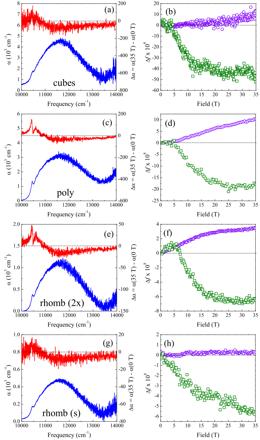
Figure S4: (left) 4.2 K absorption and 35 T magnetic field-induced absorption difference for various \alpha -Fe 2 O 3 nanoparticles. (right) Oscillator strength trends for the d-d excitation and magnon sideband for the corresponding samples.
