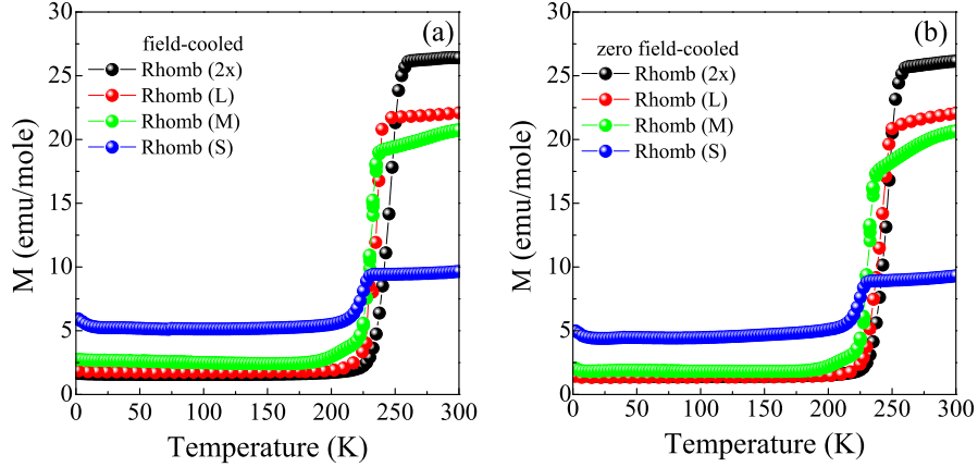
Figure S6: (a) Field-cooled and (b) zero field-cooled magnetization of the rhombohedral \alpha\text{-Fe}_2\text{O}_3 nanoparticles. Here, we employ the sample designations as given in Table 1 of the main text.
