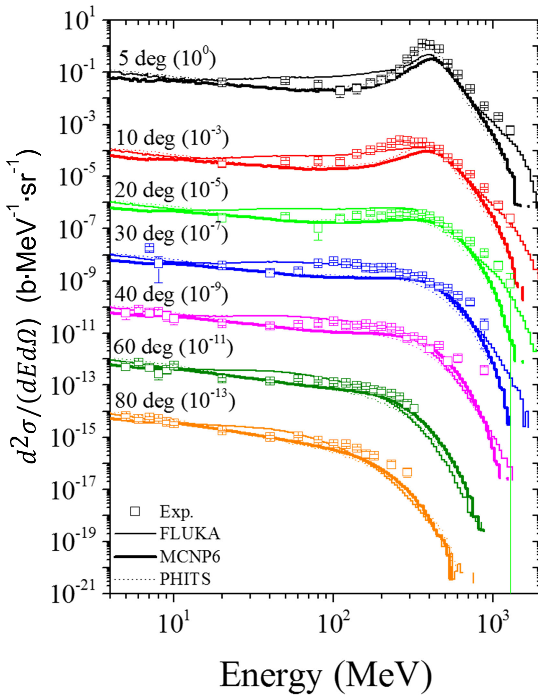
Figure 51. The neutron DDX with 400-MeV/nucleon ^{40}\text{Ar} + ^{\text{nat}}\text{Cu} target.
