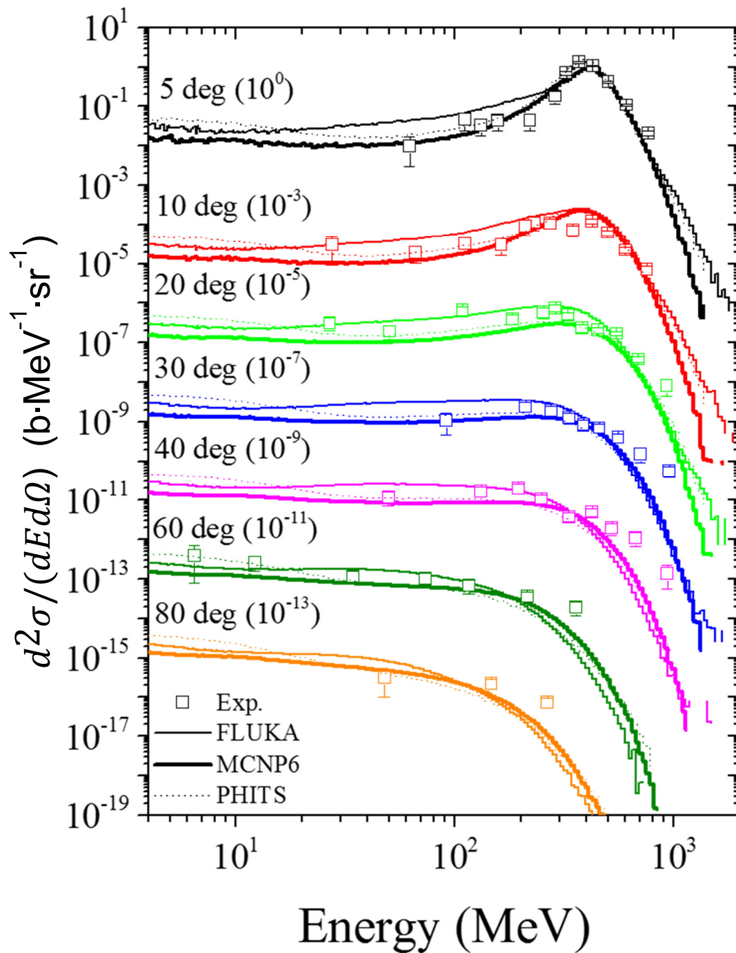
Figure 54. The neutron DDX with 400-MeV/nucleon ^{84}\text{Kr} + ^{\text{nat}}\text{Al} target.
