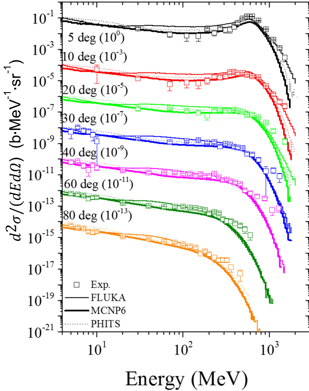
Figure 50. The neutron DDX with 600-MeV/nucleon ^{20}\text{Ne} + ^{\text{nat}}\text{Cu} target.
