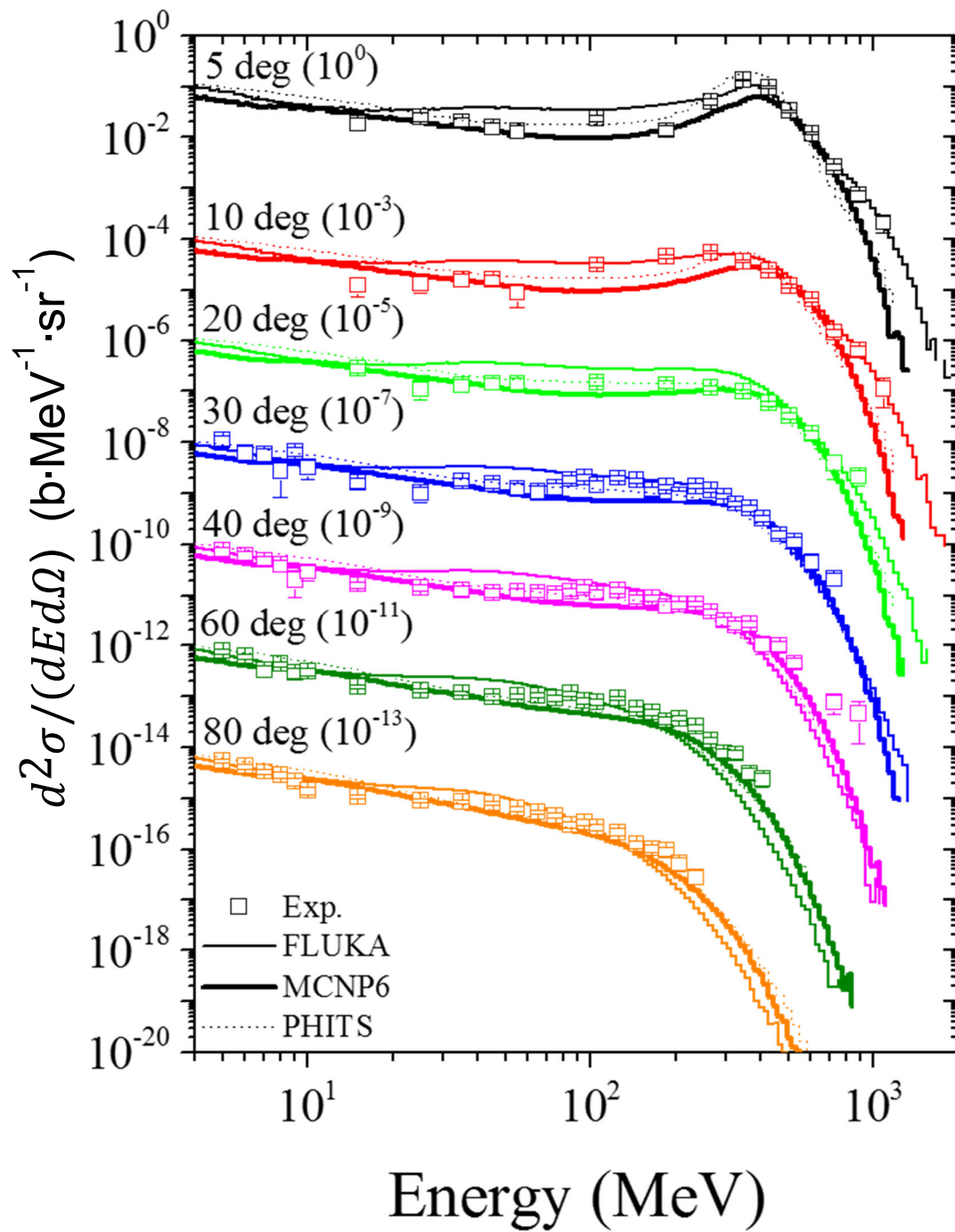
Figure 49. The neutron DDX with 400-MeV/nucleon ^{20}\text{Ne} + ^{\text{nat}}\text{Cu} target.
