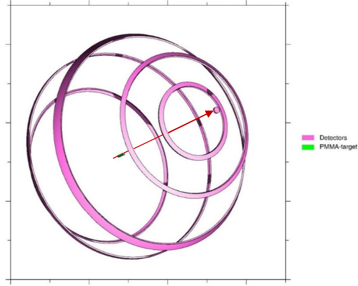
Figure 22. The geometry setup used in PHITS for 230-MeV/nucleon ^4\text{He} ions stopped in the thick PMMA target.
