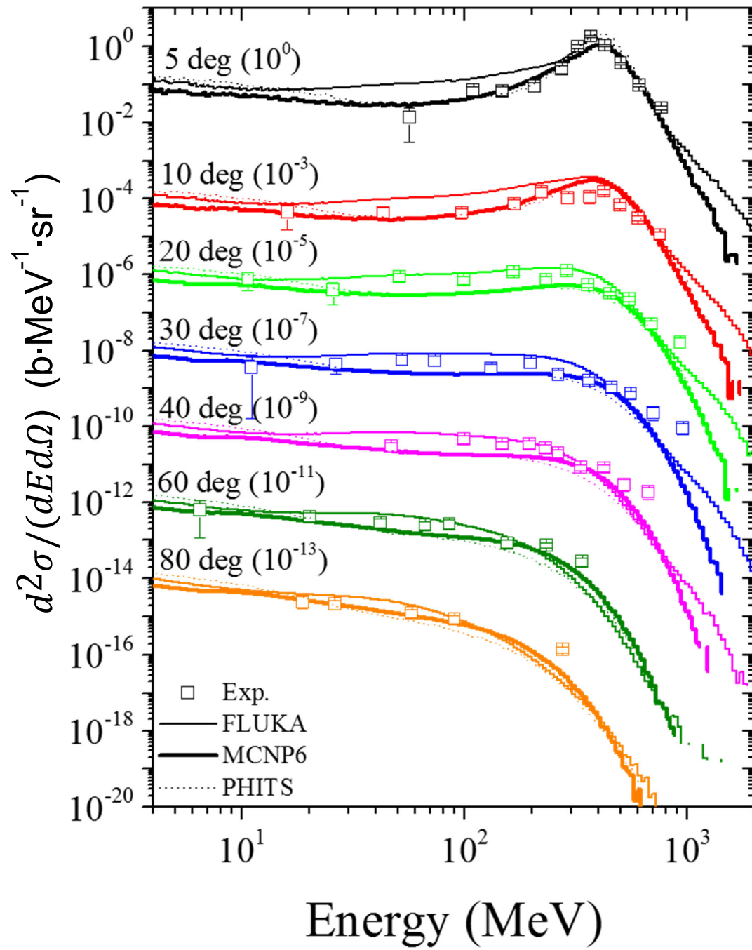
Figure 55. The neutron DDX with 400-MeV/nucleon ^{84}\text{Kr} + ^{\text{nat}}\text{Cu} target.
