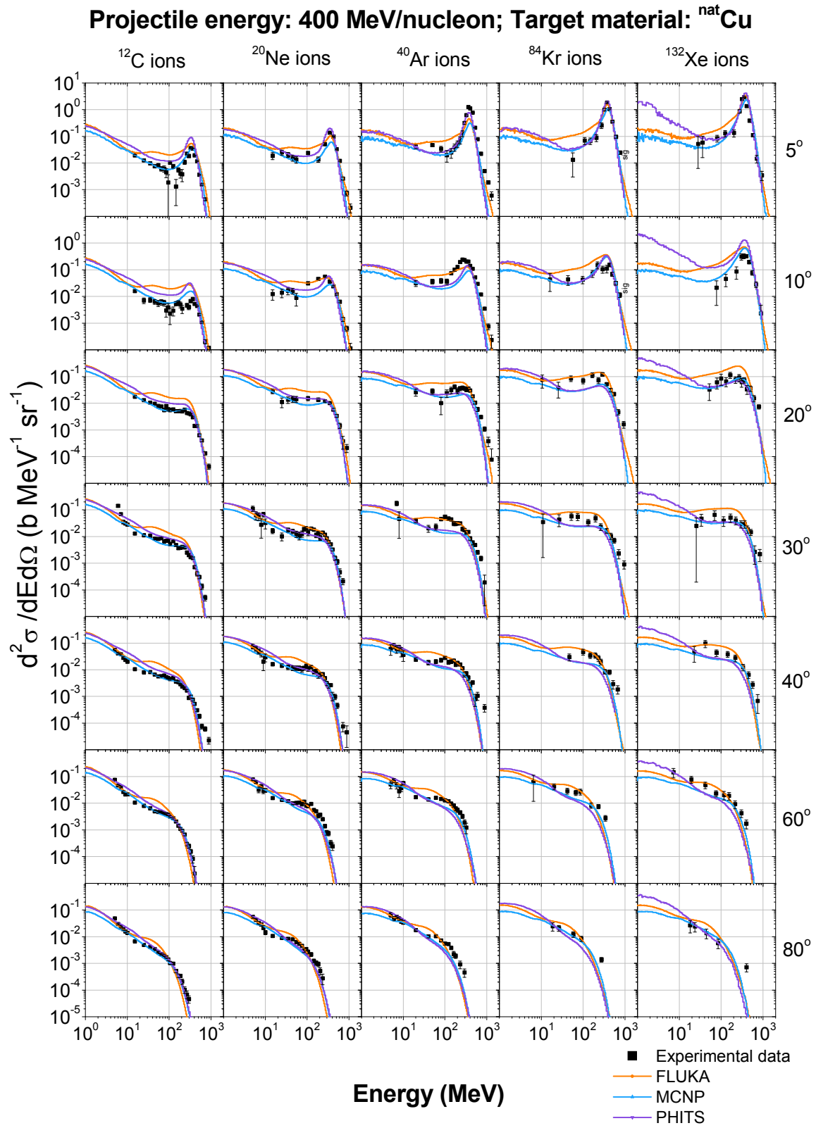
Figure 42. The projectile-mass-dependent DDX with ^{nat}\text{Cu} targets.
