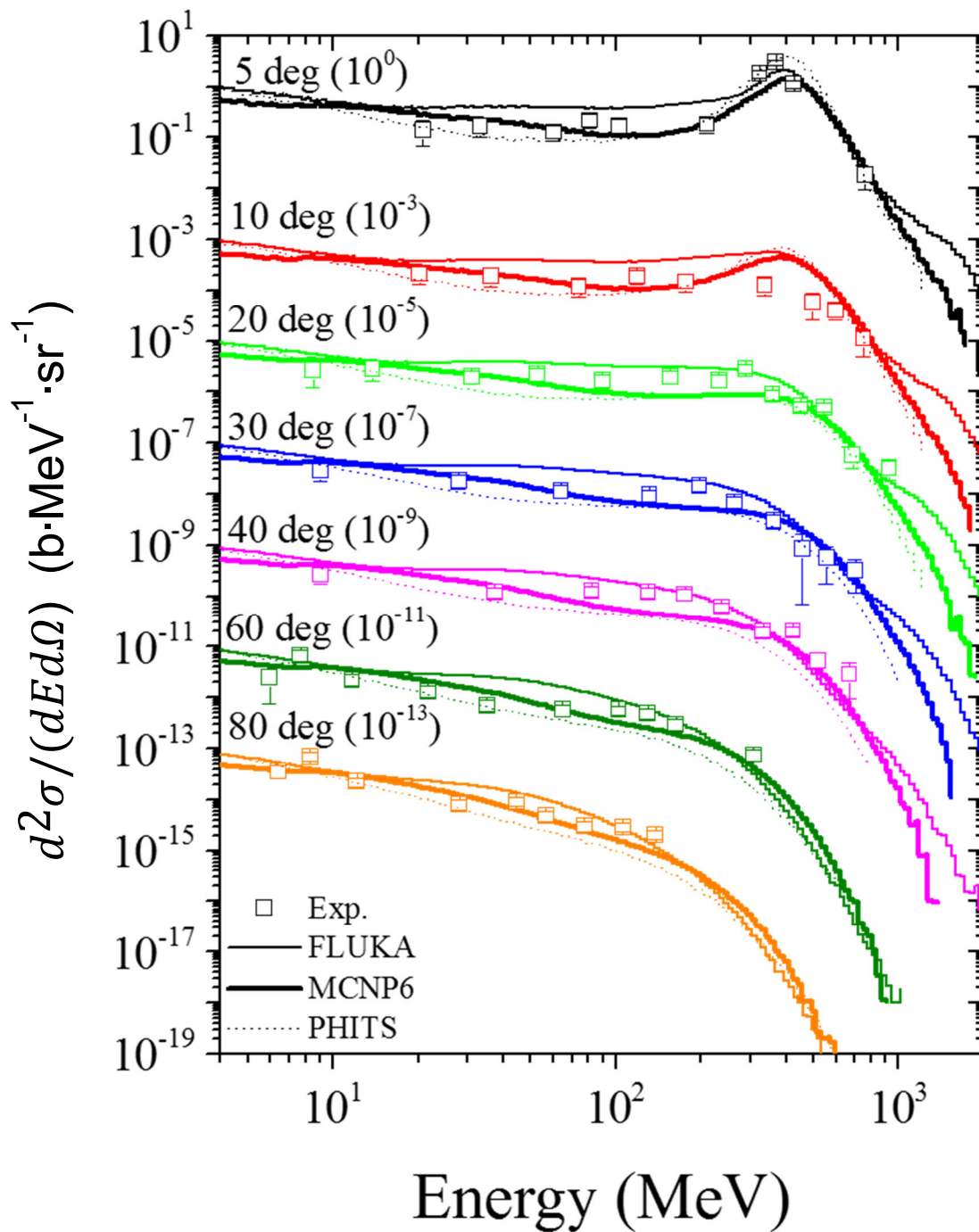
Figure 56. The neutron DDX with 400-MeV/nucleon ^{84}\text{Kr} + ^{\text{nat}}\text{Pb} target.
