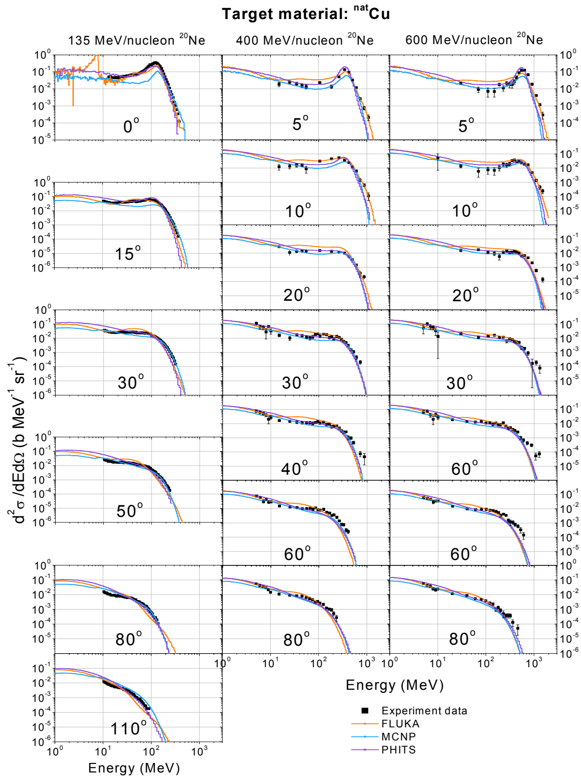
Figure 41. The projectile-energy-dependent DDX with ^{nat}\text{Cu} targets.
