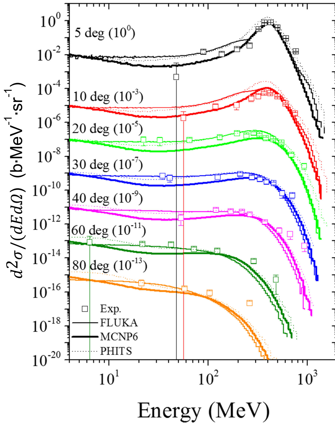
Figure 52. The neutron DDX with 400-MeV/nucleon ^{84}\text{Kr} + {}^{\text{nat}}\text{Li} target.
