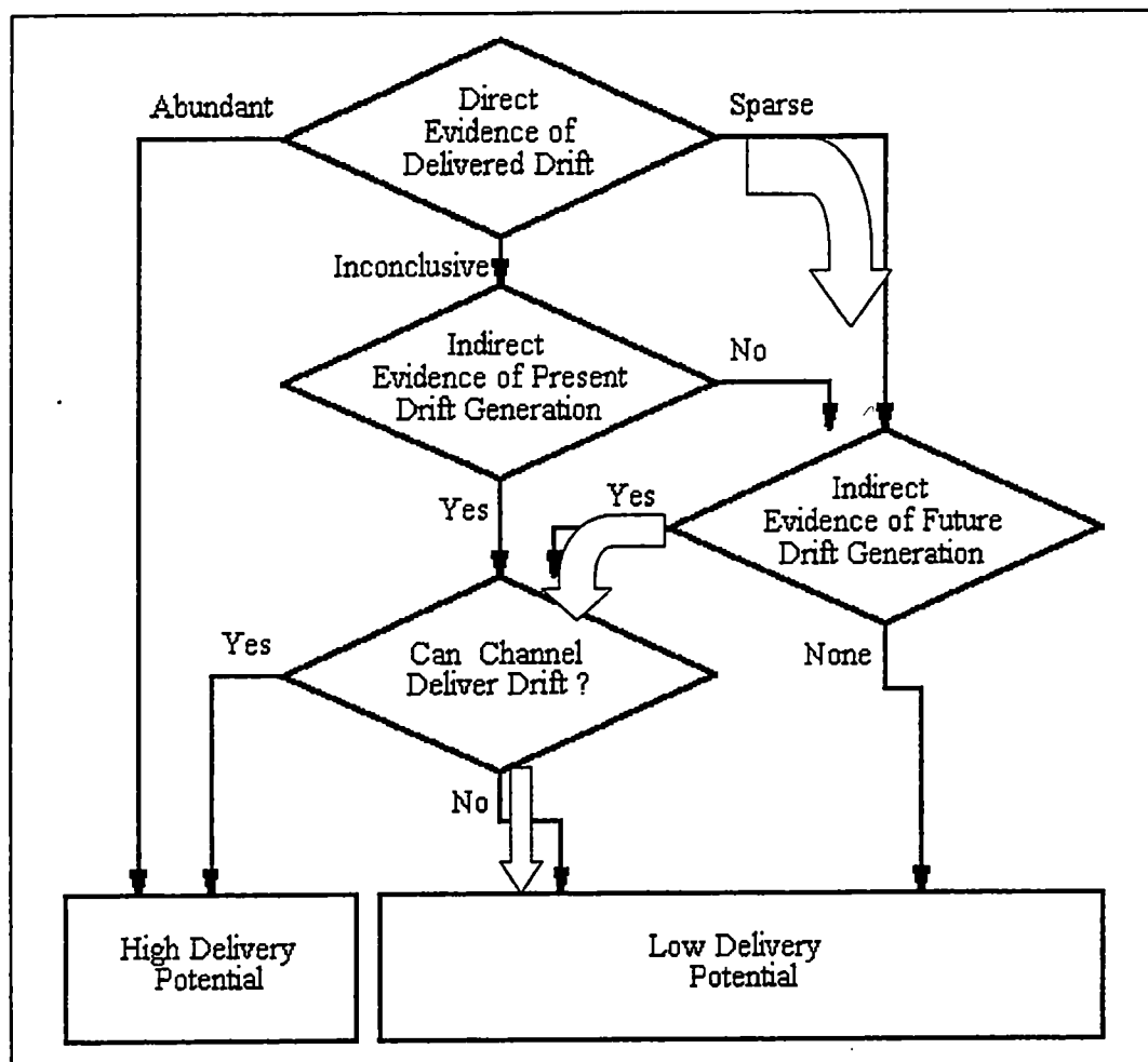
Figure C1 – Flow chart for evaluating potential for drift delivery,(from Diehl, 1997)
