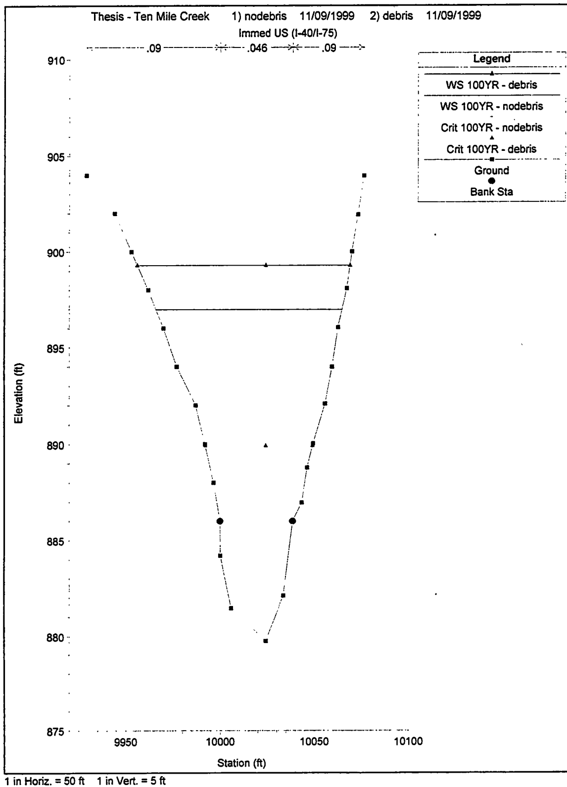
Figure C6 – Immediately Upstream Cross Section from Interstate Highway 40 / 75 Bridge.
