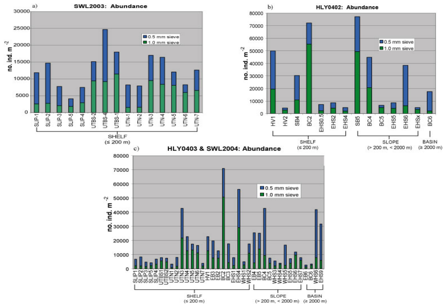
Figure 11. Abundance of fauna collected on the 0.5 mm (blue) and 1.0 mm (green) for each cruise.
