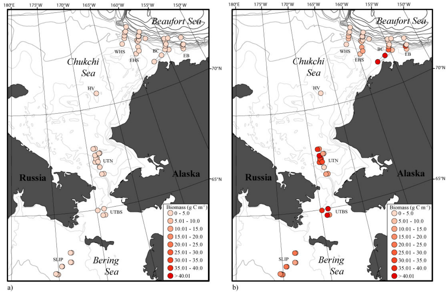
Figure 13. Benthic macrofaunal biomass ( \text{g C m}^{-2} ) retained on a) the 0.5 mm alone and b) the 1.0 mm sieve screen in the study region. Carbon biomass was calculated using wet weight biomass of sampled macrofauna following the methods of Grebmeier (1987) and previously recorded carbon conversion values of Stoker (1978).
