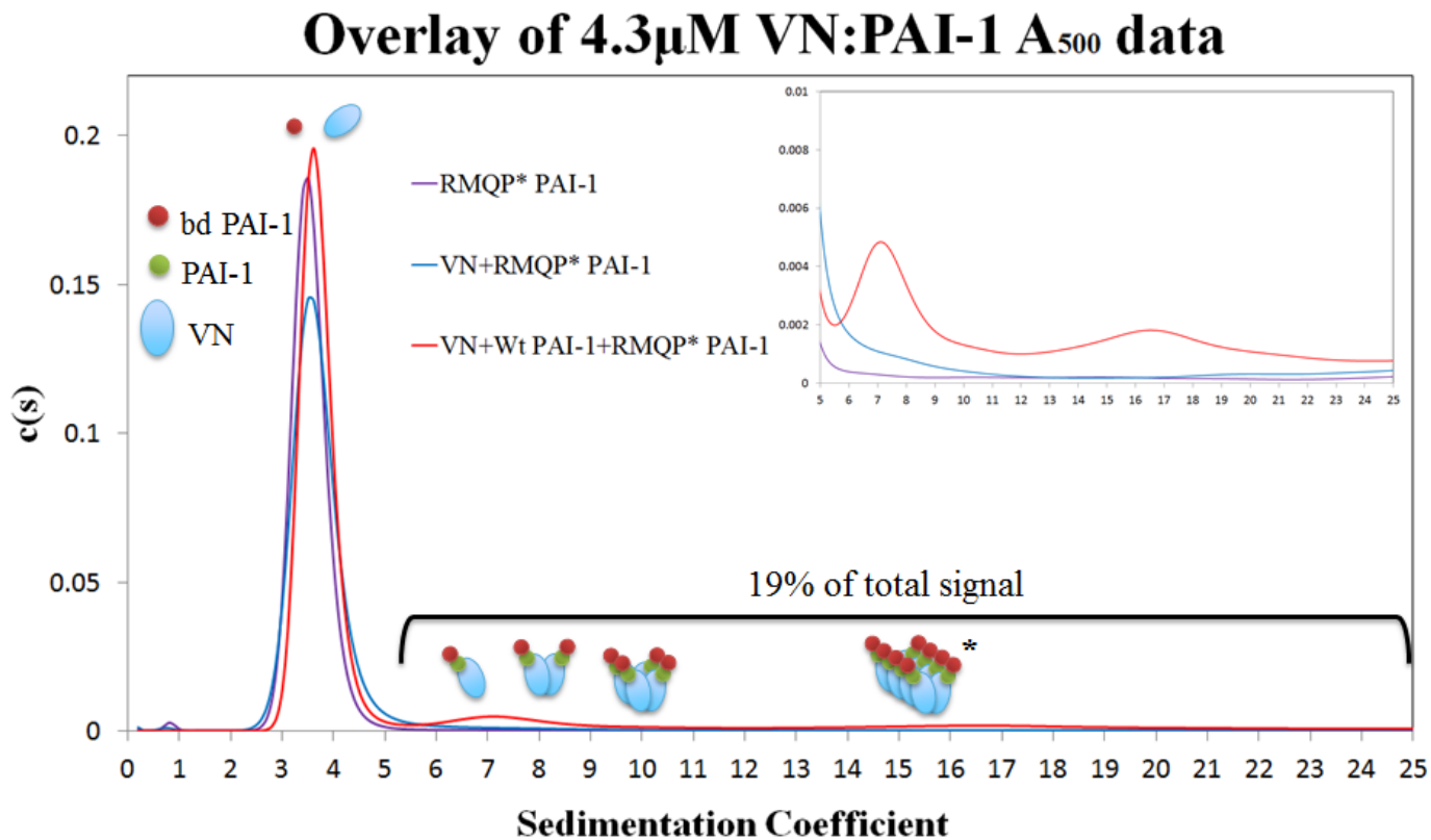
Figure 3.20 4.3 \mu M A 500 AUC Data for RMQP*NBD PAI-1:VN complex formation
