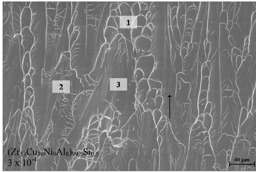
Figure 4-14: (continued) (c) fracture surface.
