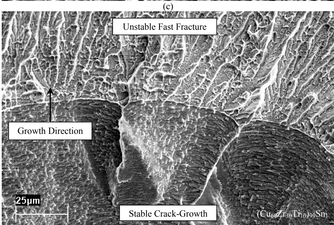
Figure 4-25: (continued) (c) Fatigue striations, (d) Transition from a stable crack-growth to unstable fast fracture.
