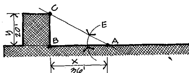
Site Section
