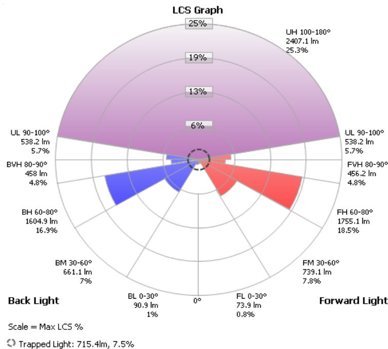
Figure 24. Light distribution curve of figure 23 luminaire (Holophane lighting procure)
