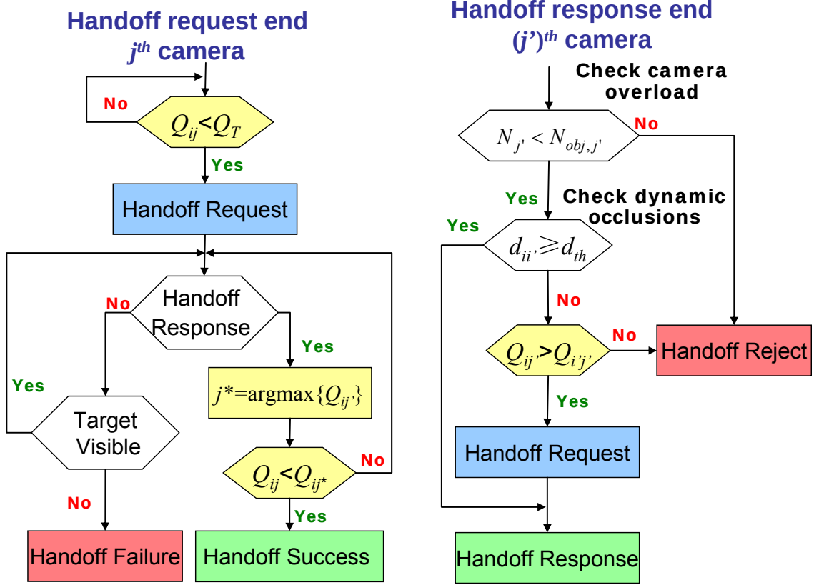
Figure 5.1. Flow chart of the camera handoff algorithm. The handoff response end has the ability to handle dynamic occlusion and camera overload. N_{j'} is the number of tracked objects in the (j')^{th} camera and N_{obj,j'} is the maximum number of objects that can be tracked simultaneously by the (j')^{th} camera. d_{ii'} denotes the distance between the images of the i^{th} and (i')^{th} targets and d_{th} is a predefined threshold for dynamic occlusions.
