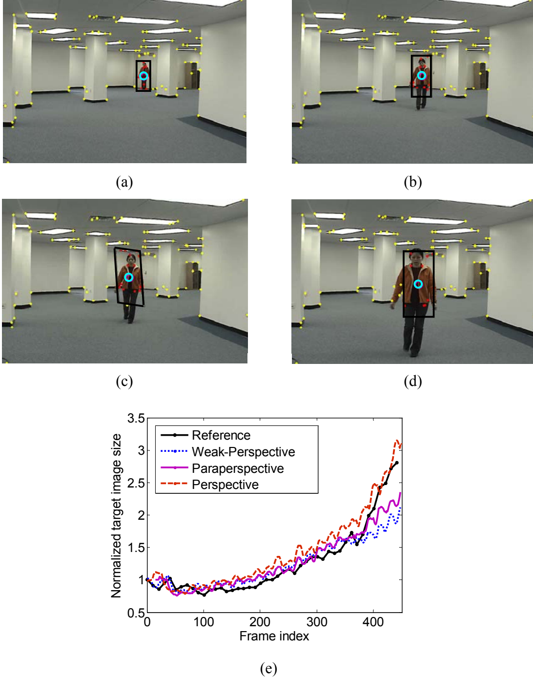
Figure 4.2. (a)-(d) Sample frames from the pedestrian sequence. Yellow and red dots present the detected corners in the background and foreground, respectively. The affine shape separating the foreground and background corners is depicted by a black quadrilateral. A light blue circle shows the gaze point, to which the camera is directed. (e) Comparison of measured and estimated target scale (normalized to the target's image size in the first frame).
