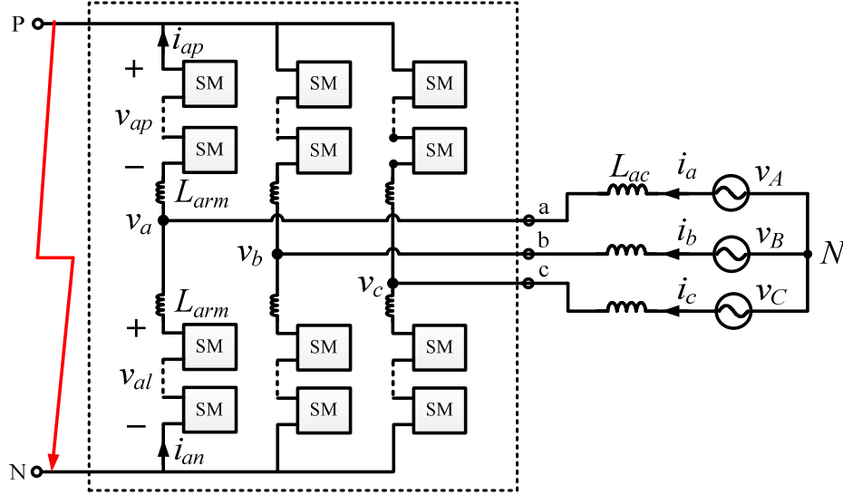
Figure 3-3. Pole to pole fault for a grid connected MMC
