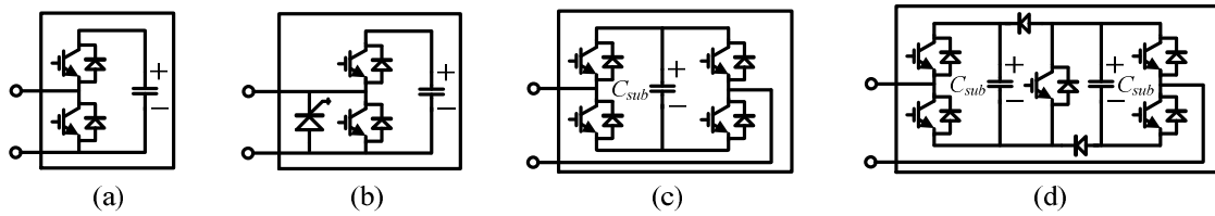
Figure 2-2. Different sub-module topologies: (a) half-bridge circuit, (b) half-bridge circuit with bypass thyristor, (c) full-bridge circuit, and (d) clamped double half-bridge circuit
