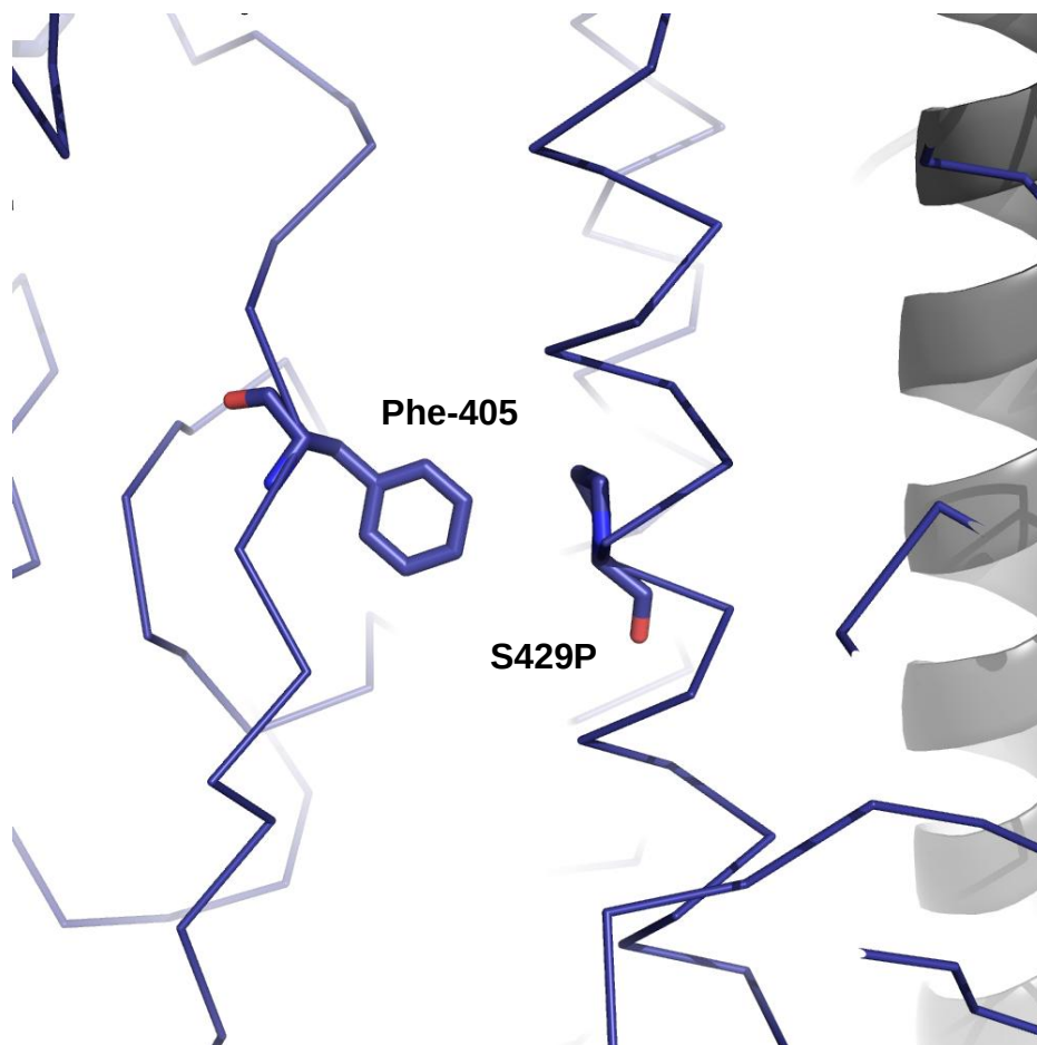
Figure 2.12 Stabilization of B-loop by S429P mutation. The addition of an aliphatic ring by the mutation of Ser-429 to proline allows the aromatic residue of Phe-405 of the B-loop to be stabilized in a ring packing manner. The S429P mutation was modeled in using Swiss pdbViewer and the lower scoring trans oriented side chain was chosen.
