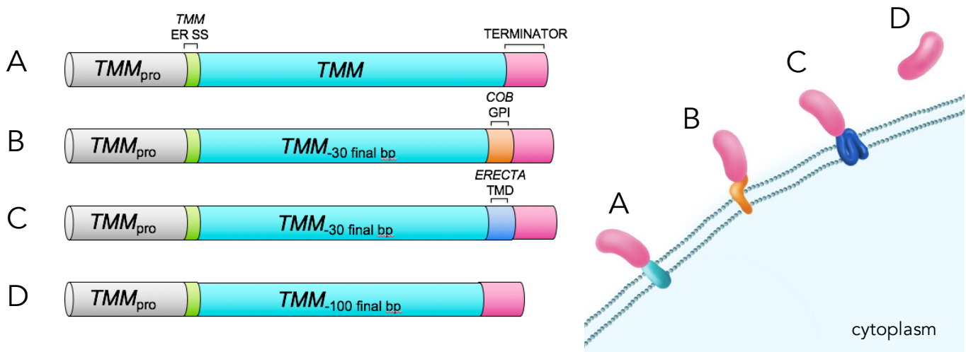
Figure 6: Map of the TMM DNA reinsertions created and theoretical image of the TMM reinsertions if localized to the plasma membrane. A) Endogenous TMM, B) TMM+GPI-Ancor, C) TMM+TMD, D) Extracellular TMM.
