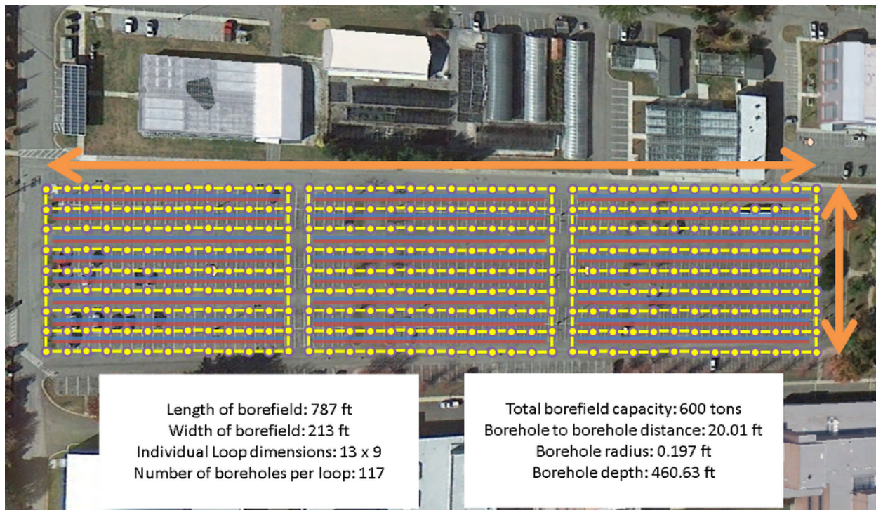
Figure 4.3: Borefield Layout
