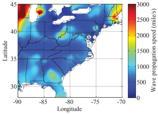
Figure 4.6. Electromechanical wave propagation speed distribution in the 25% PV penetration scenario
