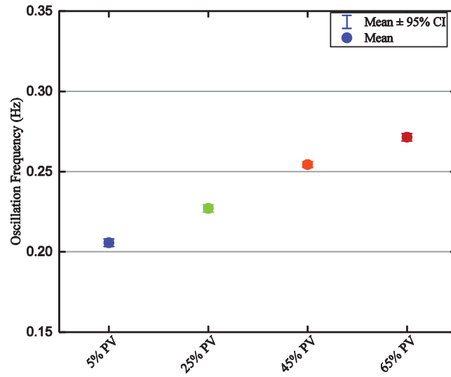
Figure 3.4 Oscillation frequency change as PV penetration increases
