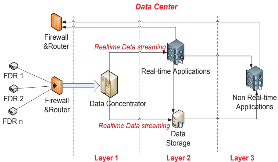
Figure 7.4. The FNET/GridEye data center structure
