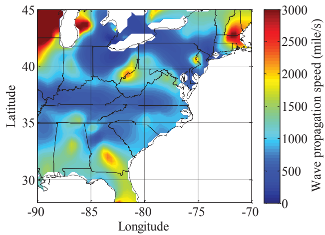
Figure 4.7. Electromechanical wave propagation speed distribution in the 45% PV penetration scenario
