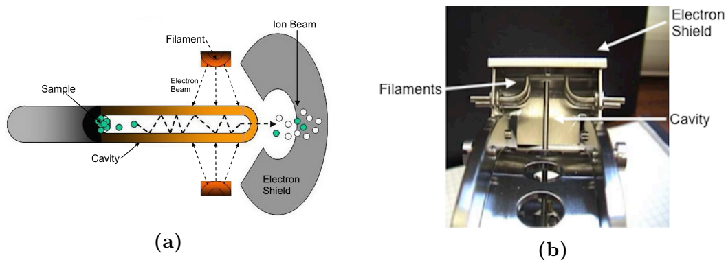
Figure 2.8: (a) An illustration of an HECS, the cavity is heated via electron bombardment; electrons are generated from resistively heated standard rhenium filament ribbons. (b) Photograph of an HECS mounted on a standard sample turret. Figures were adapted from reference [34].
