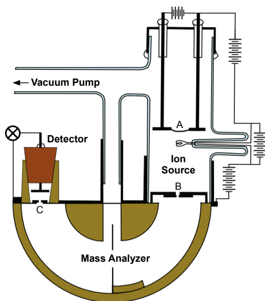
Figure 2.1: An illustration of the first thermal ionization mass spectrograph developed by A. J. Dempster, adapted from Dempster [31]. Components of Dempster’s mass spectrograph relevant to contemporary TIMS are: The platinum filament upon which the sample was loaded is labeled (A), the entrance and exit slits are labeled (B) and (C), respectively.
