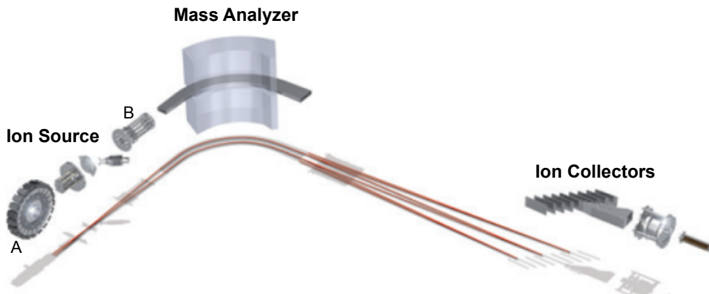
Figure 2.2: An exploded view illustration of a modern TIMS instrument. Much like Dempster’s design, contemporary TIMS instruments are composed of three main components: the ion source, mass analyzer, and the ion collector(s). The sample turret is labeled (A) and the ion optic lenses are labeled (B) are contained in the source housing. This figure was adapted from Thermo Fisher Scientific [36]
