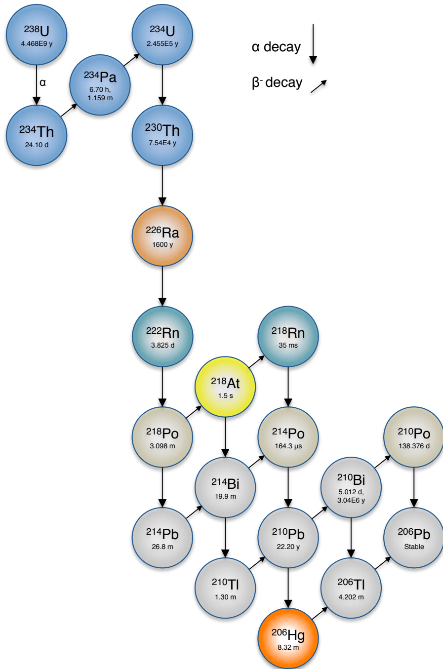
Figure 5.1: The 4n + 2 decay series with half-life and decay mode mode information. After uranium purification, ^{230}\text{Th} slowly grows in and can be used to determine time elapsed since purification.
