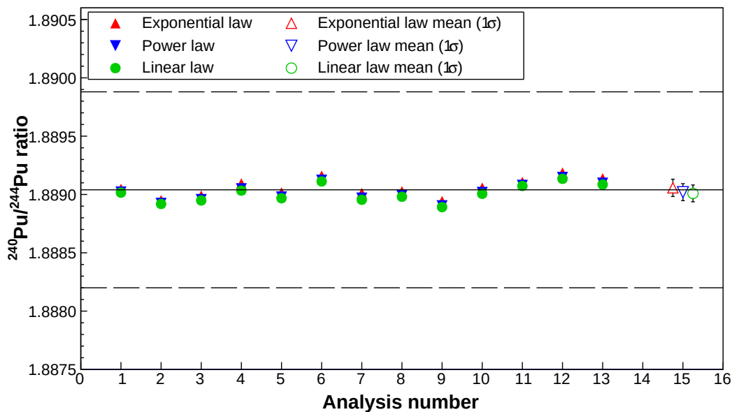
Figure 4.2: High precision data, obtained using PIE sources, corrected for mass bias. The solid line represents the certified isotope ratio; uncertainty in the certified ratio is shown by the dashed line.
