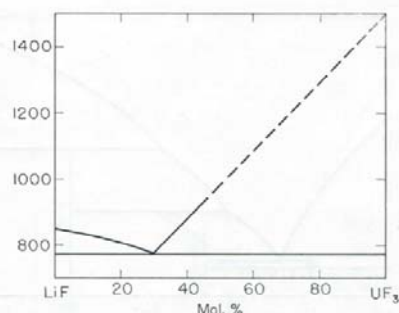
FIG. 1476.—System LiF-UF 3 ; tentative.
