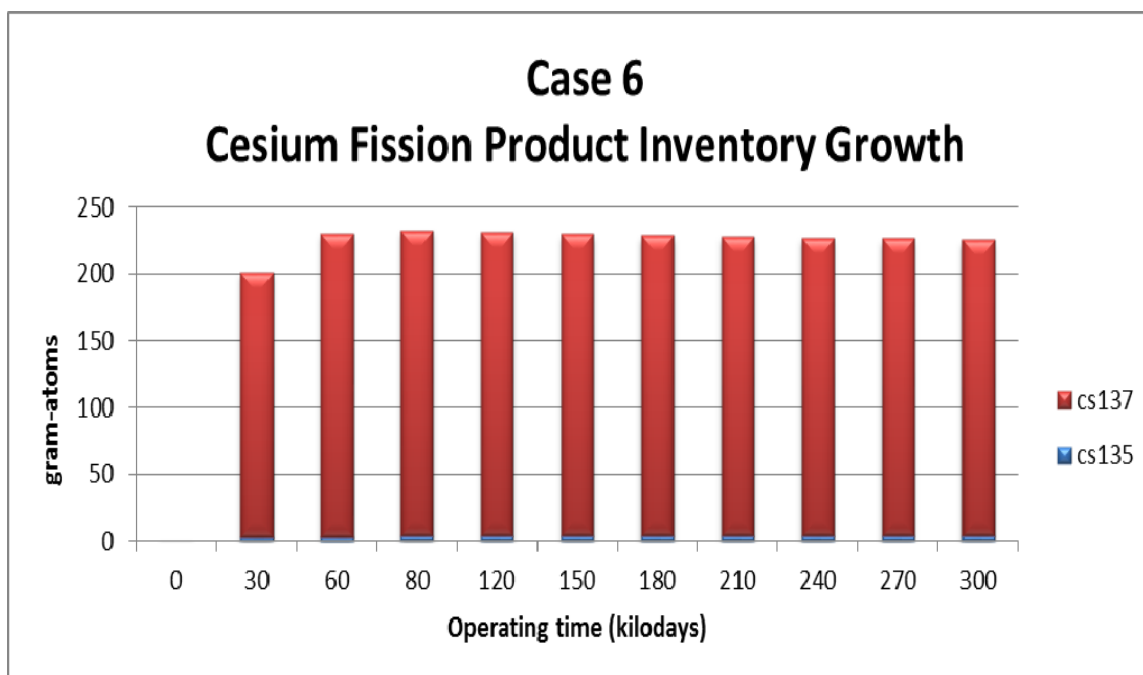
Figure 49 Case 6 Cesium Inventory
