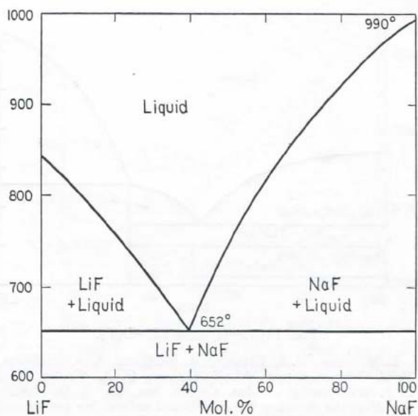
FIG. 1467.—System LiF-NaF.
