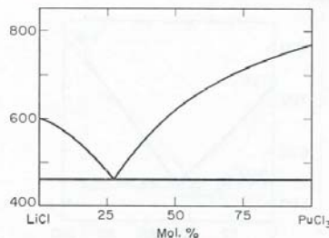
FIG. 1296.—System LiCl-PuCl 3 .
