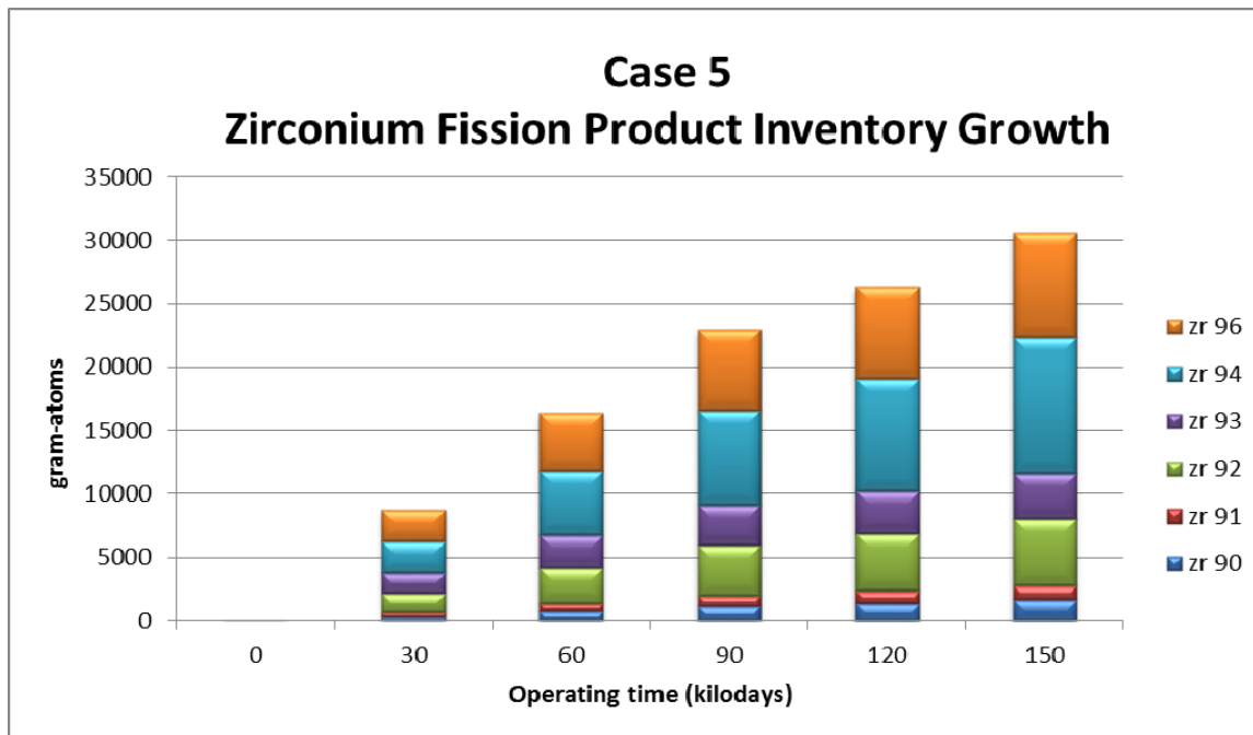
Figure 38 Case 5 Zirconium Fission Product Inventory
