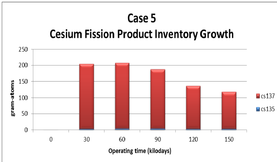
Figure 42 Case 5 Cesium Inventory
