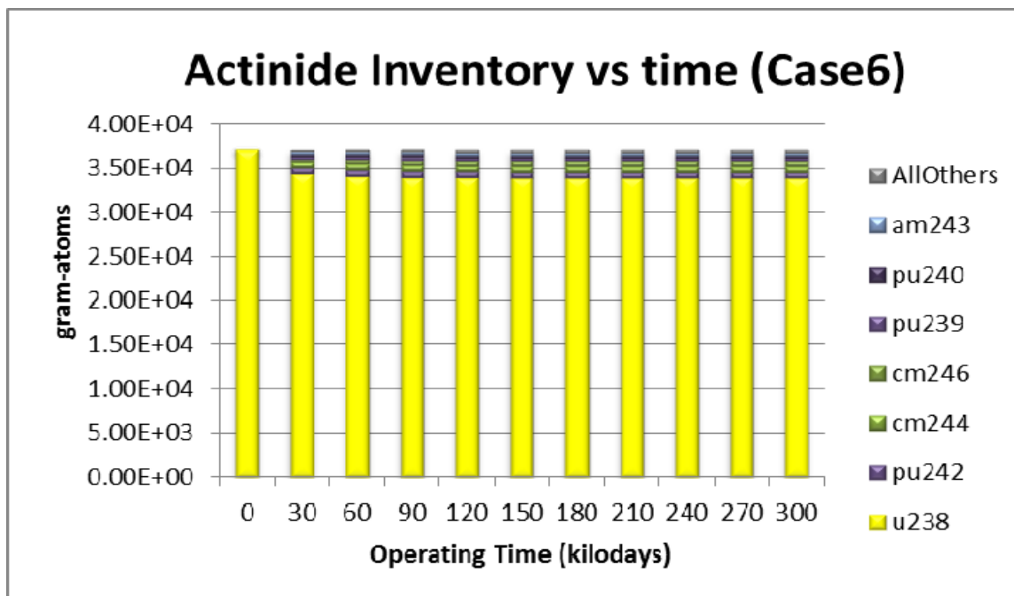
Figure 46 Case 6 Most Abundant Actinides vs. operating time
