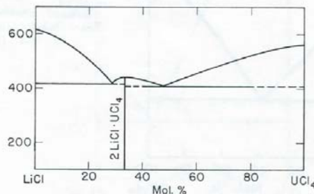
FIG. 1298.—System LiCl-UCl 4 ; tentative.
