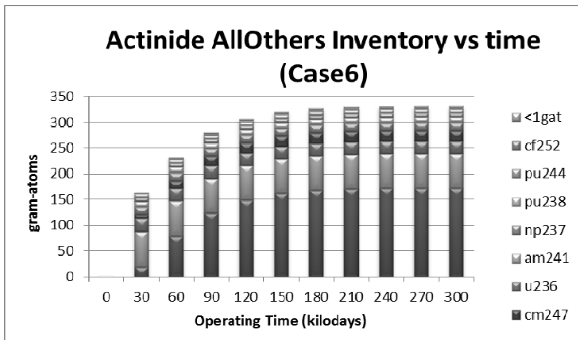
Figure 48 Case 6 Additional Actinides Sorted by Abundance
