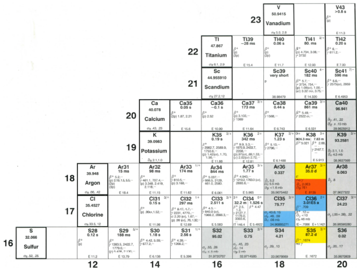
Figure 7 Chlorine Isotopes in Chart of Nuclides p 22
