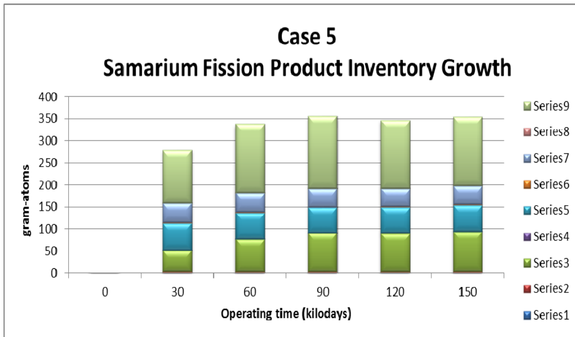
Figure 40 Case 5 Samarium Inventory
