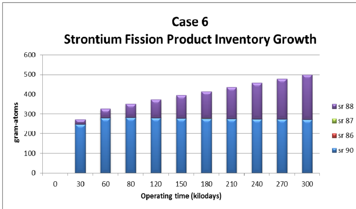
Figure 50 Case 6 Strontium Inventory
