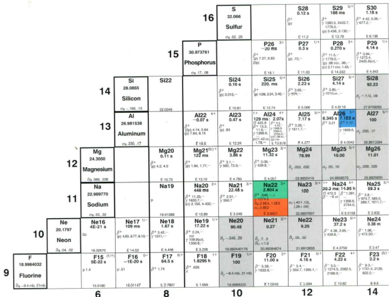
Figure 8 Fluorine and higher Isotopes in Chart of Nuclides p 20
