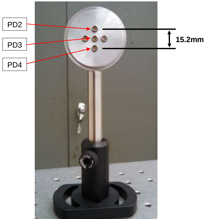
Figure 2.13: Photodiode array.
