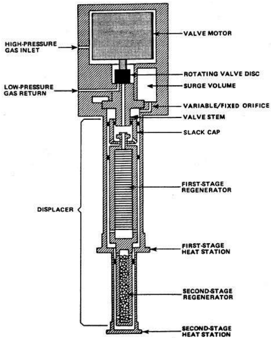
Figure 2.8: Simplified cold head diagram [20].
