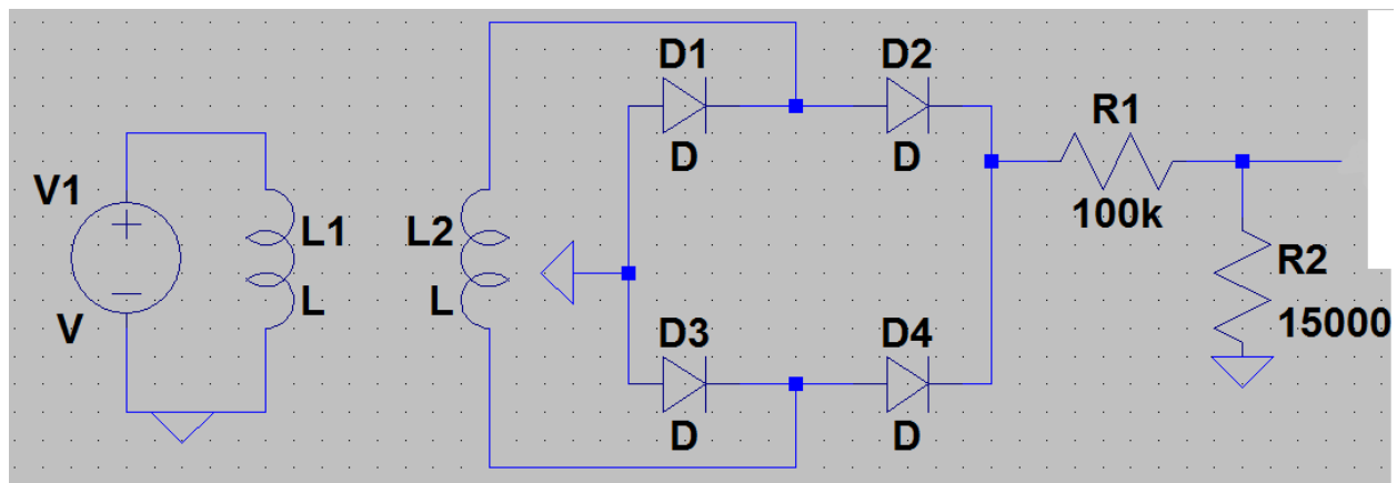
Figure 3. Voltage divider circuit
