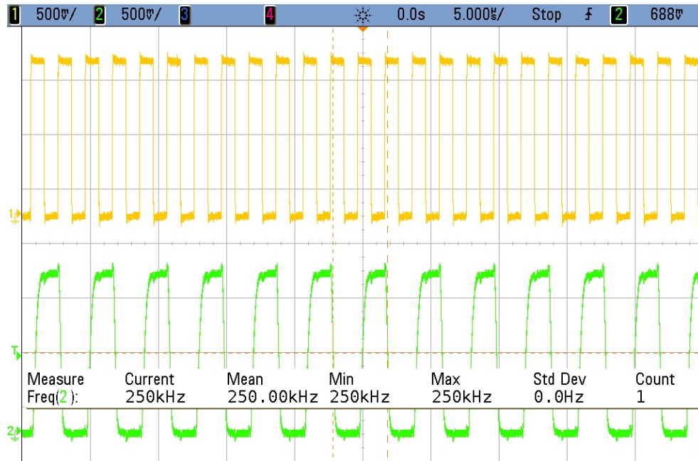
Figure 4.6: Experimental output frequency for I_S = 100 nA, I_B = 400 nA, and f_{CLK} = 500 kHz.
