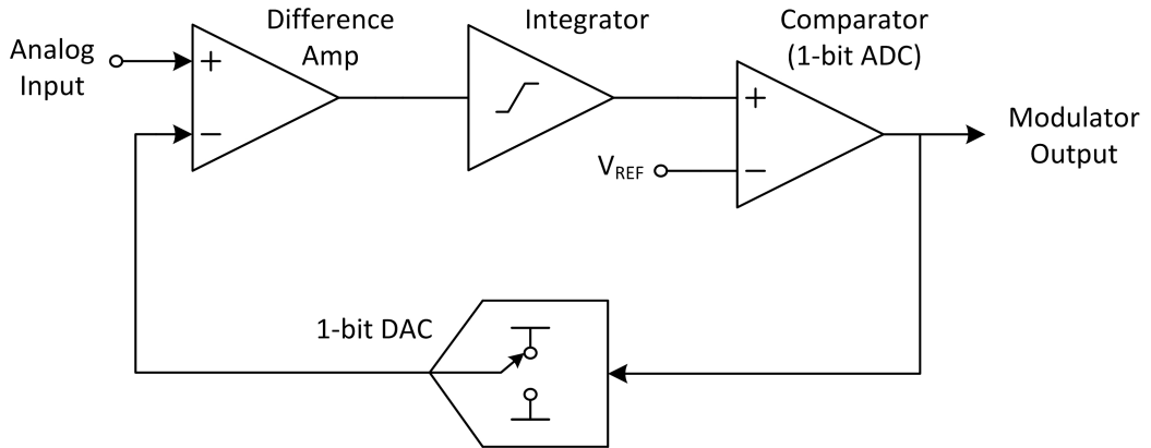
Figure 2.3: Block diagram of a first-order delta-sigma modulator.
