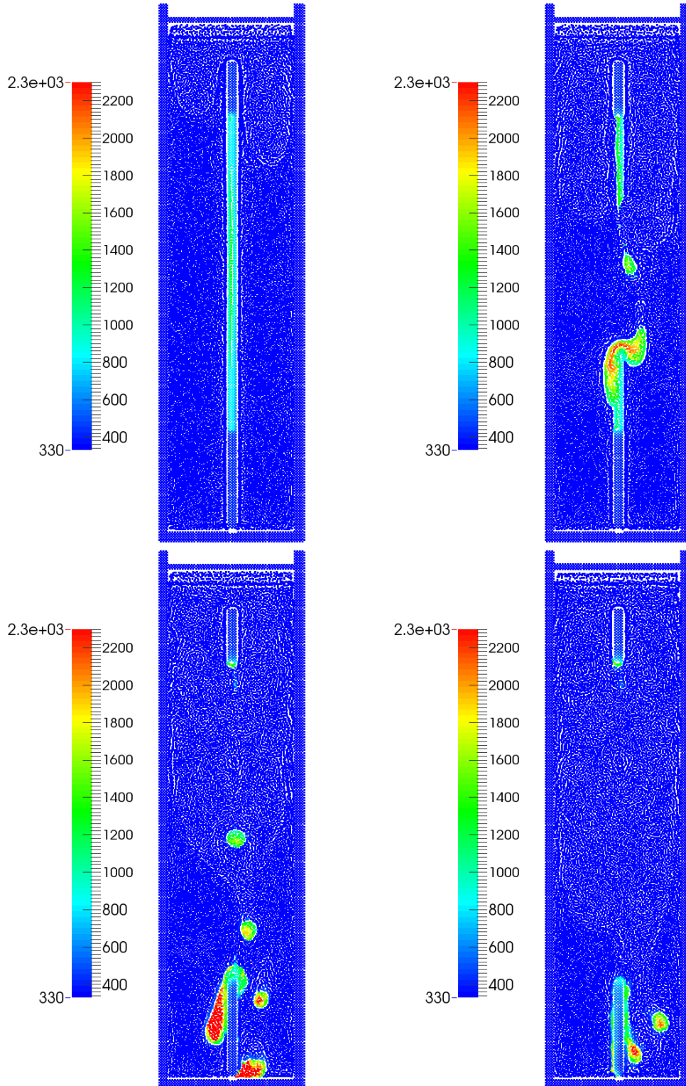
Figure 5.10: Case 4 temperature [K].
