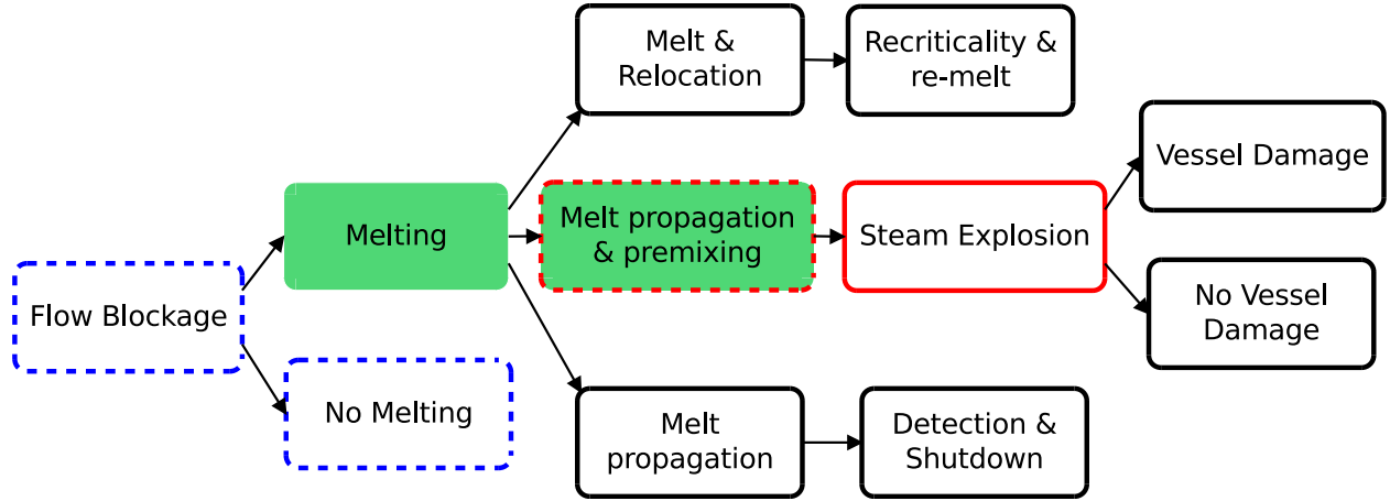
Figure 1.7: Event sequence following flow blockage [19].
