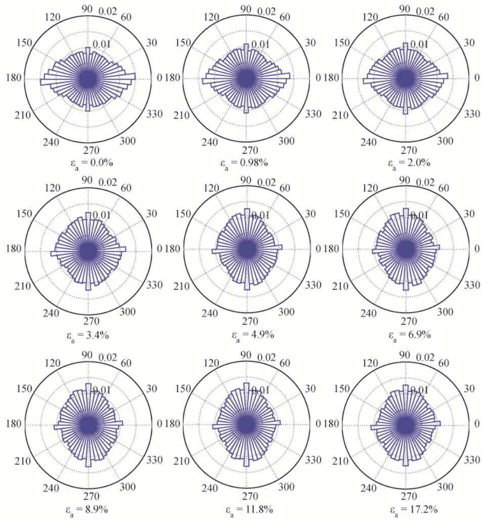
Figure 6.2. Global contact normal distribution rose diagrams for full evolution of F35-400kPa experiment
