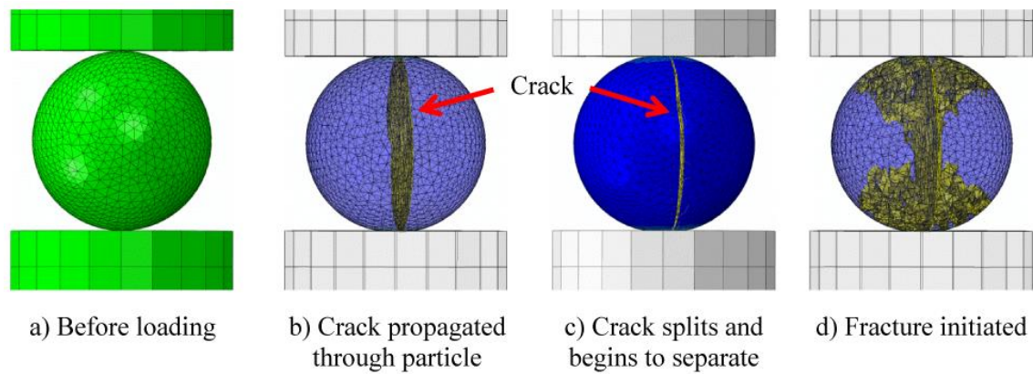
Figure 3.8. Visualization of ideal spherical particle loading and fracture mode
