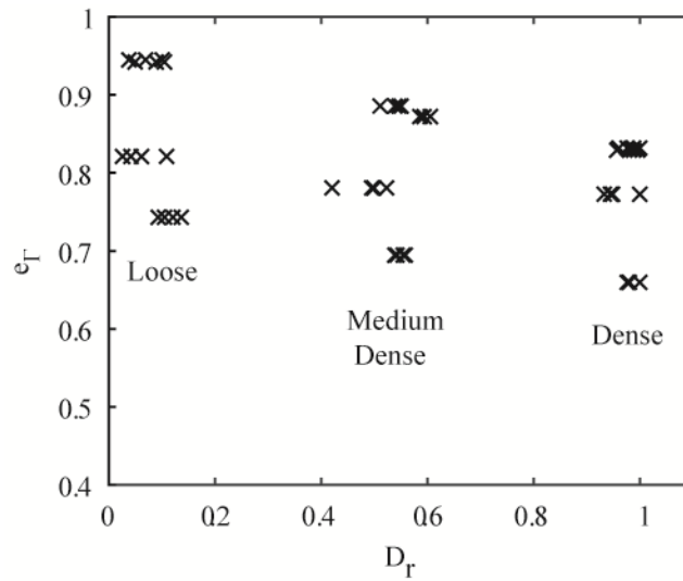
Figure 7.6. Experimental results of e_r versus D_r of four granular materials, demonstrating the effect of density and other variables on e_r
