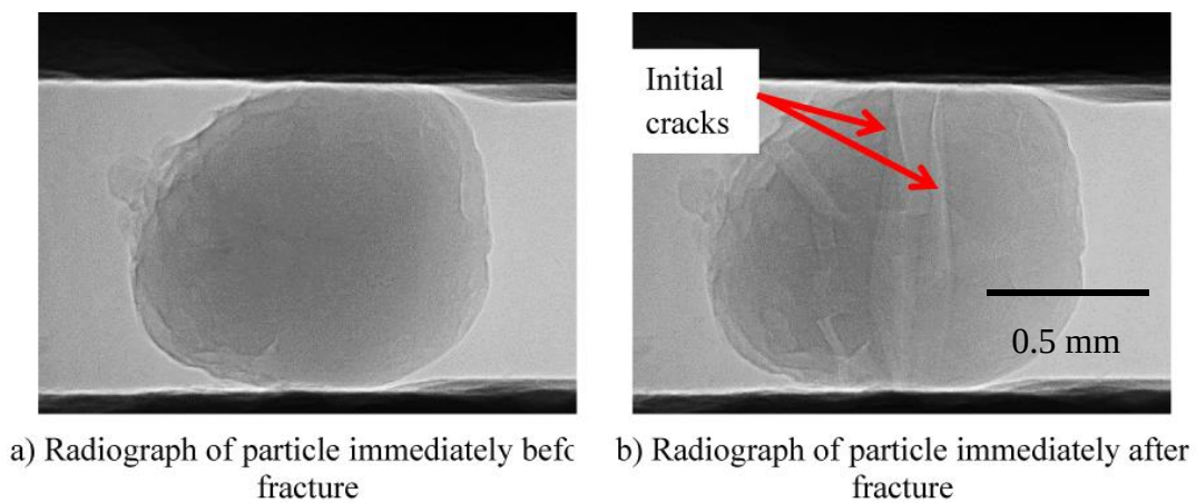
Figure 3.9. Radiograph visualization of first fracture within Particle 1
