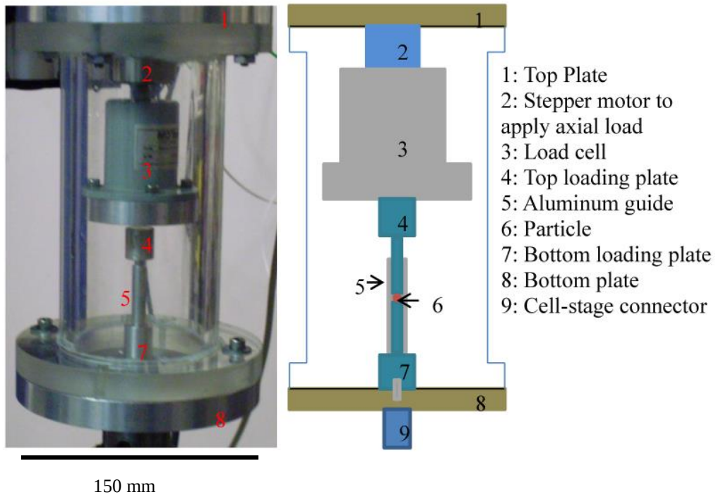
Figure 3.1. Experimental 1D unconfined compression test setup for a single sand particle
