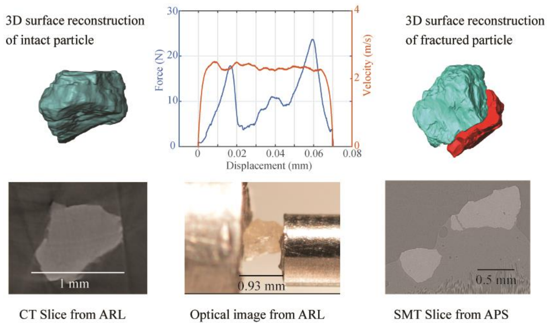
Figure 4.6. Example of experimental results from mini-Kolsky bar testing and particle imaging at Army Research Lab (ARL) and Advanced Photon Source (APS)
