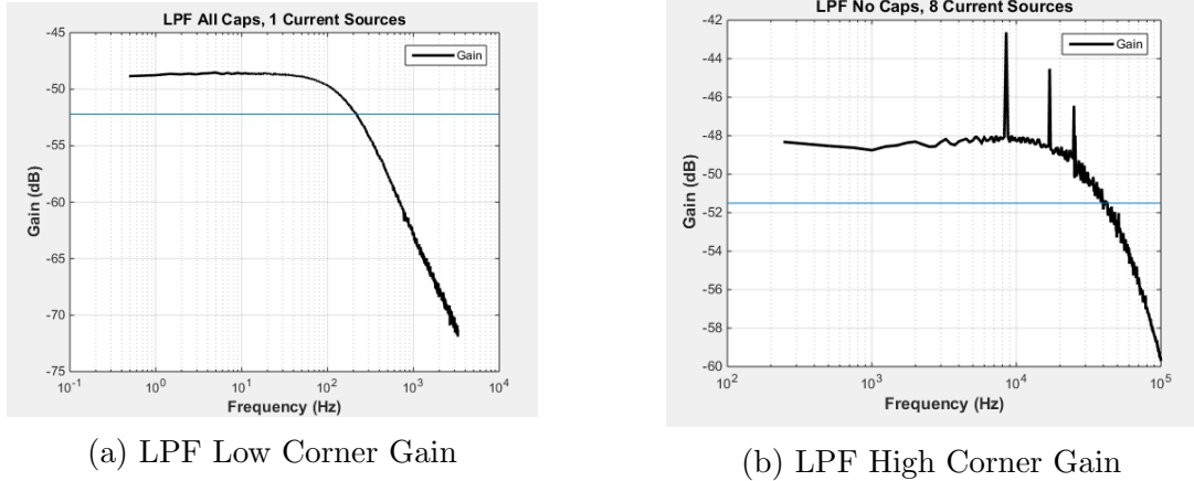
Figure 4.3: LPF Gain Results
