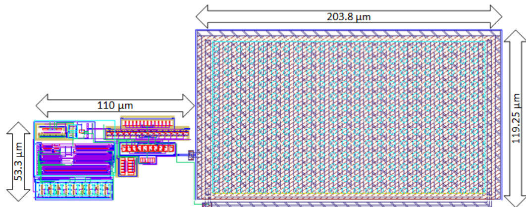
Figure 3.16: Integrator Layout
