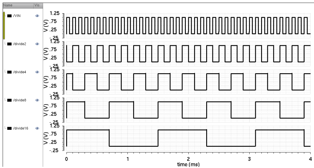
Figure 3.39: Frequency Divider Simulation
