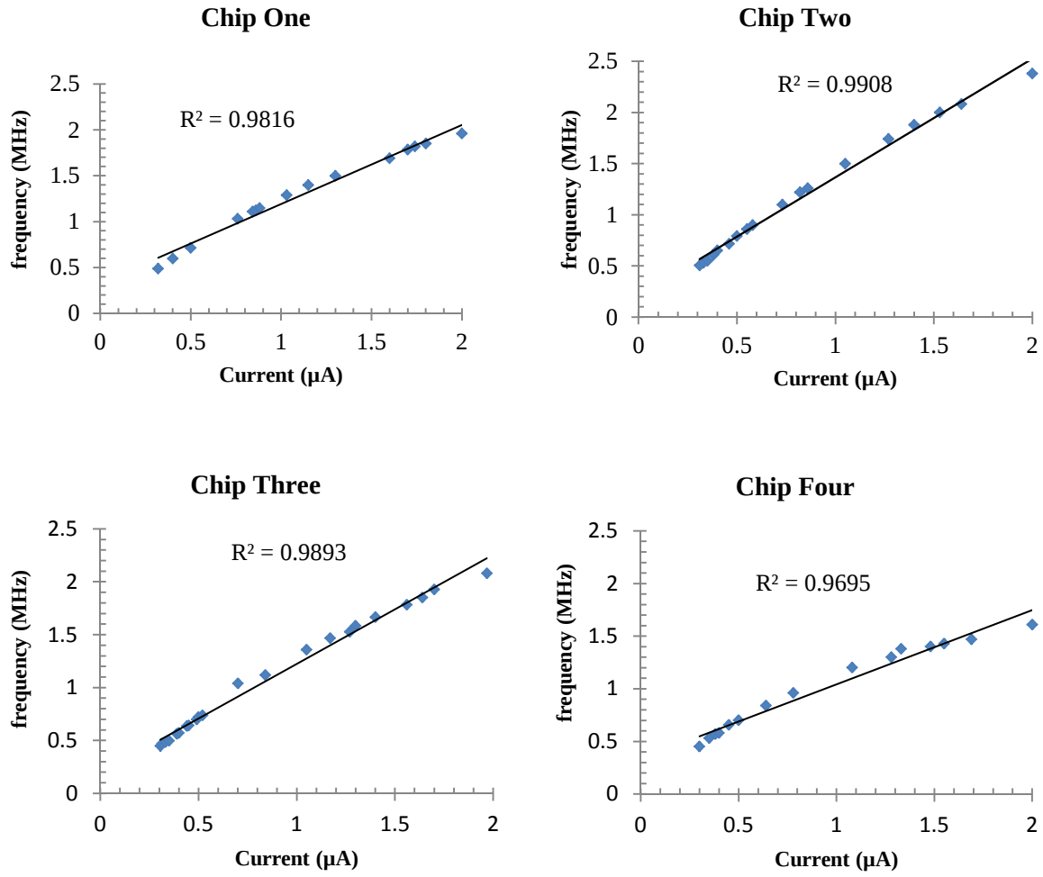
Fig. 6. 11. Chip output frequency result for different values of the sensor current for four different chips.
