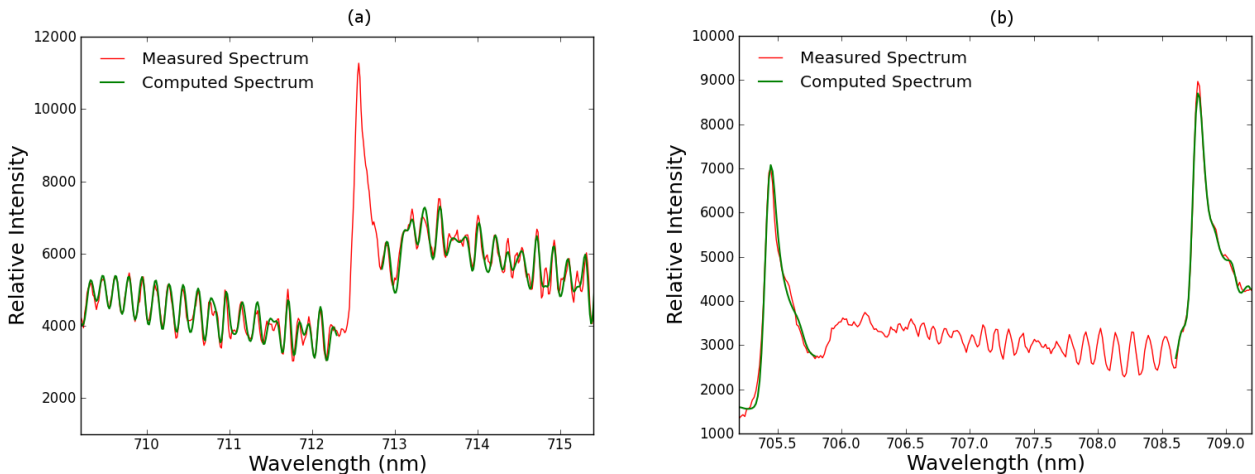
Figure 4.7: TiO A^3\Phi \rightarrow X^3\Delta transition collected at a delay time t_{delay} = 95 \mu s with a 2 \mu s slit width. (a) The fit of the rotational structure results in an inferred temperature of 3216 K. (b) The fit of the vibrational structure results in an inferred temperature of 4178 K (167).
