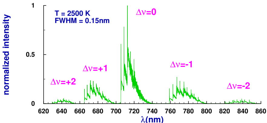
Figure 5.2: Overview of computed spectrum of TiO \gamma bands.
