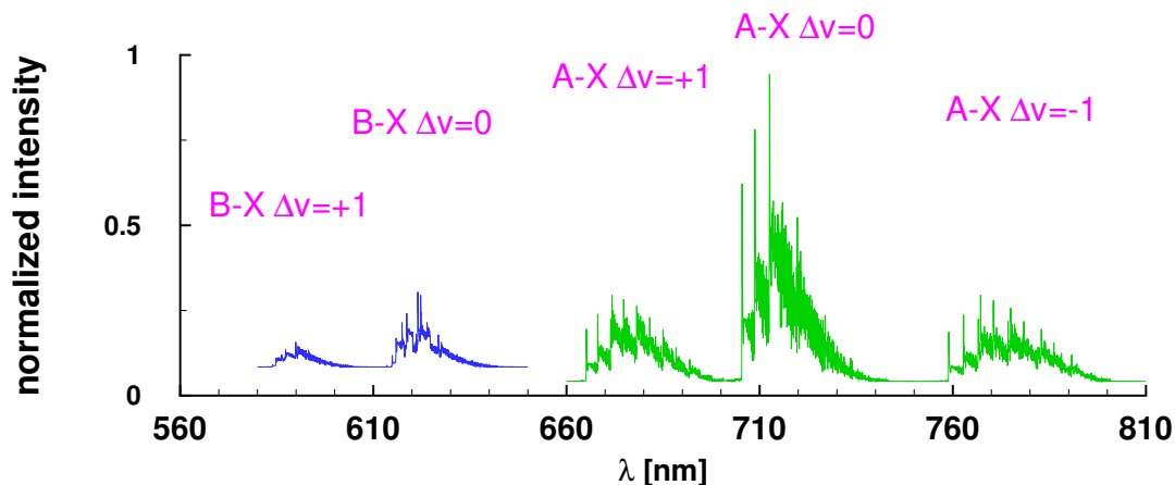
Figure 4.1: Computed B-X and A-X spectra using a \text{FWHM} = 0.08 nm. Inferred temperatures from spectral region containing B-X and A-X are, respectively, 3,800 and 3,030 K (112).
