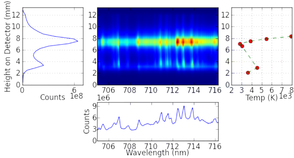
Figure 4.15: The above image represents spectra of laser ablation plasma above a titanium surface recorded at t_{delay} = 20 \mu s with a 2 \mu s gate width.
