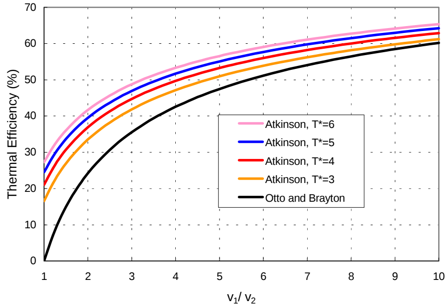
Figure 3. Comparison of the Atkinson, Otto and Brayton cycles' thermal efficiency
