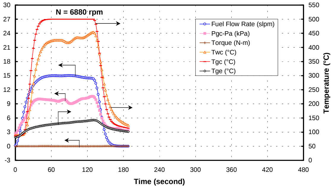
Figure 30. Case B, N = 6880 , three turns in from original gap setting
