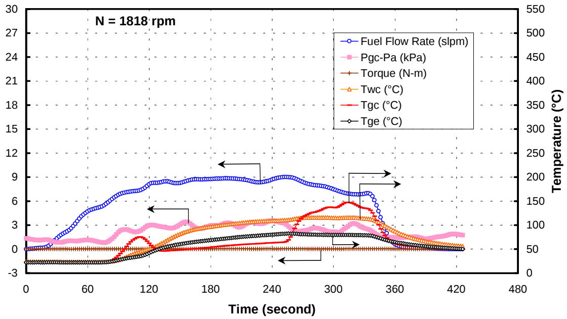
Figure 12. Case A, N = 1818 , zero turns in from original gap setting
