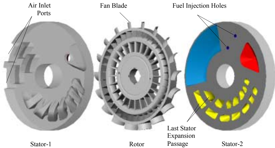
Figure 6. Schematic of three major components of the TurbX™ engine, a view showing details of Stator-2
