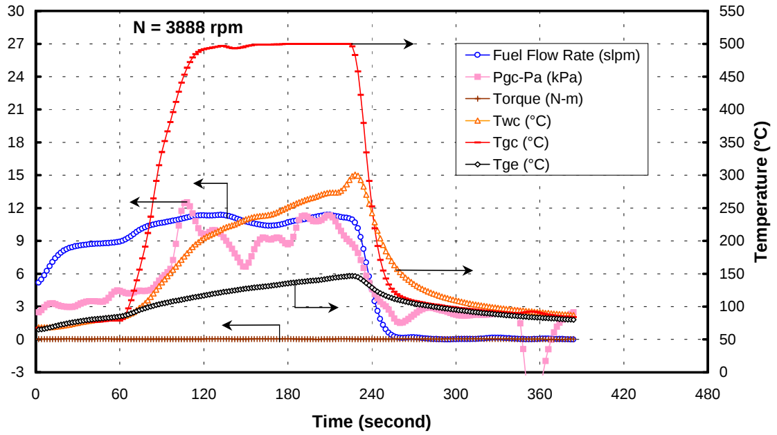
Figure 14. Case A, N = 3888 , three turns in from original gap setting
