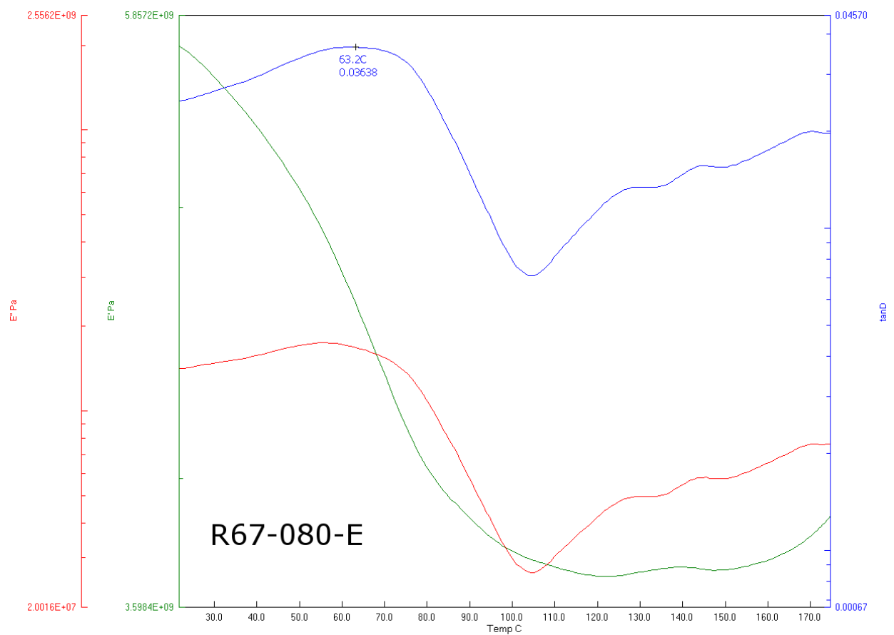
Figure 81: DMA output for R67-080-E
