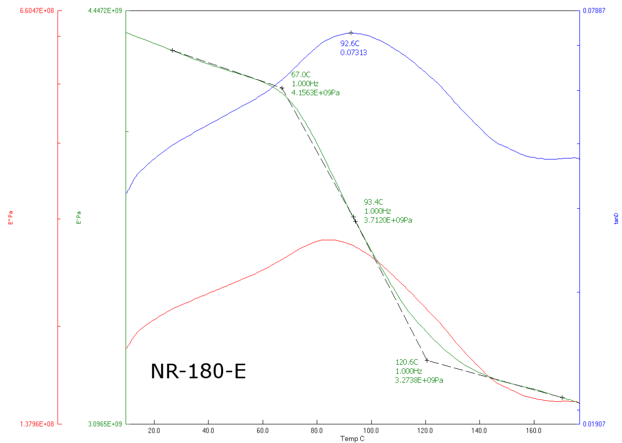
Figure 33: DMA output for NR-180-E
