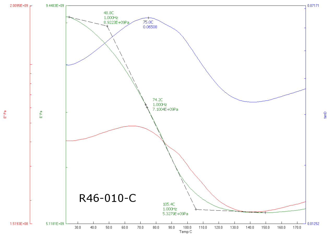
Figure 56: DMA output for R46-010-C
