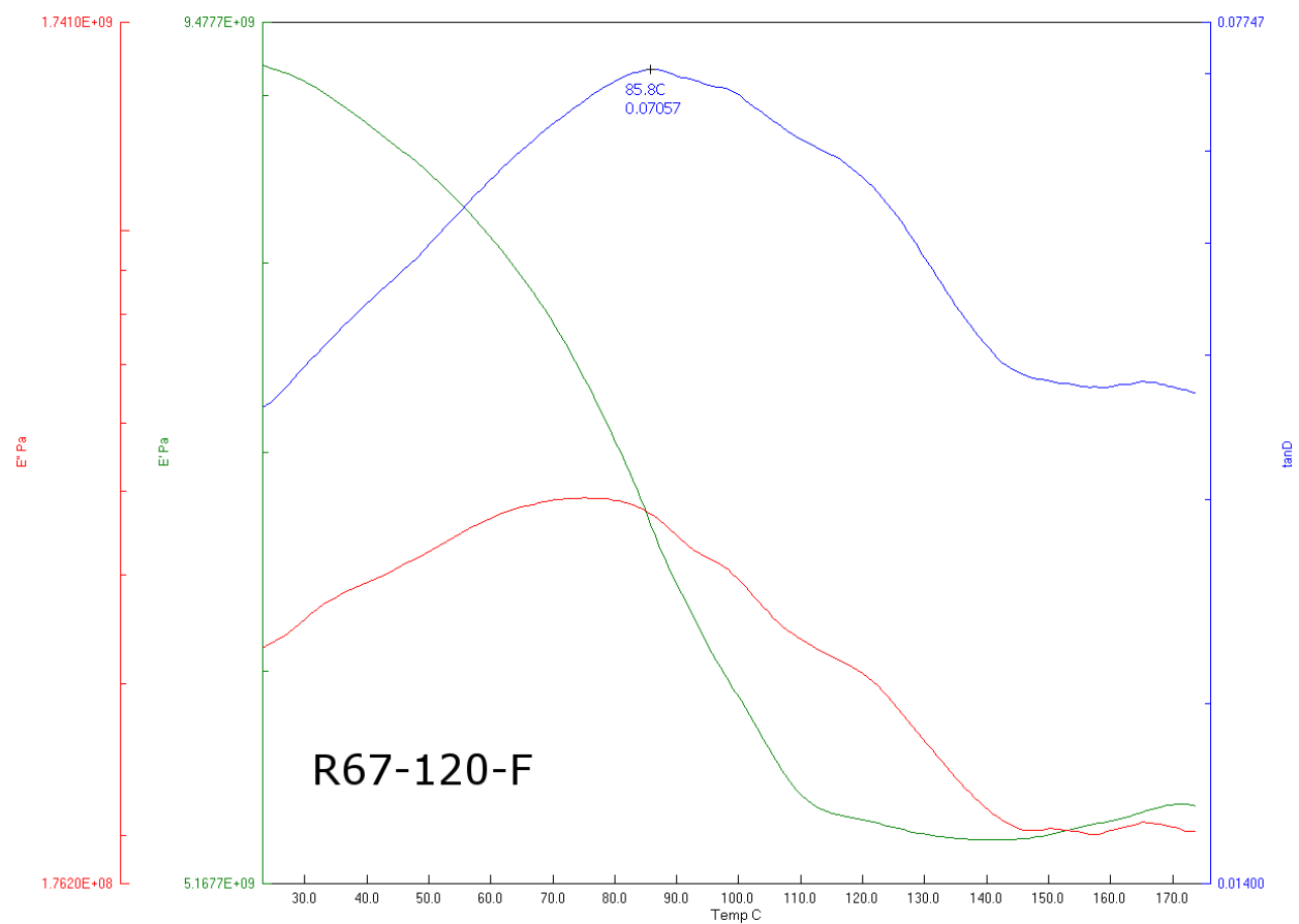
Figure 83: DMA output for R67-120-F
