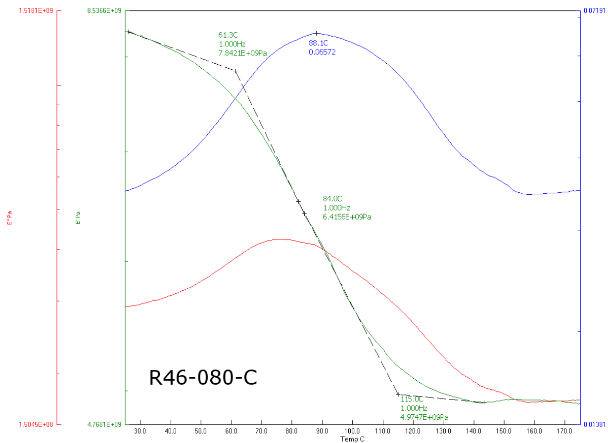
Figure 63: DMA output for R46-080-C
