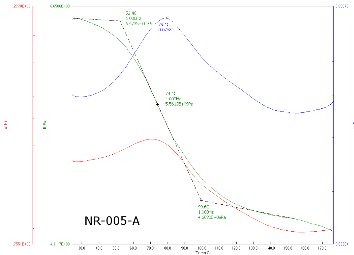
Figure 19: DMA output for NR-005-A
