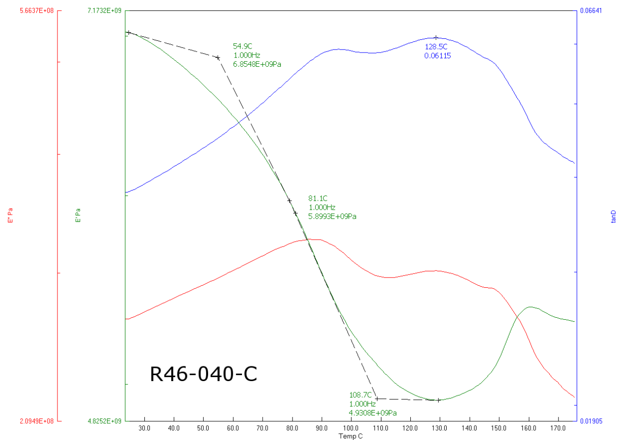
Figure 61: DMA output for R46-040-C
