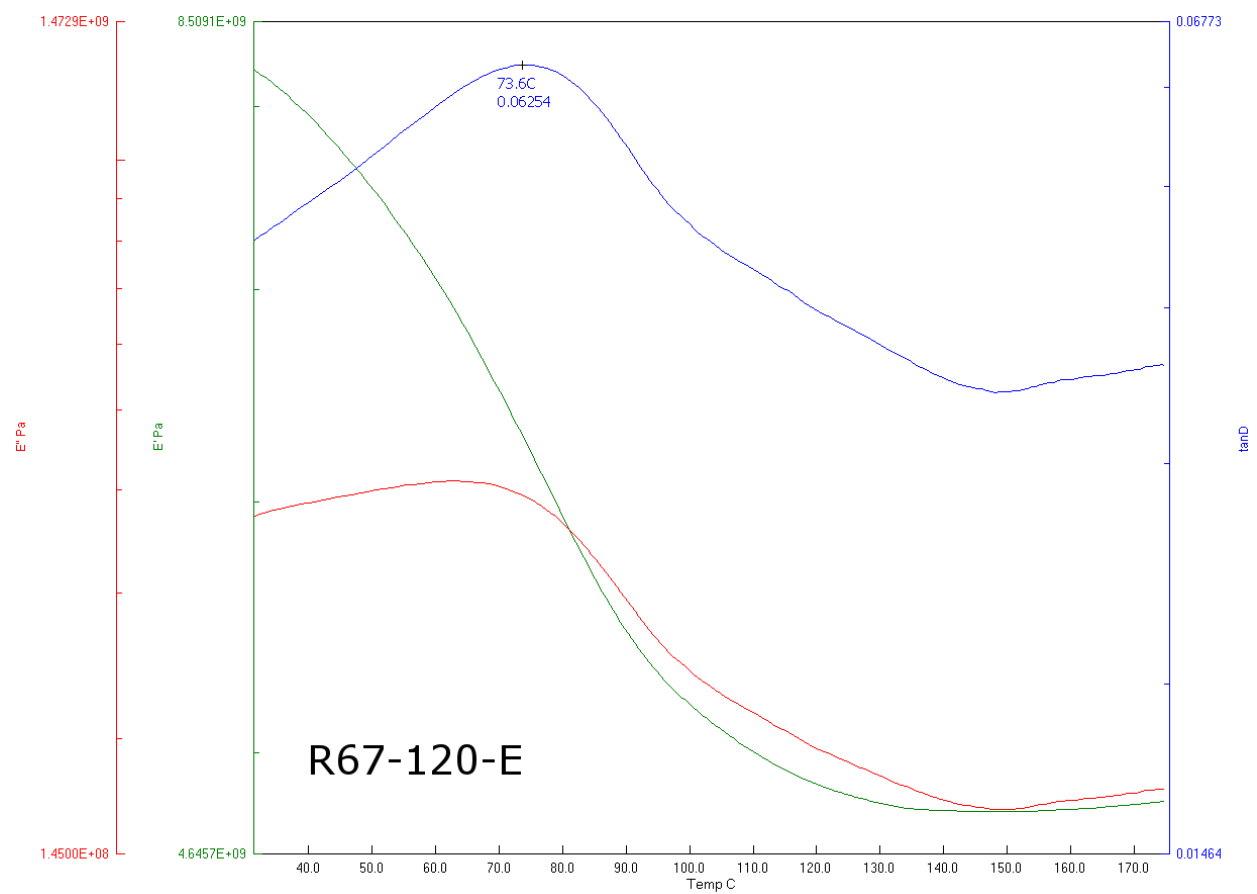
Figure 82: DMA output for R67-120-E
