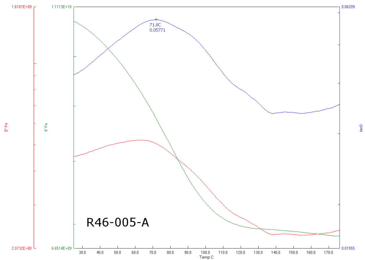
Figure 53: DMA output for R46-005-A
