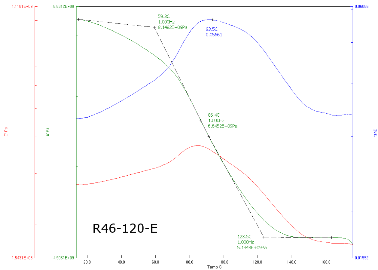
Figure 65: DMA output for R46-120-E
