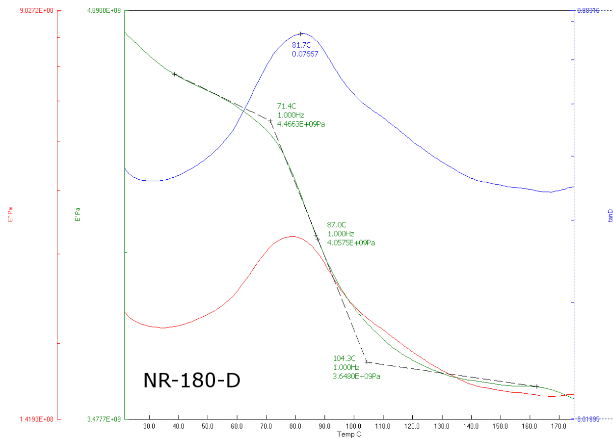
Figure 32: DMA output for NR-180-D
