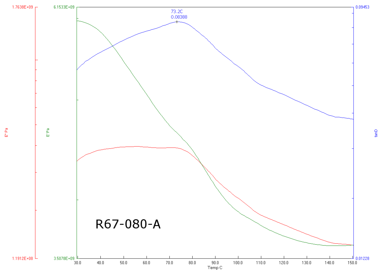
Figure 80: DMA output for R67-080-A
