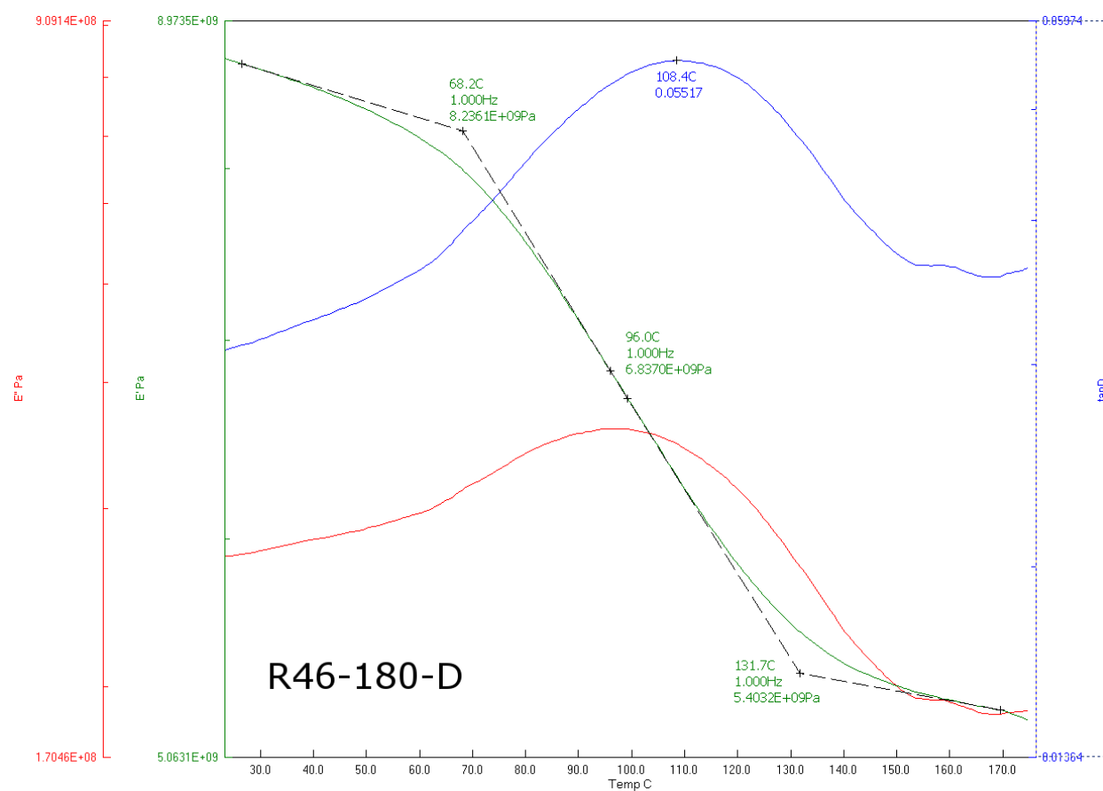
Figure 68: DMA output for R46-180-D
