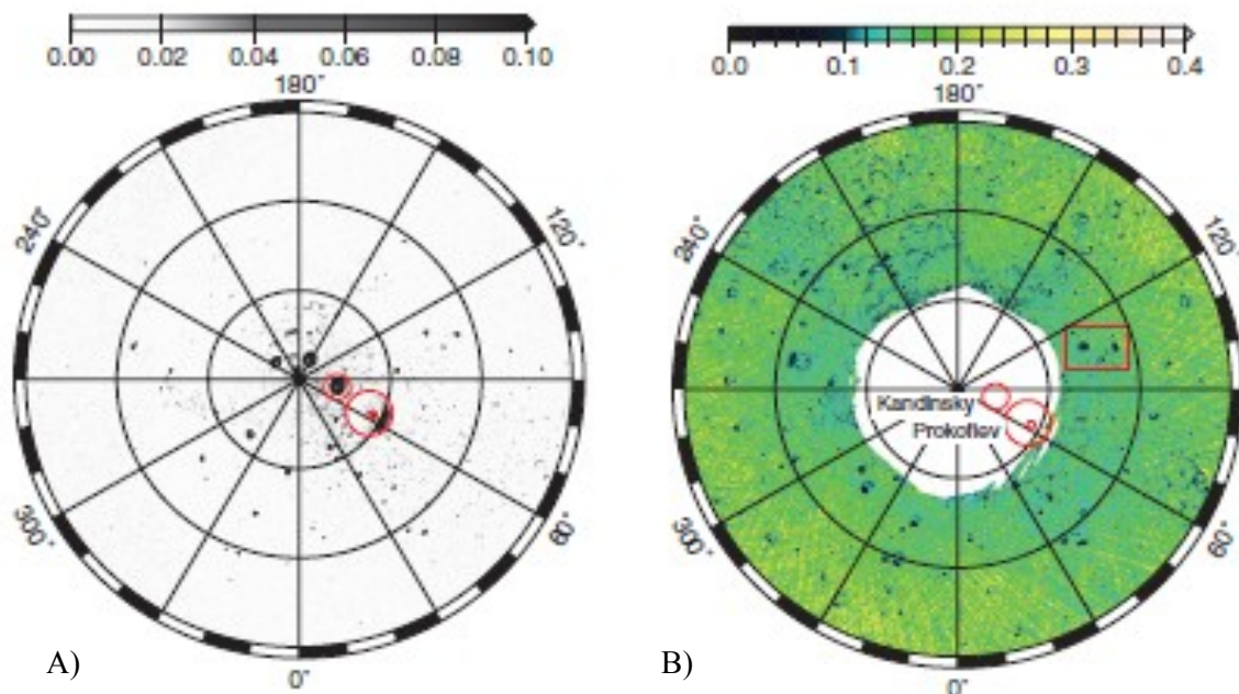
Figure 3. Maps of radar cross section and reflectance of Mercury's northern polar region showing the permanently shadowed regions of craters. A) Earth-based radar imagery with high backscatter suggestive of cold volatiles B) The 1064-nm bidirectional reflectance from MESSENGER (Neumann et al. 2013).
