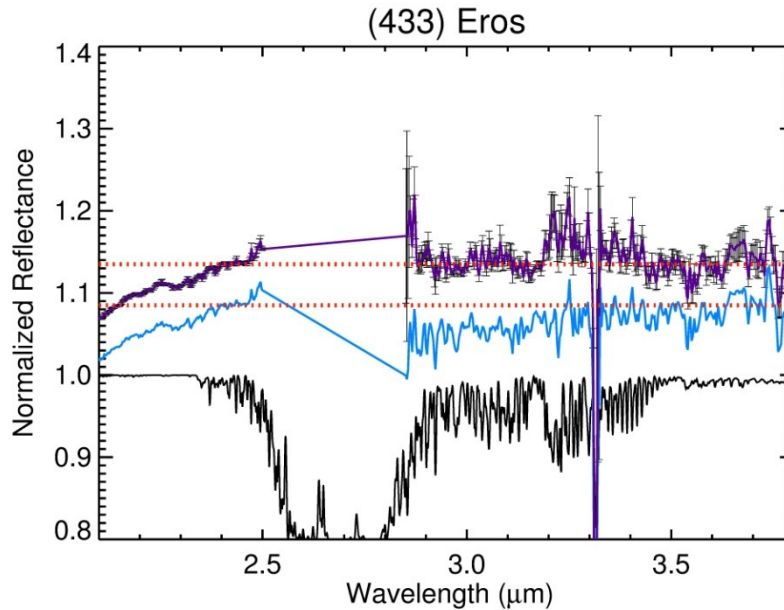
Figure 5. Overcorrecting of the 3- \mu m feature of (433) Eros. The black line shows the atmospheric transmission above the IRTF. The purple line shows the overcorrected spectrum (shifted upward by 0.1), while the blue dots show the corrected spectrum (shifted upward by 0.05). In both cases these spectra show the 2012 observation of Eros with only the reflected component of the light (i.e., thermal tail removed). The red dots show the continuum used for thermal correction and band depth computation for both of the spectra. Error bars are shown on the purple data points, but left off of the blue data points, for clarity.
