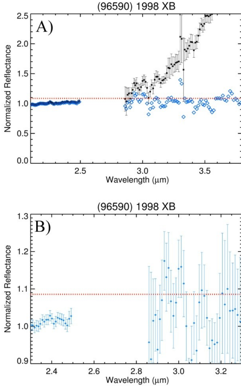
Figure 13. a) Reflectance spectra of the 3- \mu\text{m} feature of (96590) 1998 XB. The black dots show the spectrum with the thermal contribution, while the blue dots show only the reflected component of the light (i.e., thermal tail removed), and red dots the continuum used for thermal correction and band depth computation. Error bars are shown on the black data points for a, but left off of the blue data points, for clarity. b) Zoomed-in version of the thermally corrected spectrum.
