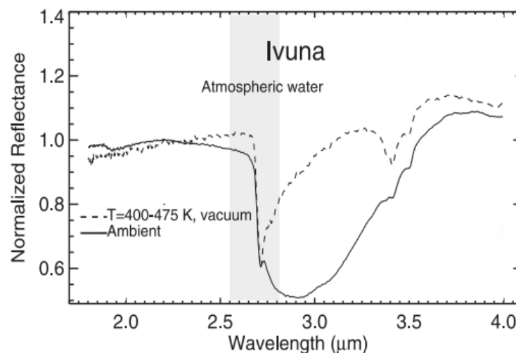
Figure 4. 3- \mu\text{m} spectroscopy of the carbonaceous chondrite Ivuna. The phyllsilicate band center is at 2.7- \mu\text{m} (Takir et al. 2013).
