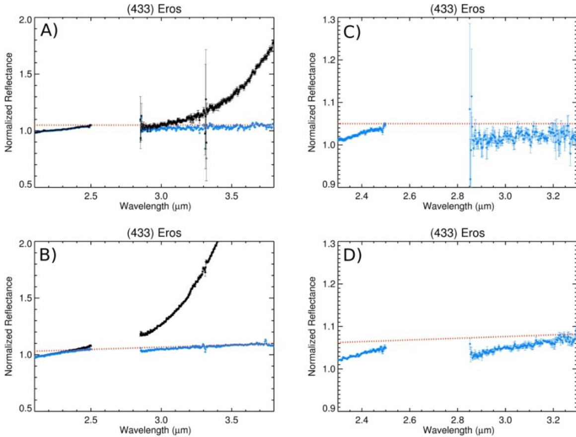
Figure 9. Reflectance spectra of the 3- \mu m feature of (433) Eros. a) LXD spectra of the September 1, 2009 observation of Eros. b) LXD spectra of the January 28, 2012 observation of Eros. c) The thermally corrected spectrum from September 1, 2009 zoomed in to better illustrate the 3- \mu m region. d) The thermally corrected spectrum from spectrum from January 28, 2012 zoomed in to better illustrate the 3- \mu m region. The black dots show the spectrum with the thermal contribution, while the blue dots show only the reflected component of the light (i.e., thermal tail removed), and red dots the continuum used for thermal correction and band depth computation. Error bars are shown on the black data points on A and B, but left off of the blue data points, for clarity.
