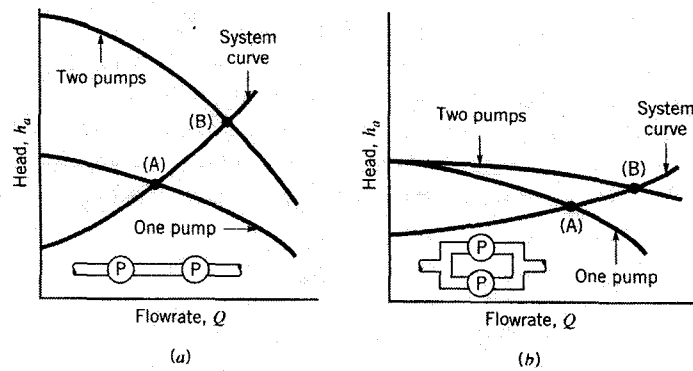
Figure II-4: (a) The effect on the pump curve for operating pumps in series is to add the head rise at a given flowrate. (b) The effect on the pump curve for operating pumps in parallel is to add the flowrates for a given head rise. [Reproduced from Munson (11)].
