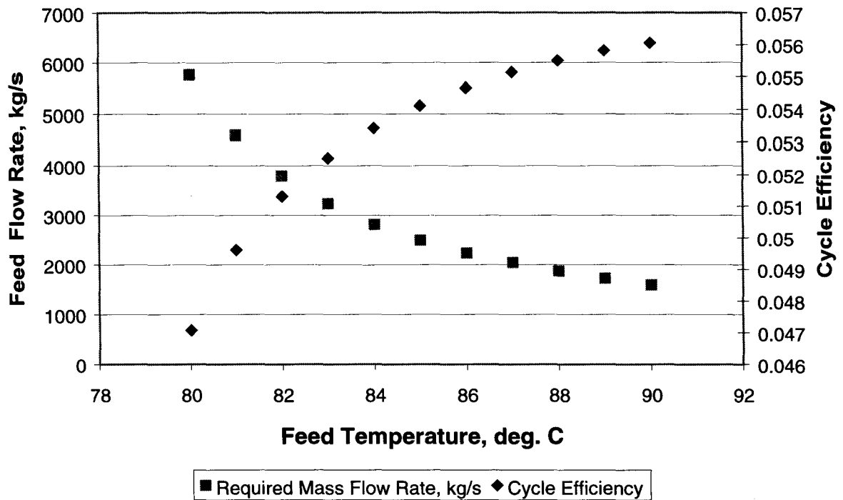
Figure V-3: System characteristics as a function of feed (pond) temperature, assuming a salinity of 150 gm/kg and a flash pressure 28700 Pa. Available power from the system is approximately 5 MW.
