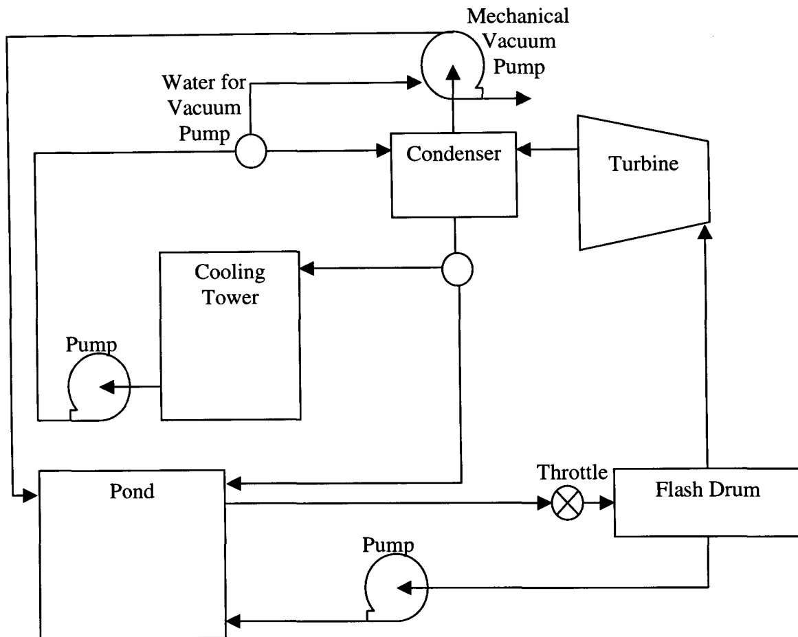
Figure I-2. Flash cycle for salt-gradient solar pond power generation.
