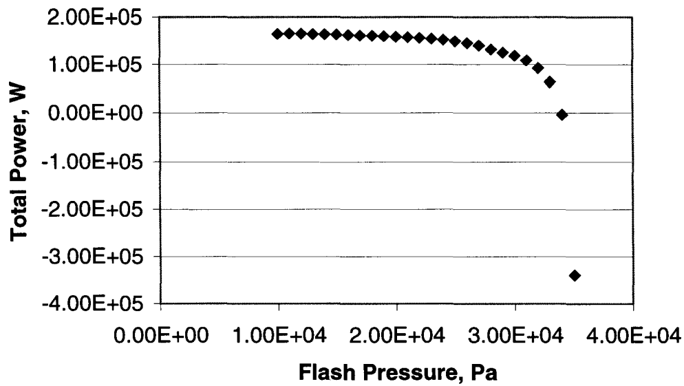
Figure III-3: The effect of flash pressure on the total available power, per 1 kg/s through turbine with brine salinity of 150 gm/kg.
