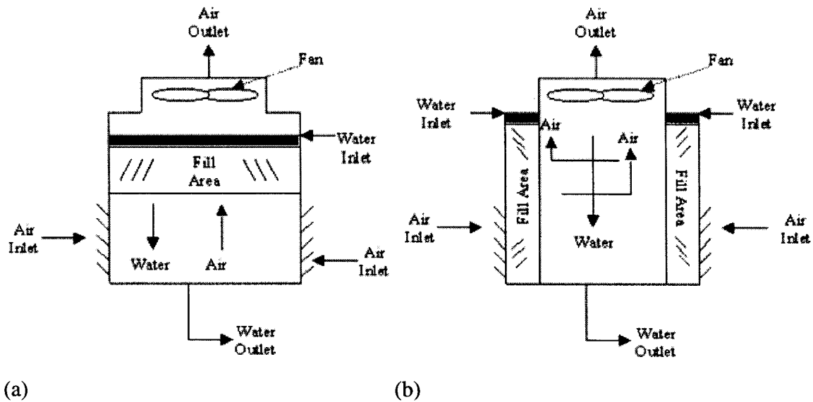
Figure II-7: Mechanical Draft Cooling Towers. a) Forced-draft Cooling Tower b) Induced-draft Cooling Tower (Reproduced from 18.)
