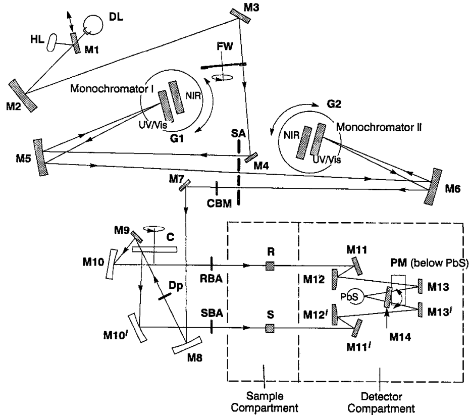
Figure 2.4: Optical layout of Perkin-Elmer λ-900
