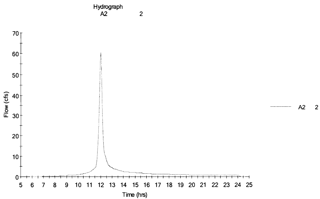
Figure 24 – A2 Postdevelopment 2 Year
