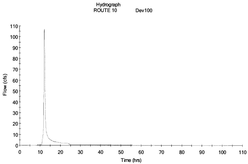
Figure 19 – A1 Routed 100 Year
