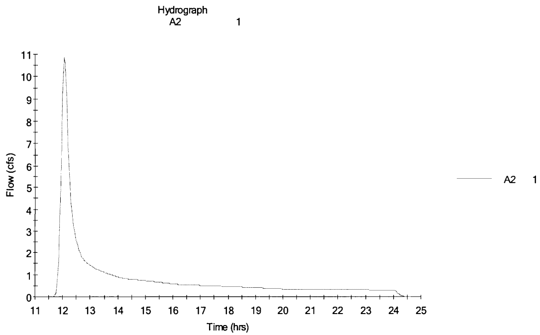
Figure 20 – A2 Predevelopment 1 Year
