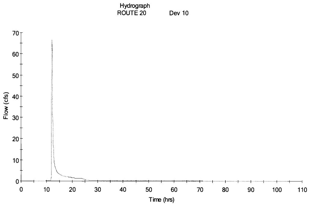
Figure 31 – A2 Routed 10 Year
