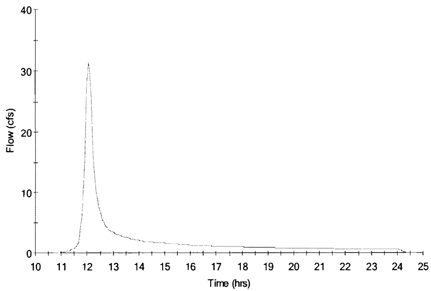
Figure 8 – A1 Predevelopment 2 Year
