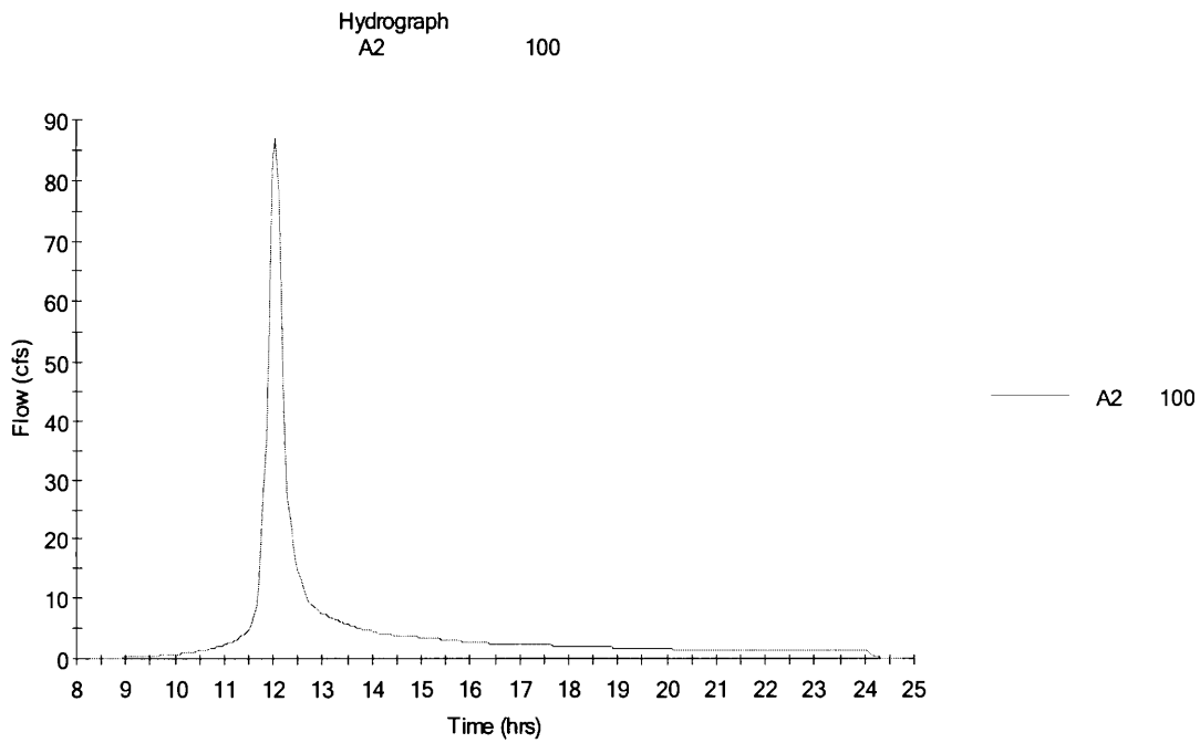
Figure 32 – A2 Predevelopment 100 Year
