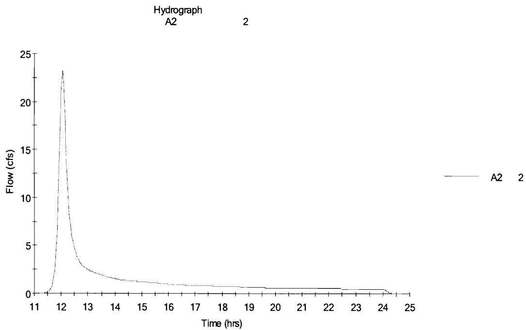
Figure 23 – A2 Predevelopment 2 Year
