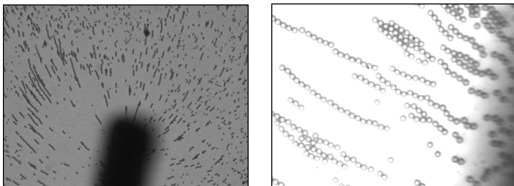
Figure 27. DEP pearl chains formed around the electrode tips by latex particles. The picture on the left is taken at 20X objective lens while the picture on the right is the detailed look at the pearl chain using 100X lens.
