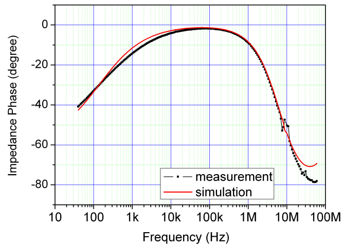
Figure 14. Comparison of impedance phase angle for measured and simulation data for low conductivity solution (20 mS/m). The spacing between the electrodes is 200 \mu\text{m} .
