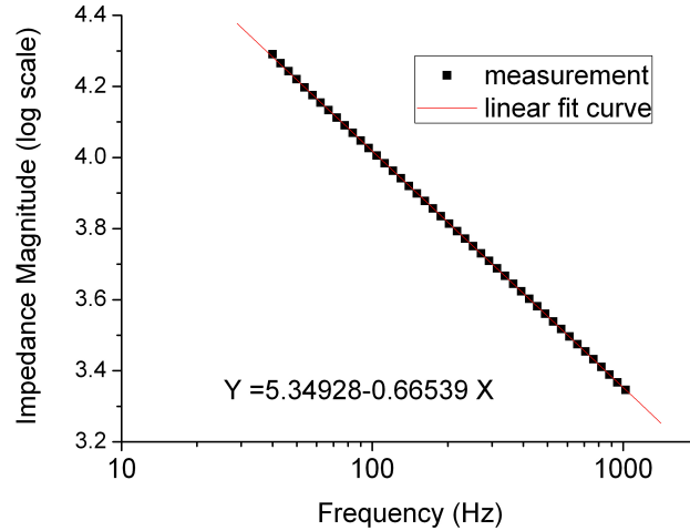
Figure 12. Double layer impedance measurement and fit curve ( \sigma = 20 \text{ mS/m} ). The measured data fits perfectly with linear relationship, revealing the constant phase angle characteristics and validity of the double layer impedance model.
