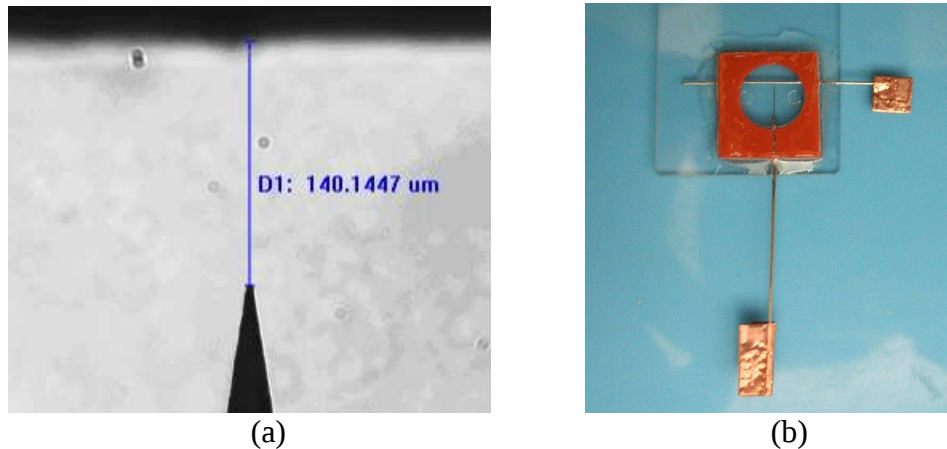
Figure 8. Orthogonal electrodes configuration used in the research. (a) A sharp tip micromanipulator needle is used as the vertical electrode. The separation between electrodes is measured to be 140\text{ }\mu\text{m} , (b) orthogonal electrode pair fitted in the slip cover chamber on a glass slide.
