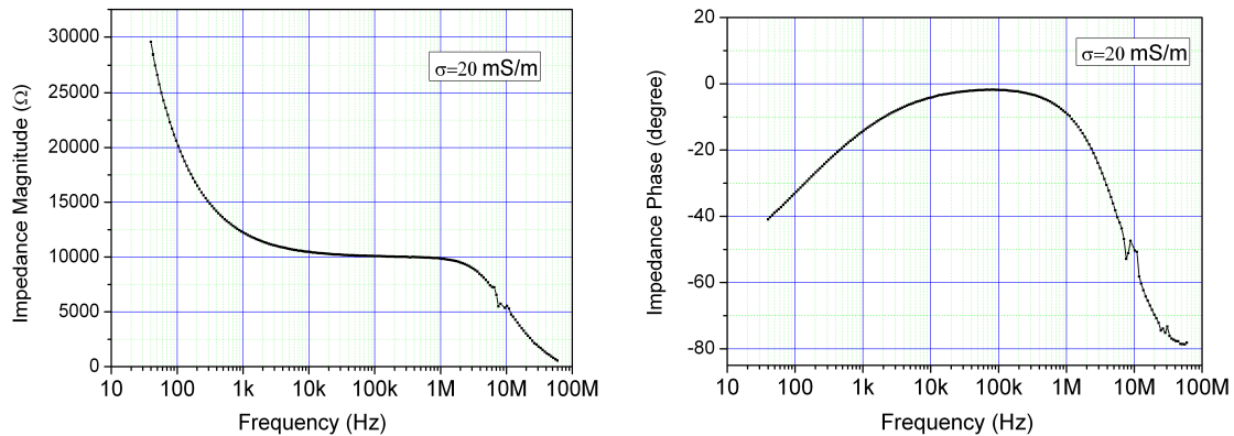
Figure 10. Impedance measurement of orthogonal electrode pair with \sigma=20 mS/m. Magnitude and phase information is plotted separately. The spacing between the electrodes is 200 \mu\text{m} and measurement is excited by 0.5 volt signal.
