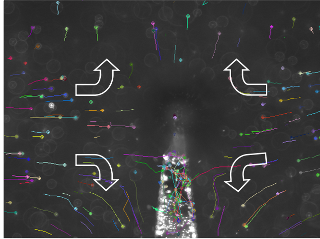
Figure 18. Flow pattern at 200 Hz and 20 Vpp. At electrode tip, some tracer particles go to the gap between the electrodes as compared with the capacitive charging that causes the ACEO flow in figure 12. Arrows show the directions of flows.
