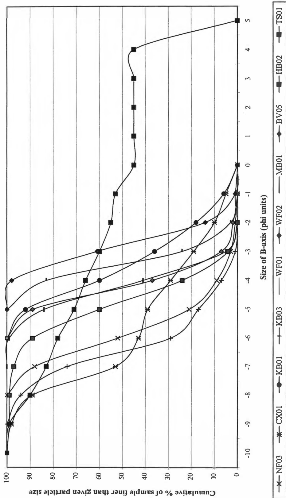
Figure 3-4. Particle Size Distributions
