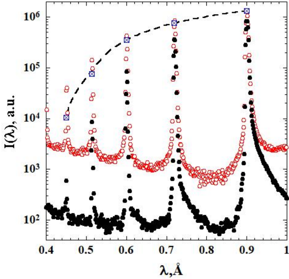
Figure V.4 - Spectra of the Cu (111) PM (red open circles) and Si (220) M (black closed circles) matched at \lambda_4 = 0.9 Å. The Bragg-peak intensities \delta\theta_4 I(\lambda_n)_M / \delta\theta_n normalized for n = 4 are shown by blue crossed rectangles connected by the dashed line.
