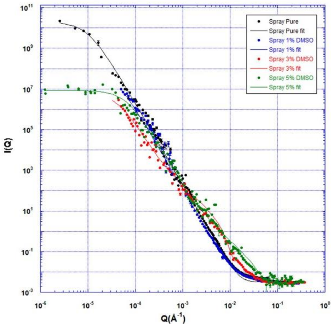
Figure II.3 – Plot of neutron scattering intensity ( I(Q) ) as a function of Q ( \text{\AA}^{-1} ) for spray-coated films. SANS data for Pristine (black), 1%wt DMSO (blue), 3%wt DMSO (red), and 5%wt DMSO (green) solutions are dots and corresponding fits to Equation 1 are lines.
