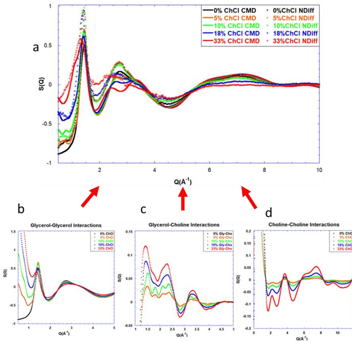
Figure IV.3 – S(Q) plots for wide-angle neutron diffraction a) compared to classical molecular dynamic simulations over a range of 0-10 \text{ \AA}^{-1} , b) glycerol-glycerol interactions, c) glycerol-choline interactions, d) choline-choline interactions.
