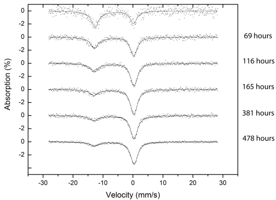
Figure 44 Mössbauer spectra of \text{EuCl}_3 heated at 700\text{ }^\circ\text{C} for an hour as a function of time.
