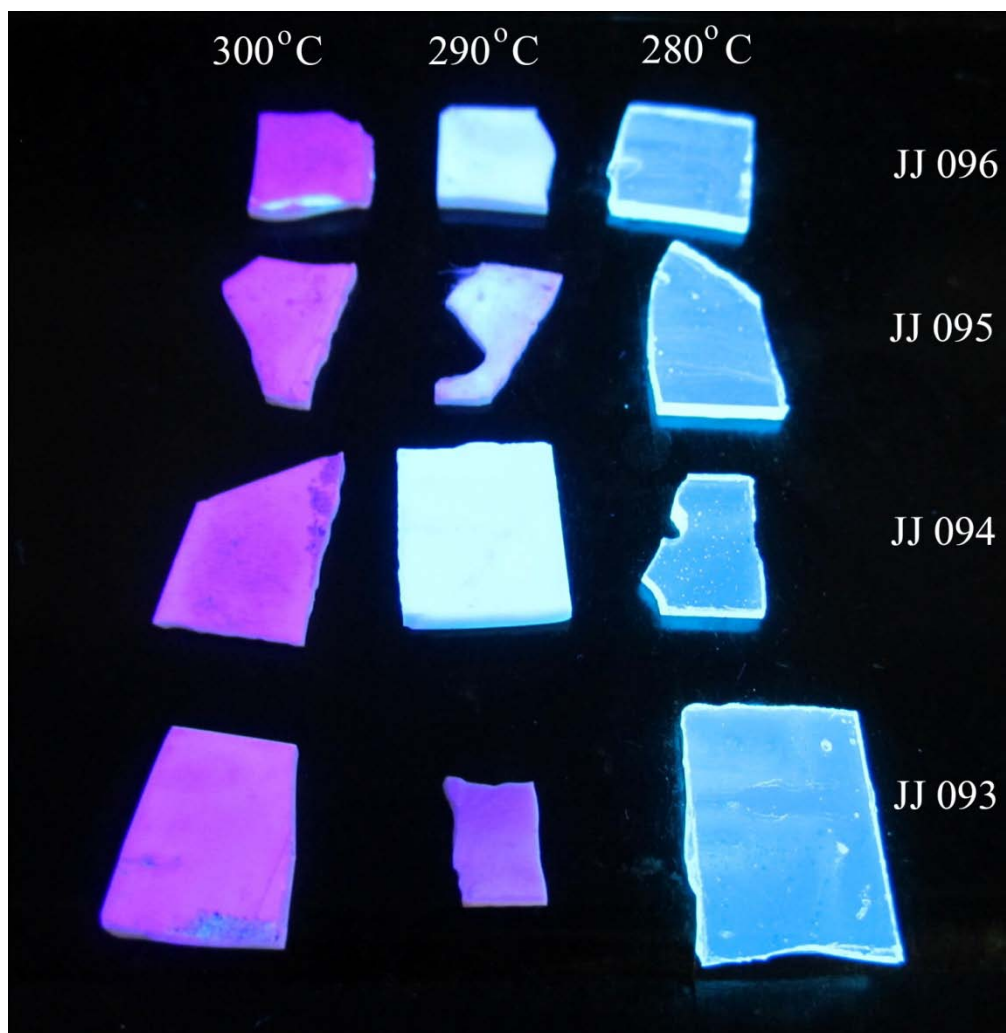
Figure 34 Photoluminescence test under UV light on ZBLAN glass sample doped with 2 % \text{Eu}^{2+} after annealing at different temperatures for 5 min.
