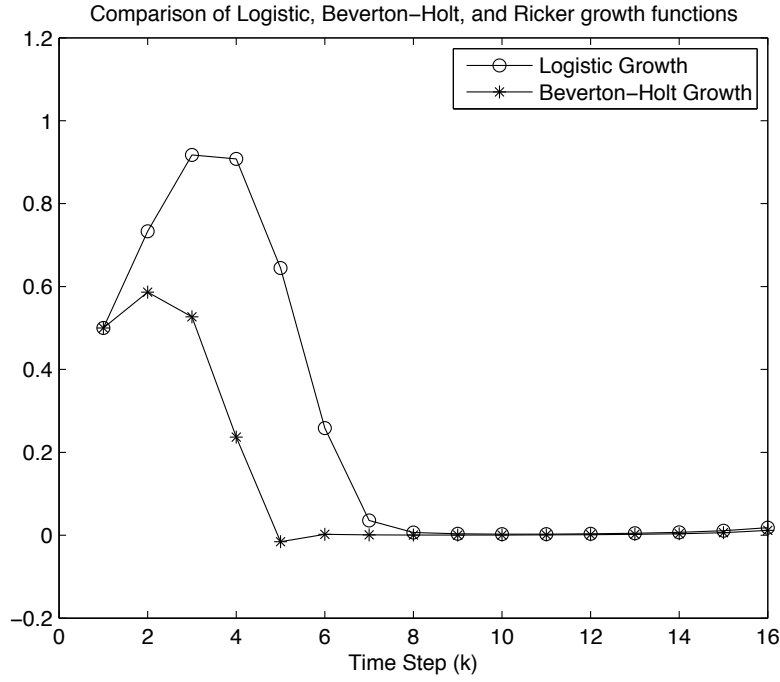
FIGURE 13. Logistic growth function and Beverton-Holt growth function without control. For the logistic growth function, c = 1.0, d = 0.8, r = 0.2, K = 1.5, x_0 = 0.5 , and y_0 = 1.0 . For the Beverton-Holt growth function, R = 1.1, d = 0.8, r = 0.9, K = 2.0, x_0 = 0.5 , and y_0 = 1.0
