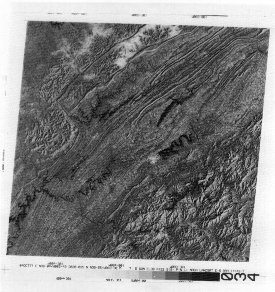
Figure 8. Landsat Scene E5899-141427, Band 7, 4 October 1977. Scale: 1:116,600.
