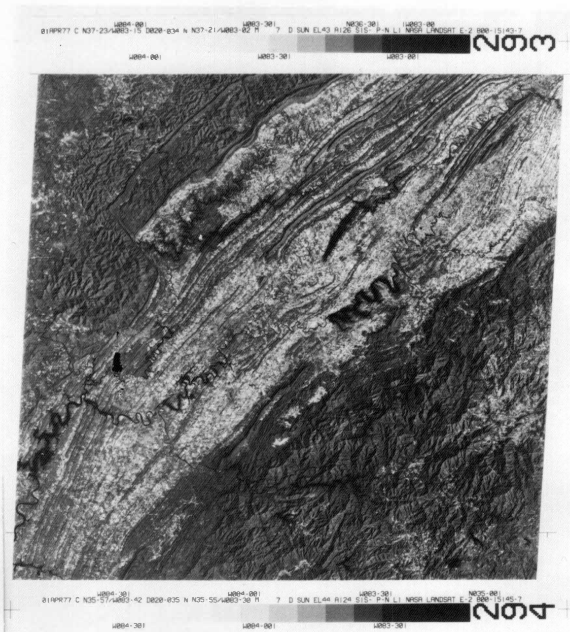
Figure 6. Landsat Scene E2800-151457, Band 7, 1 April 1977. Scale: 1:116,600.
