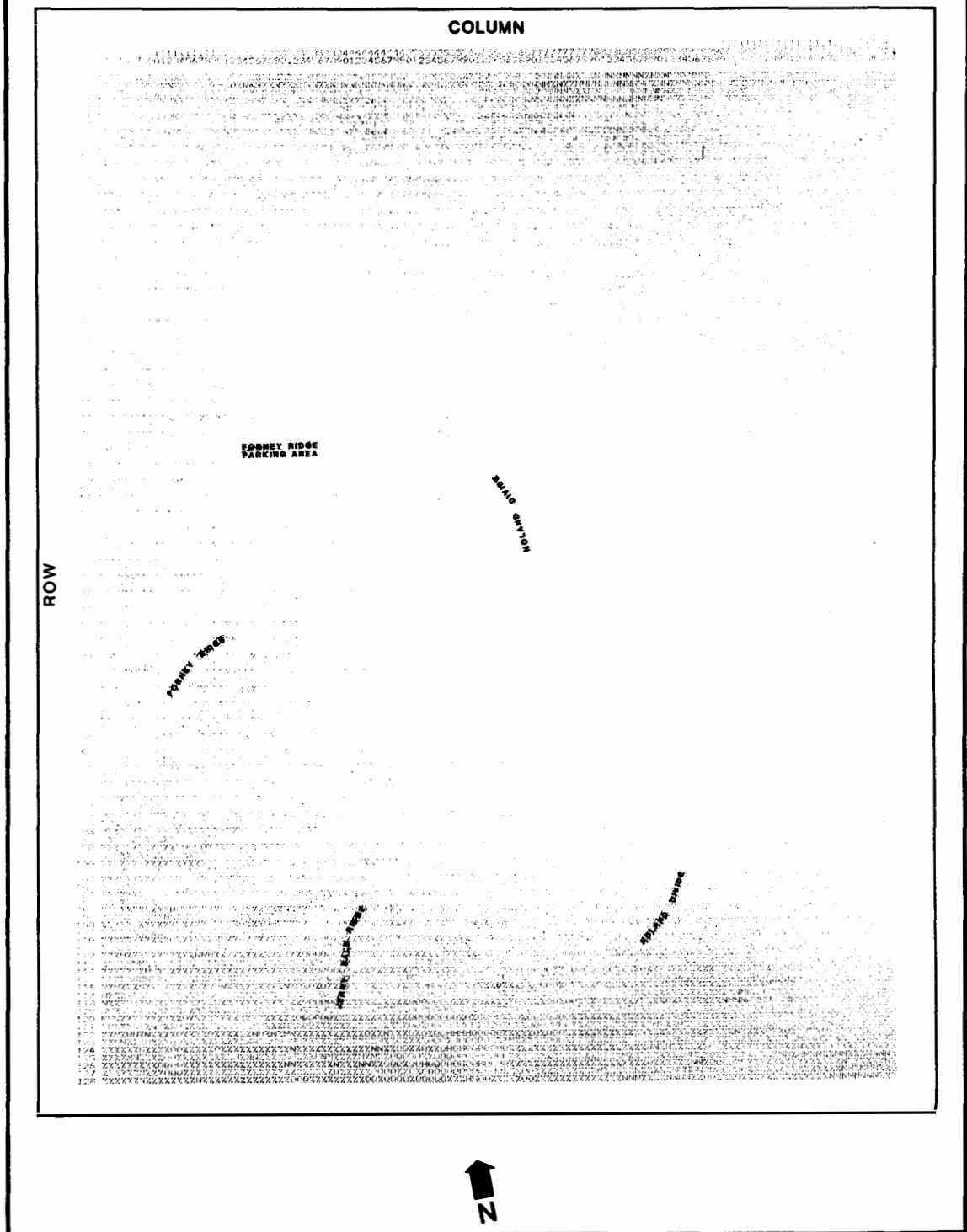
Figure 30. Gray Scale Map for Band Ratio Transformation of Scene GSM77R.
