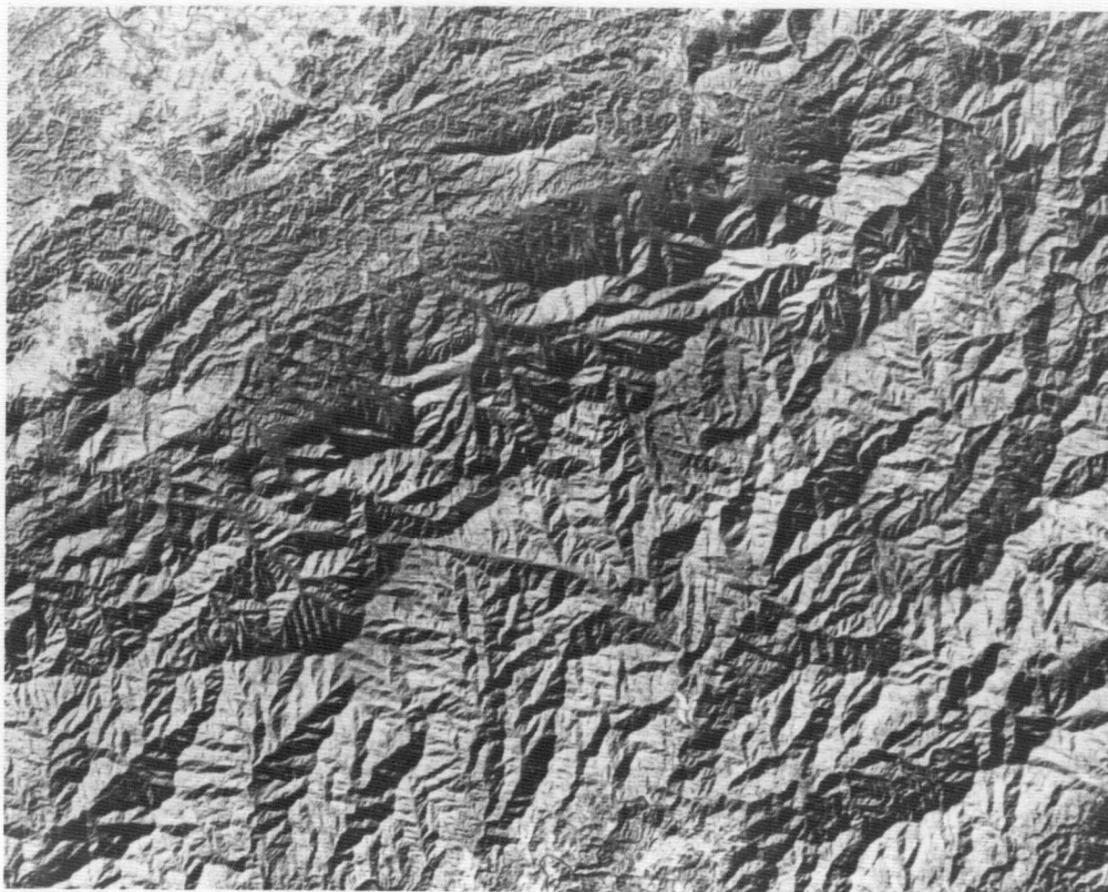
Figure 23. Enlarged Landsat Scene E2692-151927, Band 7, 14 December 1977. Scale: 1:375,000.
