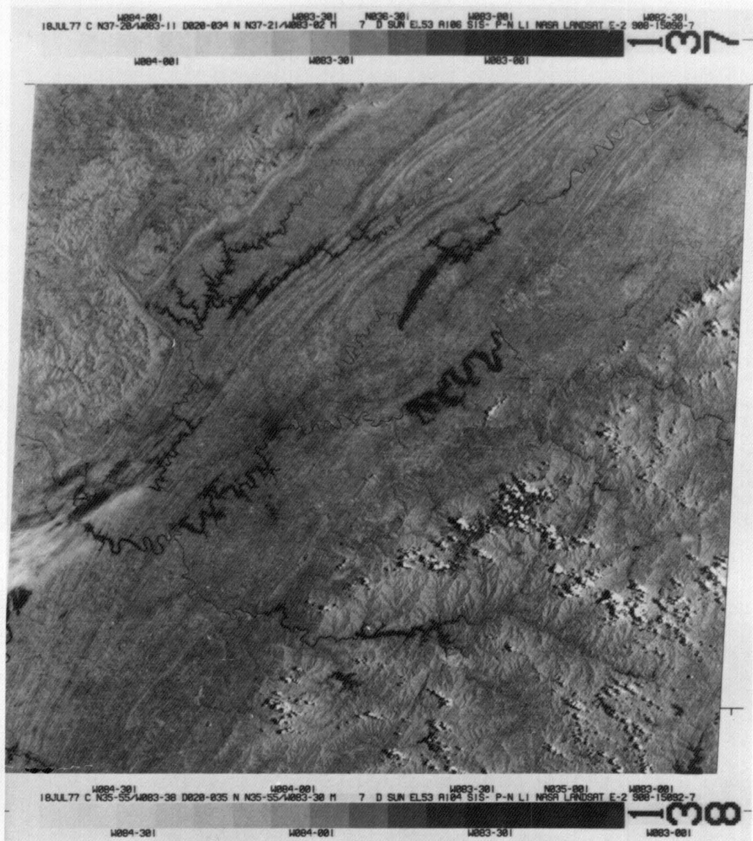
Figure 7. Landsat Scene E2908-150927, Band 7, 18 July 1977. Scale: 1:116,600.
