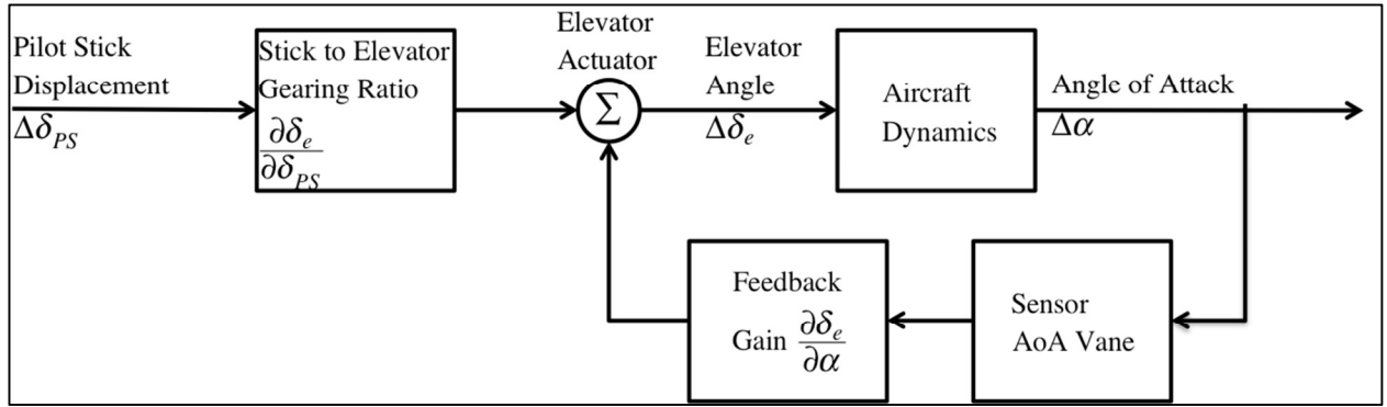
Figure 4.1 Simple Angle of Attack Feedback System
