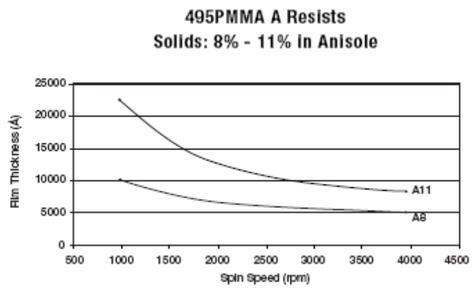
Figure 2.23: Spin Curves for 495K PMMA formulated in Anisole [40]
