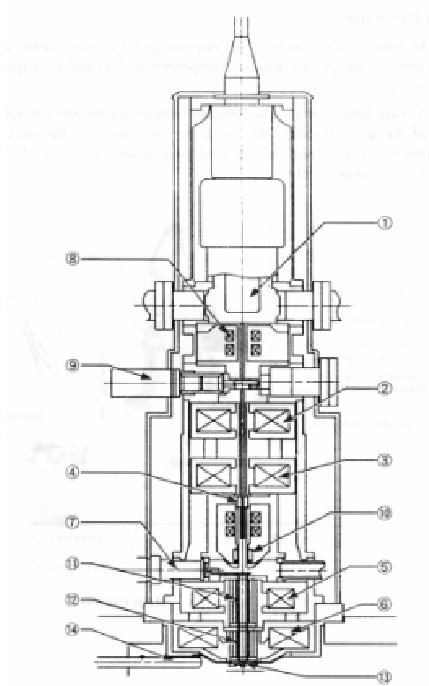
Figure 2.10: Gun Column for JBX 6000 FS/E (Courtesy JEOL – Peabody, MA)
