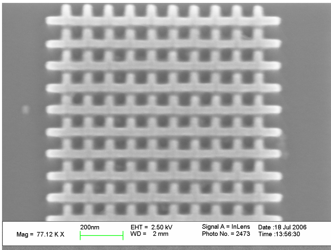
Figure 3.11: Calibration artifact with a pitch of 100 nm, and with dose in the range of 1300\text{C}\mu/\text{cm}^2 - 1400\mu\text{C}/\text{cm}^2 .
