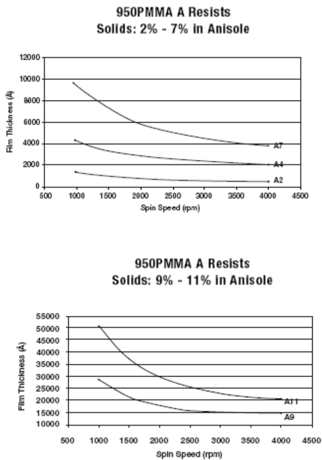
Figure 2.24: Spin Curves for 950K PMMA formulated in Anisole [40]
