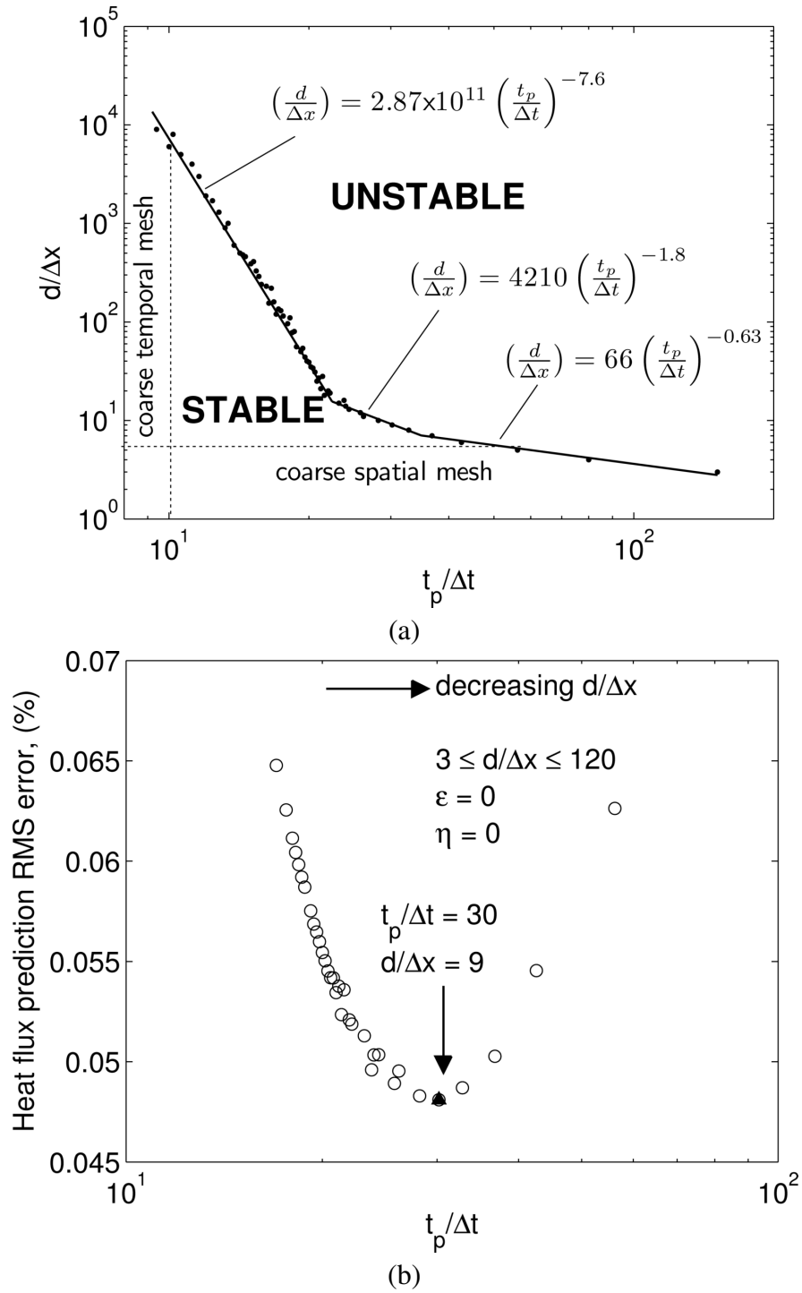
Figure 2.5: Optimization of mesh for test case 1. (a) Stability correlation relating the spatial mesh size ( d/\Delta x ) to the temporal mesh size ( t_p/\Delta t ) and (b) optimum mesh for both stability and accuracy.
