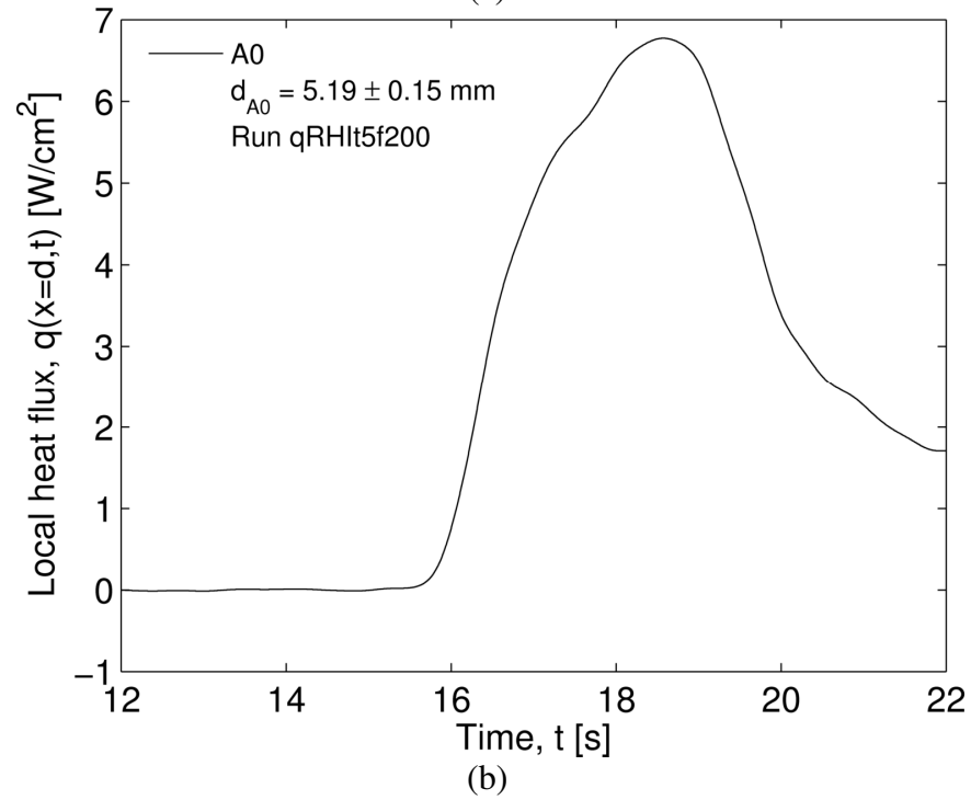
Figure 7.12: (a) Raw and LCSR-shifted experimental A0 data for run qRHIt5f200 and (b) resulting local heat flux for probe A0.
