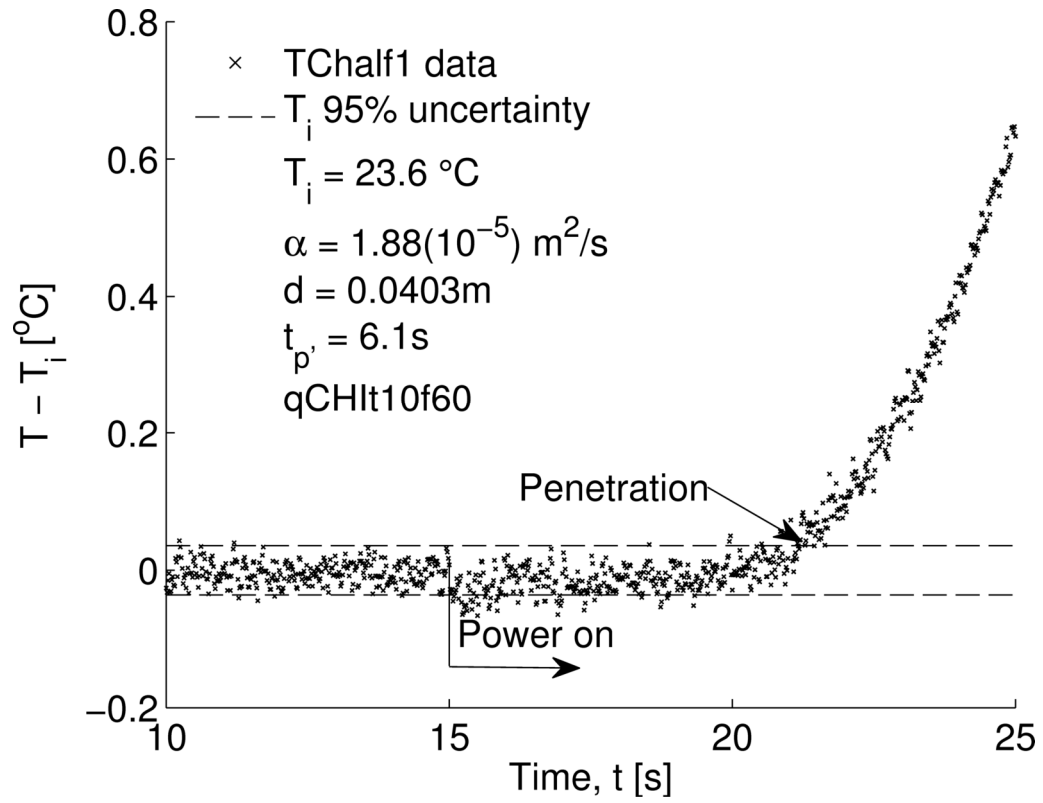
Figure 7.1: Penetration time of back surface with run qCHlt10f60 where t_{p'} = t_{on} + t_p .
