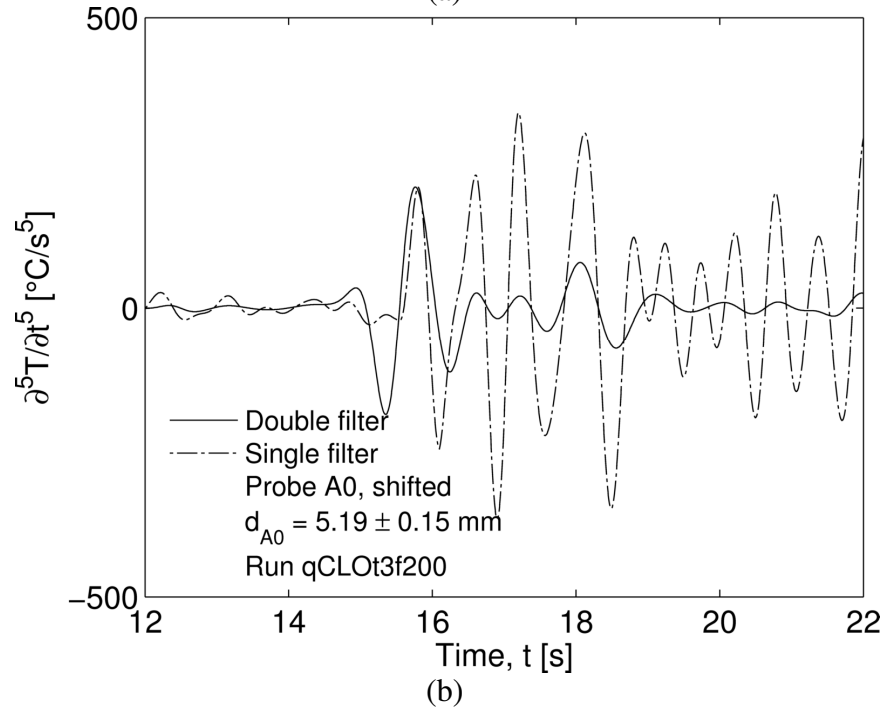
Figure 7.14: (a) First and (b) fifth time derivative of shifted temperature data from run qCLOt3f200 with f_c = 0.9 \text{ Hz} .
