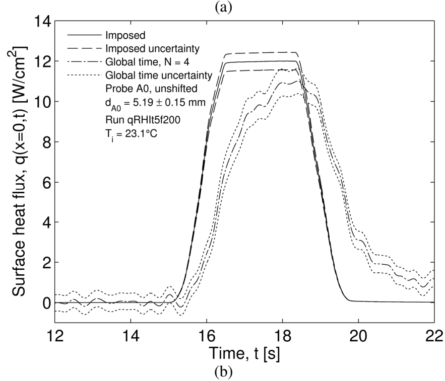
Figure 6.2: Inverse predicted surface temperature and heat flux using sandwich experiment data from run qRHIt5f200, uncorrected for response time. (a) Surface temperature with uncertainty band and (b) surface heat flux with uncertainty band. Data used can be seen in Figure 6.1.
