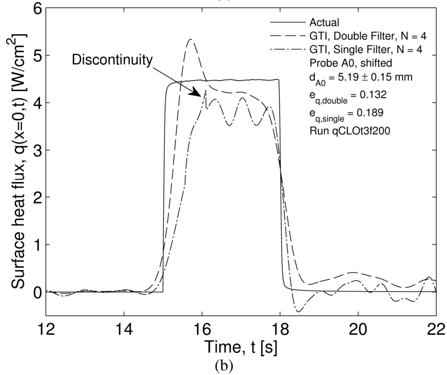
Figure 7.15: Global time inverse (a) temperature and (b) heat flux results using global time inverse method with N = 4 and f_c = 0.9 Hz for run qCLOt3f200. Discontinuity seen when single filter method of obtaining time derivatives is employed. The error norms were calculated over 12\text{s} \leq t \leq 22\text{s} .
