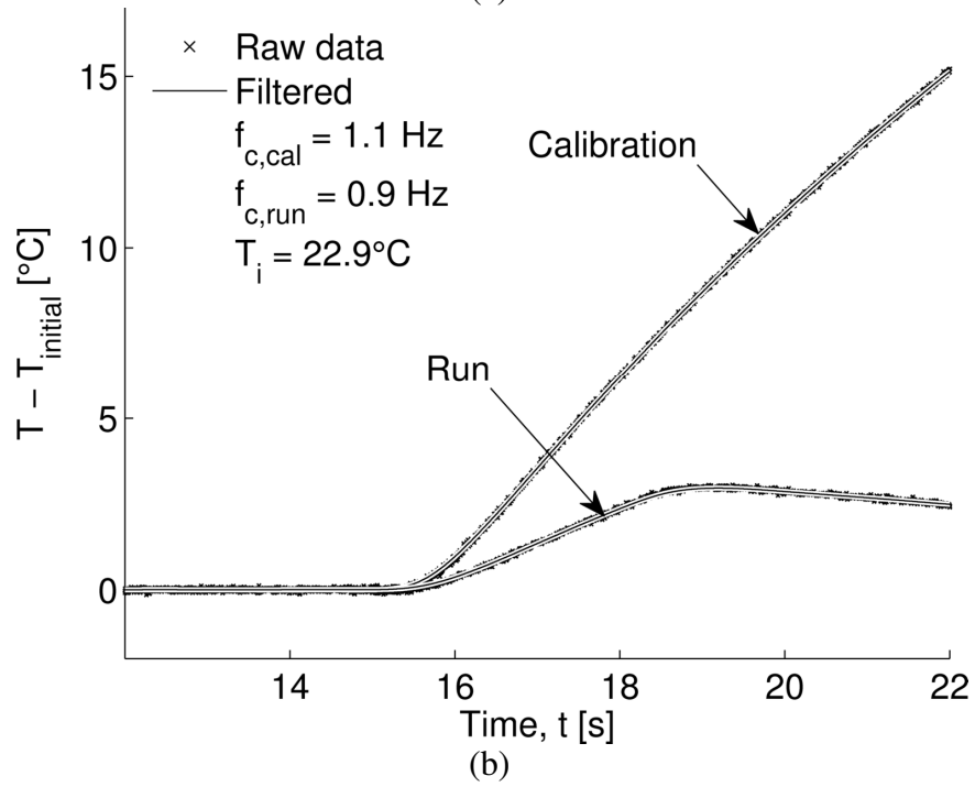
Figure 7.20: Calibration integral method data for calibration qCHIt10f200 and real run qCLOt3f200 . (a) Actual calibration and real run heat flux and (b) calibration and real run temperature histories.
