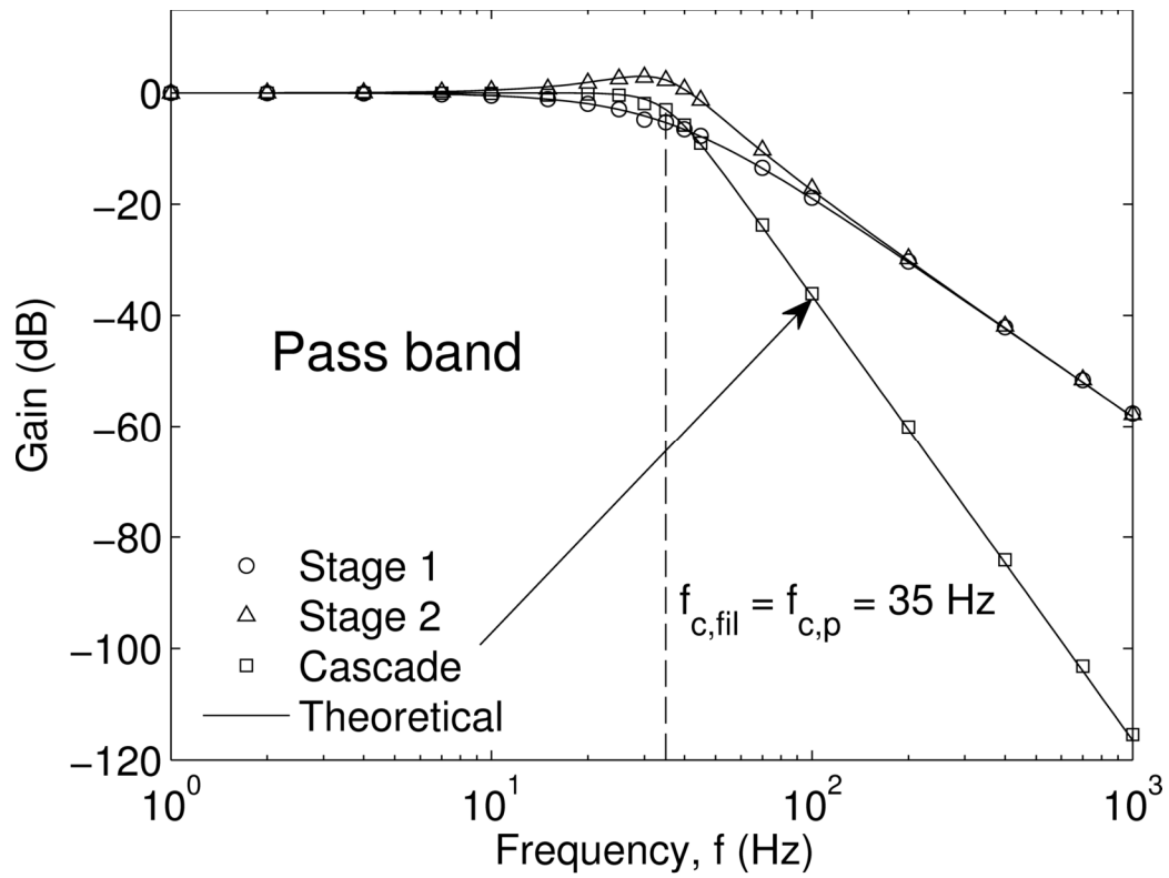
Figure 4.10: Butterworth filter characteristics as a function of frequency for each stage and as a cascaded filter indicating f_{fil} = f_{c,p} = 35 Hz as designed.
