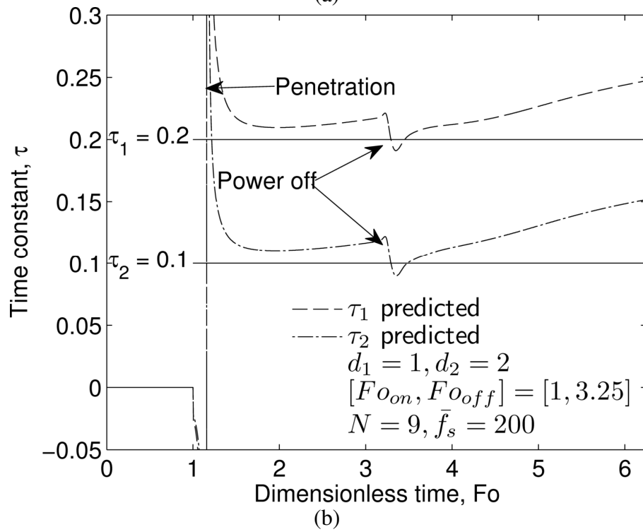
Figure 6.13: Effect of varying (a) number of derivatives used and (b) sampling rate on the resulting Two-Probe Taylor series results using simulated data.
