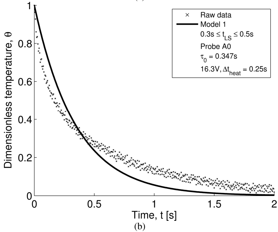
Figure 6.6: Model 1 results for LCSR testing of probe A0. (a) Sensitivity coefficient and (b) comparison of model with raw data. Testing parameters were V_{RMS} = 16.3V , \Delta t_{heat} = 0.25s , \Delta T = 12.7^\circ C , and f_s = 200 Hz.
