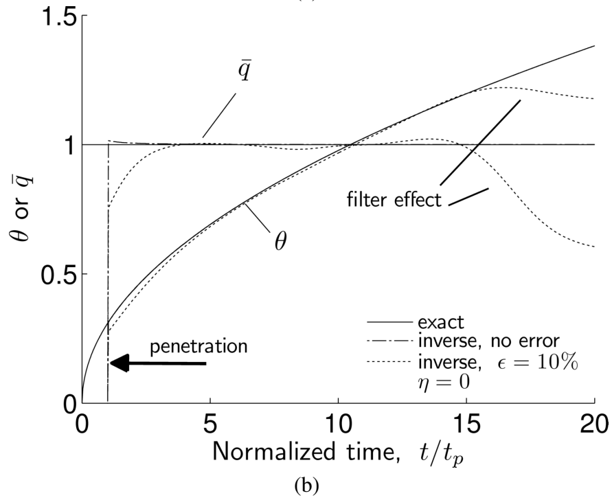
Figure 2.7: Effectiveness of filter at eliminating unwanted noise. (a) Noisy, filtered temperature and heat flux input data ( \eta = 1 ) used to predict (b) surface ( \eta = 0 ) conditions. Parameters used were \bar{f}_c = 2.0 , d/\Delta x = 9 and t_p/\Delta t = 30 for test case 1.
