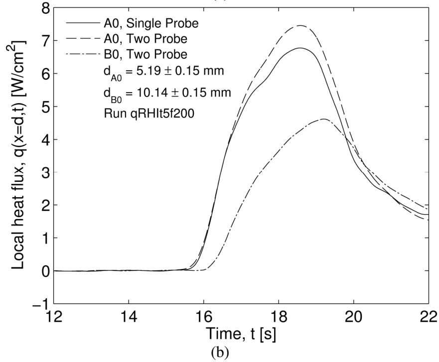
Figure 8.4: Inputs for inverse problem using data from run qRHIt5f200. (a) Raw, filtered, and shifted temperature data for both probes and (b) local heat flux at both probe sites using the single- and two-probe approach. Cutoff frequencies used were f_{c,A0} = 1.5 Hz and f_{c,B0} = 1.1 Hz.
