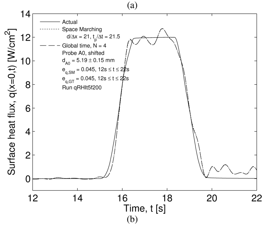
Figure 8.5: Two-probe inverse results for surface (a) temperature and (b) heat flux. Data used from run qRHIt5f200 seen in Figure 8.4.
