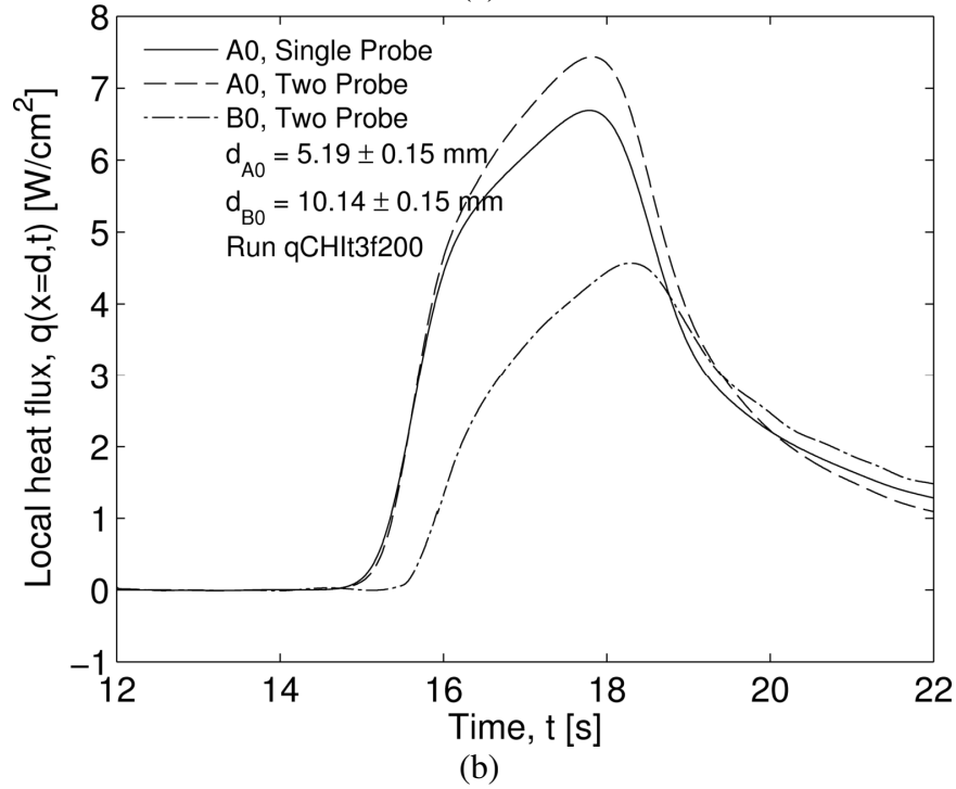
Figure 8.2: Inputs for inverse problem using data from run qCHIt3f200. (a) Raw, filtered, and shifted temperature data for both probes and (b) local heat flux at both probe sites using the single- and two-probe approach. Cutoff frequencies used were f_{c,A0} = 0.9 Hz and f_{c,B0} = 1.1 Hz.
