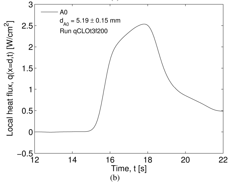
Figure 7.6: (a) Direct FD model temperature history at probe A0 depth compared with LCSR-shifted experimental A0 data and (b) resulting local heat flux using semi-infinite medium integral equation. Experimental data was regularized with f_c = 0.9\text{ Hz} .
