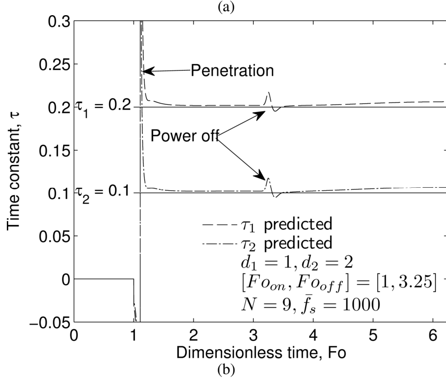
Figure 6.12: Two-Probe Taylor Series method results with simulated data. (a) Input dimensionless data and (b) resulting time constant prediction with N = 9 , \bar{f}_s = 1000 .
