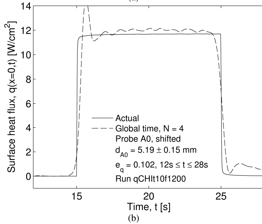
Figure 8.11: Effect of increasing the data density on the two-probe global time inverse results for surface (a) temperature and (b) heat flux. Data used from run qCHlt10f1200 seen in Figure 8.10.
