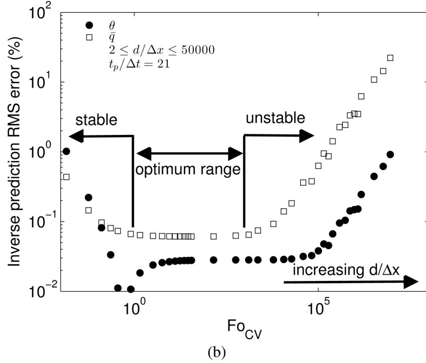
Figure 2.4: Inverse prediction RMS error for test case 1 over the interval 5 < t/t_p < 15 for the dimensionless surface temperature and heat flux values using exact data for (a) fixed nodal spacing and (b) fixed temporal mesh.
