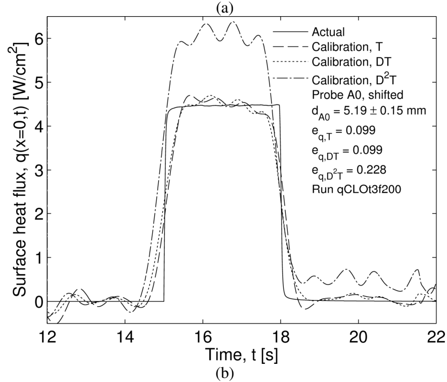
Figure 7.22: Calibration integral method inverse results for (a) temperature and (b) heat flux using calibration run qCHIt10f200 ( f_c = 1.1 Hz) and real run qCLOt3f200 ( f_c = 0.9 Hz). The error norms were calculated over 12\text{s} \leq t \leq 22\text{s} .
