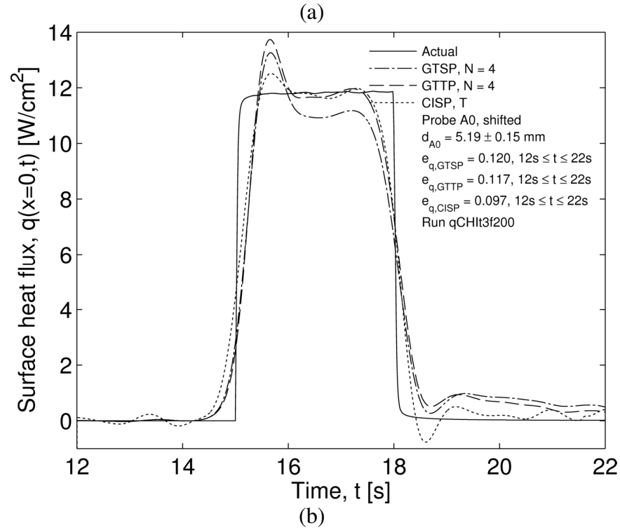
Figure 8.6: Comparison of two-probe inverse results with single-probe global time and calibration integral method for surface (a) temperature and (b) heat flux. Data used from run qCHIt3f200 seen in Figure 8.2.
