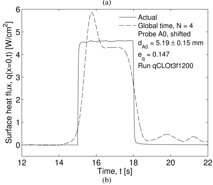
Figure 7.16: Effect of increased sampling rate on global time inverse method. Inverse (a) temperature and (b) heat flux results for run qCLOt3f1200 using global time inverse method with N = 4 and f_c = 0.9 Hz. The error norms were calculated over 12\text{s} \leq t \leq 22\text{s} .
