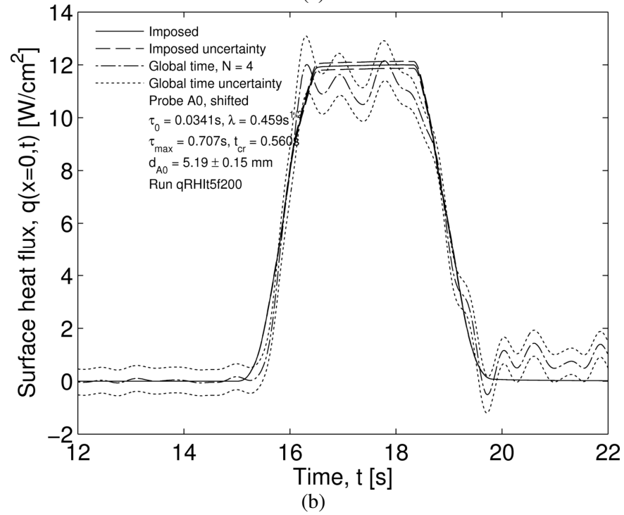
Figure 6.11: Inverse predicted surface temperature and heat flux using data corrected for response time. (a) Surface temperature prediction with uncertainty band and (b) Surface heat flux with uncertainty band. Data used for prediction can be seen in Figure 6.10 with one-probe analysis as detailed in Chapter 7.
