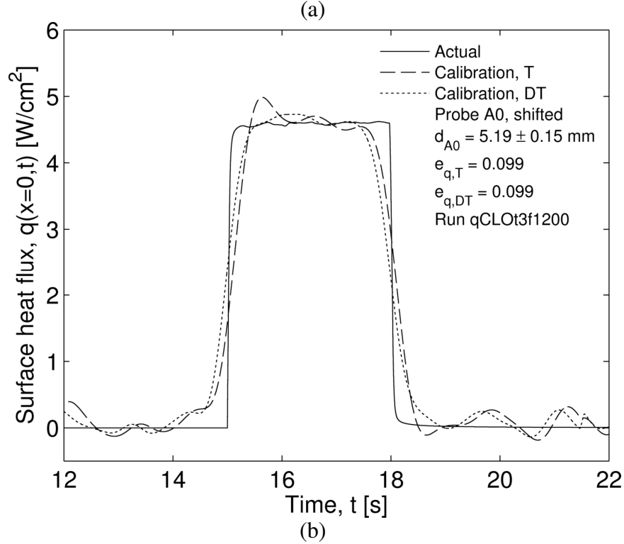
Figure 7.23: Calibration integral method inverse results for (a) temperature and (b) heat flux using calibration run qCHIt10f1200 ( f_c = 0.9 Hz) and real run qCLOt3f1200 ( f_c = 0.9 Hz). The error norms were calculated over 12\text{s} \leq t \leq 22\text{s} .
