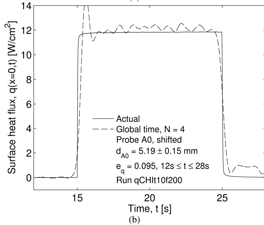
Figure 8.9: Two-probe inverse results for surface (a) temperature and (b) heat flux. Data used from run qCHlt10f200 seen in Figure 8.8. Note semi-infinite medium condition is violated at t = 22 s.
