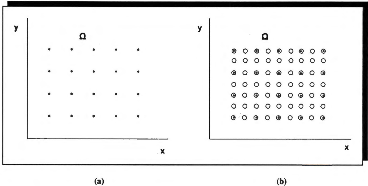
Figure 4. The refinement of numerical simulation by narrowing grid size: (a) coarse grid intervals, (b) fine grid intervals.
