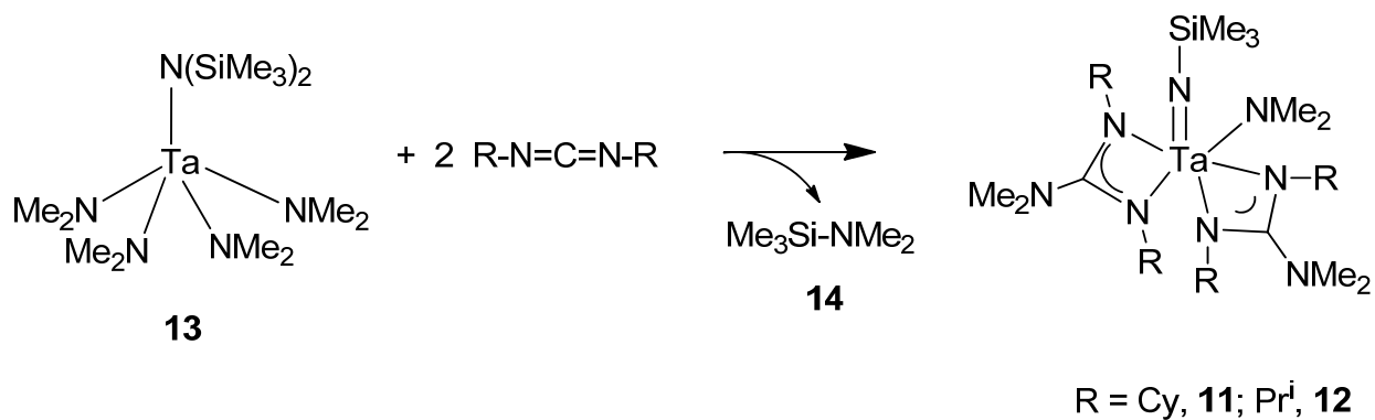
Scheme 4.3. Formation of 11 and 12 .
