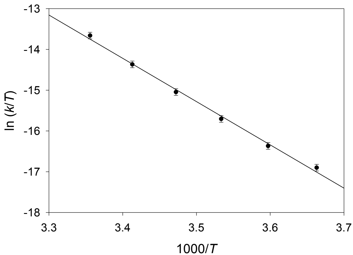
Figure 2.6. Eyring plot of the conversion of 1- d_{10} \rightarrow 2- d_7 .
