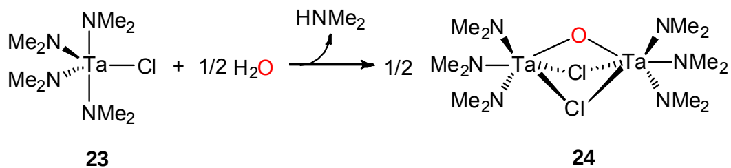
Scheme 5.3. Formation of [(\text{Me}_2\text{N})_3\text{TaCl}]_2\text{O} ( 24 ) from the reaction of \text{TaCl(NMe}_2)_4 ( 23 ) with water. 153
