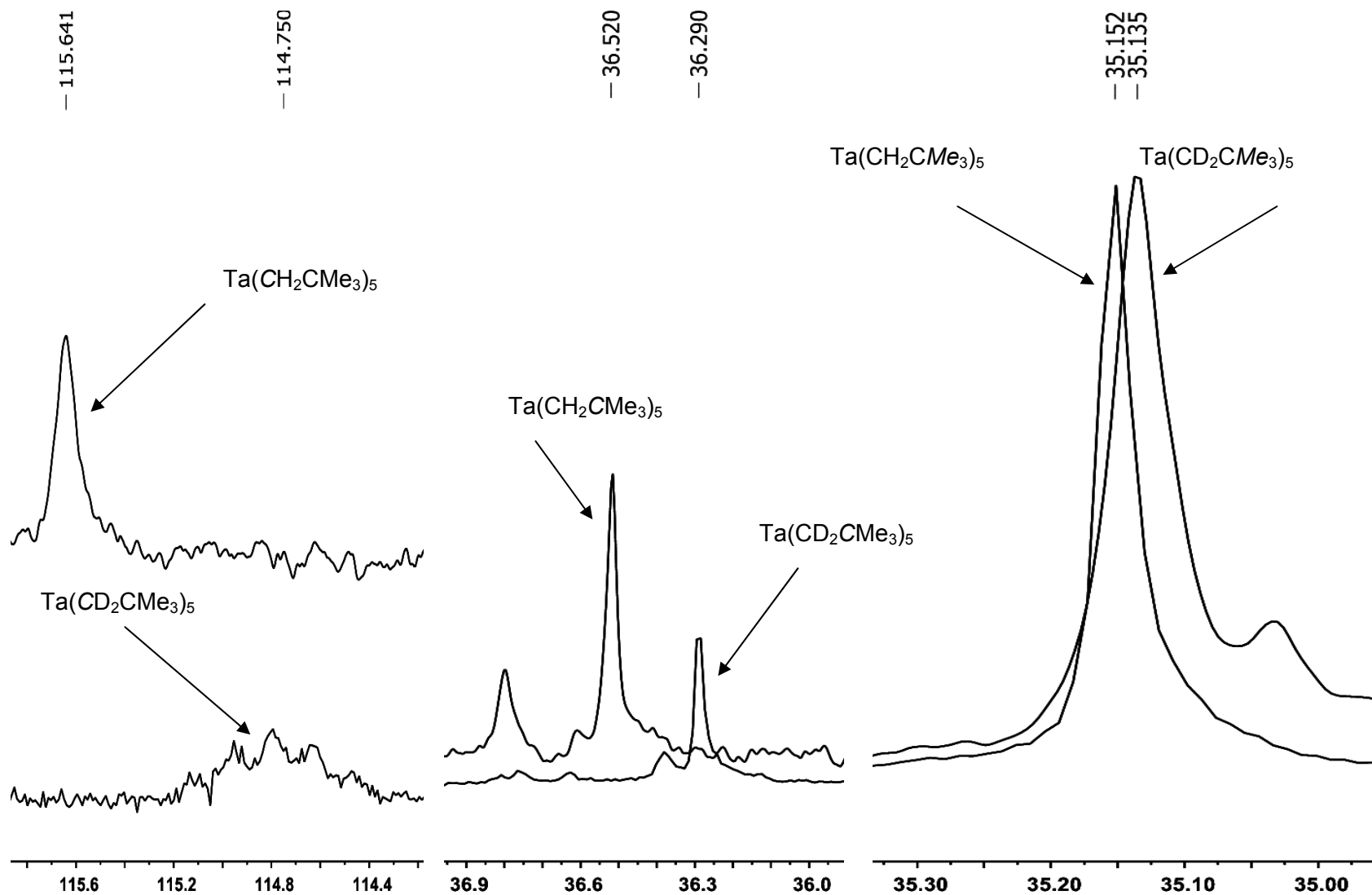
Figure 3.5. ^{13}\text{C} NMR spectrum of (\text{Bu}^t\text{CH}_2)_5\text{Ta} ( 1 ) and (\text{Bu}^t\text{CD}_2)_5\text{Ta} ( 1- d 10 ).
