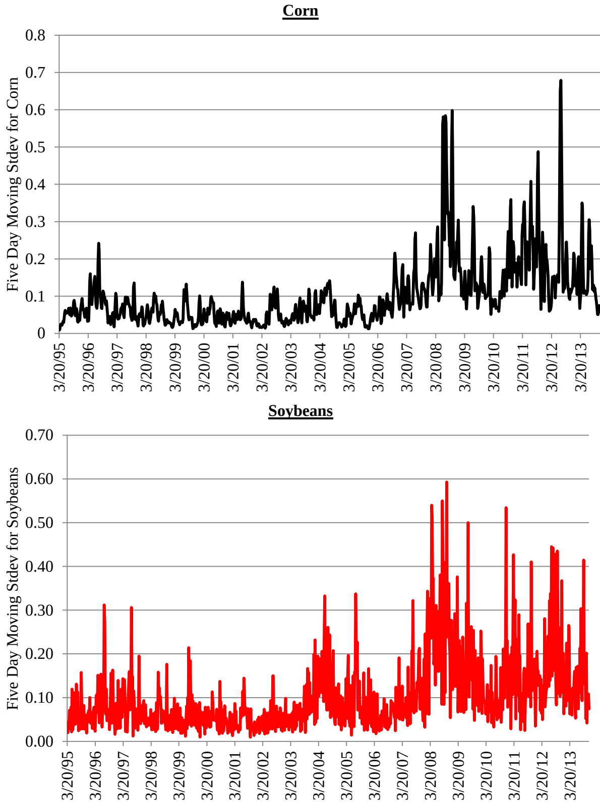
Figure 10. Five-day rolling standard deviation of weighted average price for corn and soybeans, nominal prices, Chicago Mercantile Exchange (CME), 1995-2013
