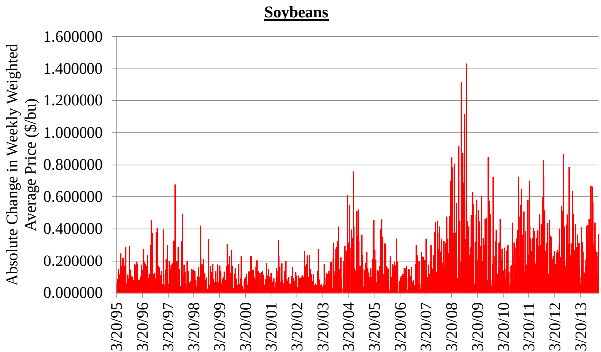
Figure 8. Absolute change in weekly average weighted average price for corn and soybeans, nominal prices, Chicago Mercantile Exchange (CME), 1995-2013
