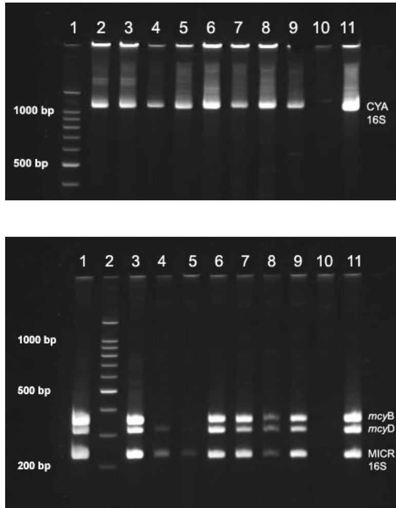
Figure 3. Gel image of multiplex PCR results. Gel A. Detection of cyanobacterial 16S rDNA fragment. Lane 1: 100 bp molecular weight marker; Lane 2: site 1a; Lane 3: site 1b; Lane 4: site 2; Lane 5: site 3; Lane 6: site 4; Lane 7: site 5; Lane 8: site 6; Lane 9: site 7; Lane 10: negative control, no template DNA; Lane 11: positive control ( M. aeruginosa LE-3 genomic DNA). Gel B: detection of Microcystis spp. 16S rDNA fragment and microcystin synthetase genes mcyB and mcyD . Lane 1: site 1a; Lane 2: 100 bp molecular weight marker; Lane 3: site 1b; Lane 4: site 2; Lane 5: site 3; Lane 6: site 4; Lane 7: site 5; Lane 8: site 6; Lane 9: site 7; Lane 10: negative control, no template DNA; Lane 11: positive control ( M. aeruginosa LE-3 genomic DNA).
