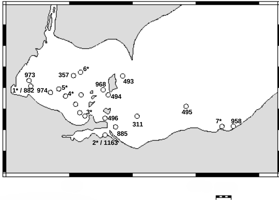
Figure 2. Sampling sites in 2003 and 2004. Sampling sites visited in 2003 are indicated with a number 1-7 and an asterisk. Stations were renumbered consecutively because different groups collecting samples used different coding system for the sampling sites. The sampling sites used in August 2004 are numbered according to Environment Canada station coding system consisting of 3 and 4 digit station numbers as indicated on the map.
