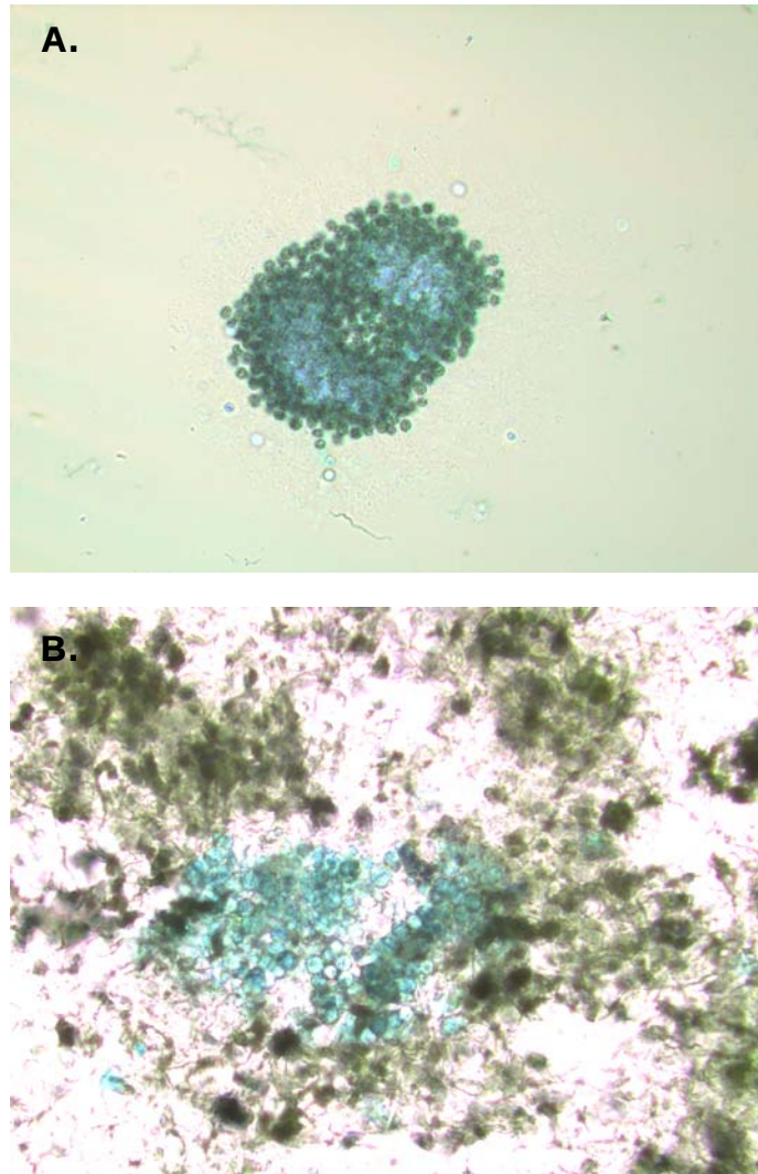
Figure 2. Light microscopy images of material cultured from Lake Erie sediment samples collected in 2006. Colonies with morphological characteristics consistent with Microcystis spp. were observed both in isolation (A.) and integrated amongst other cellular materials (B.).
