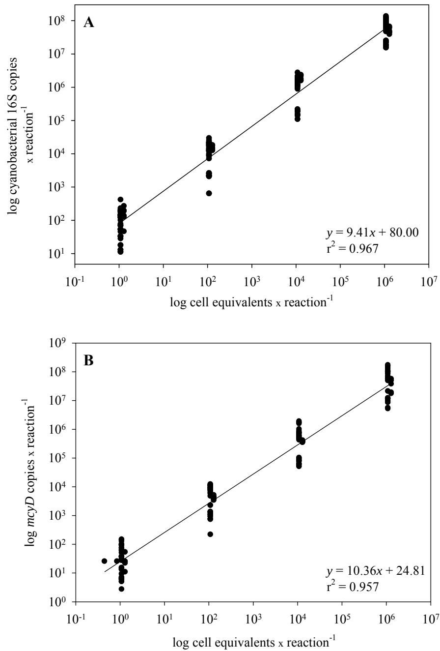
Figure 3. Linear regression between target gene copy abundance and Microcystis aeruginosa LE-3 cell equivalents. Graph A: Target gene cyanobacterial 16S rRNA gene. Graph B: target gene mcvD . Cell equivalents correspond to a quantity of DNA that was extracted from a known quantity of Microcystis aeruginosa LE-3 cells.
