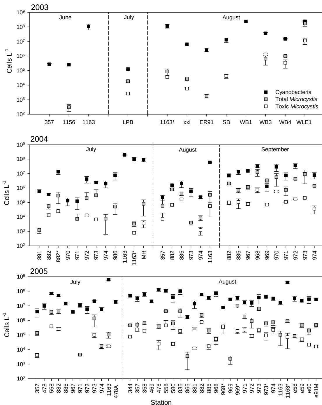
Figure 2. Cell abundances on western basin sampling locations in 2003-2005. Station numbers are organized according to their codes for each month. An asterisk indicates that same station was visited twice at separate times during one month. Error bars represent standard deviation among replicate assays (n=3).
