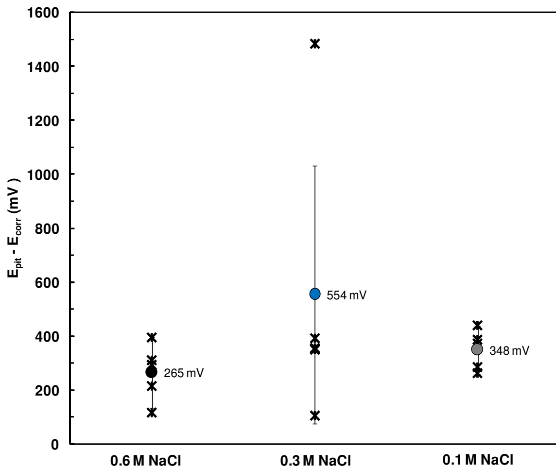
Figure 38. The pitting resistance parameters ( E_{\text{pit}} - E_{\text{corr}} ) of Vitreloy 105 as a function of chloride concentration. Circles and error bars represent mean values and 95% confidence intervals, respectively. Mean values are noted on the chart.
