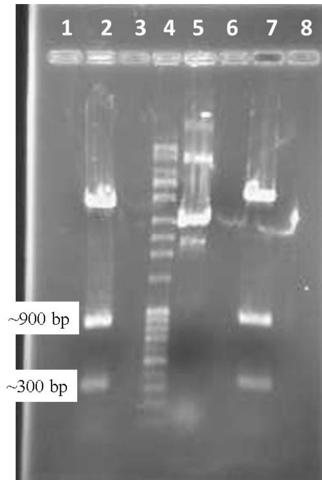
Figure 3-17 NdeI and XhoI digested glyA .
