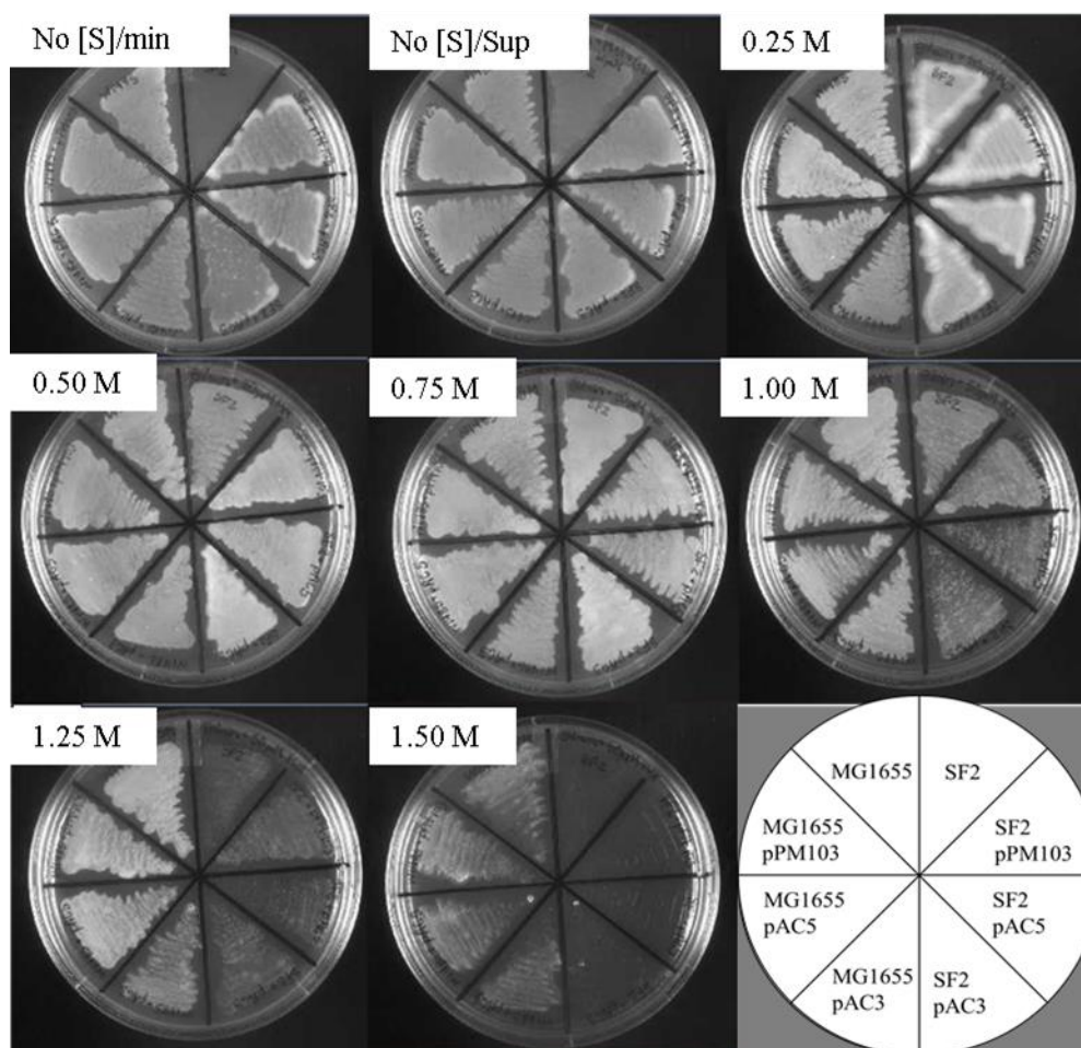
Figure 3-11 Assessing the effect of increasing osmolality on the ability of SF2 to grow in the presence of a sub-optimal methionine concentration.
