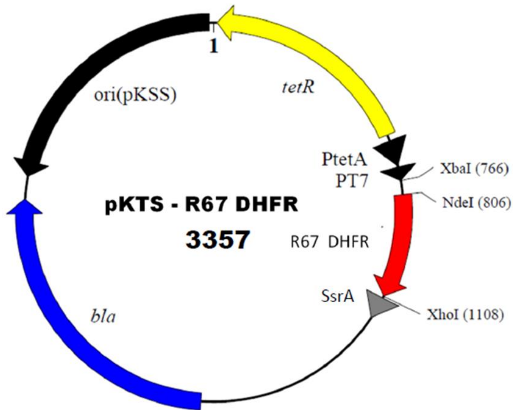
Figure 1-8 Map of the tunable vector pKTS
