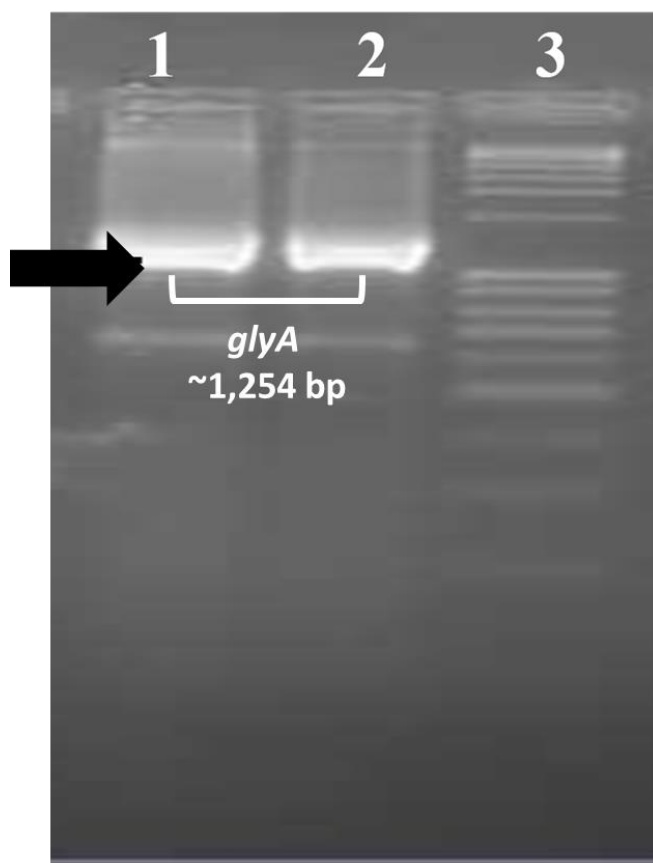
Figure 3-16 glyA PCR product.
