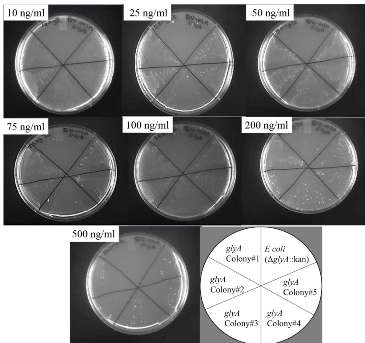
Figure 3-20 Tetracycline dependent glyA production.
