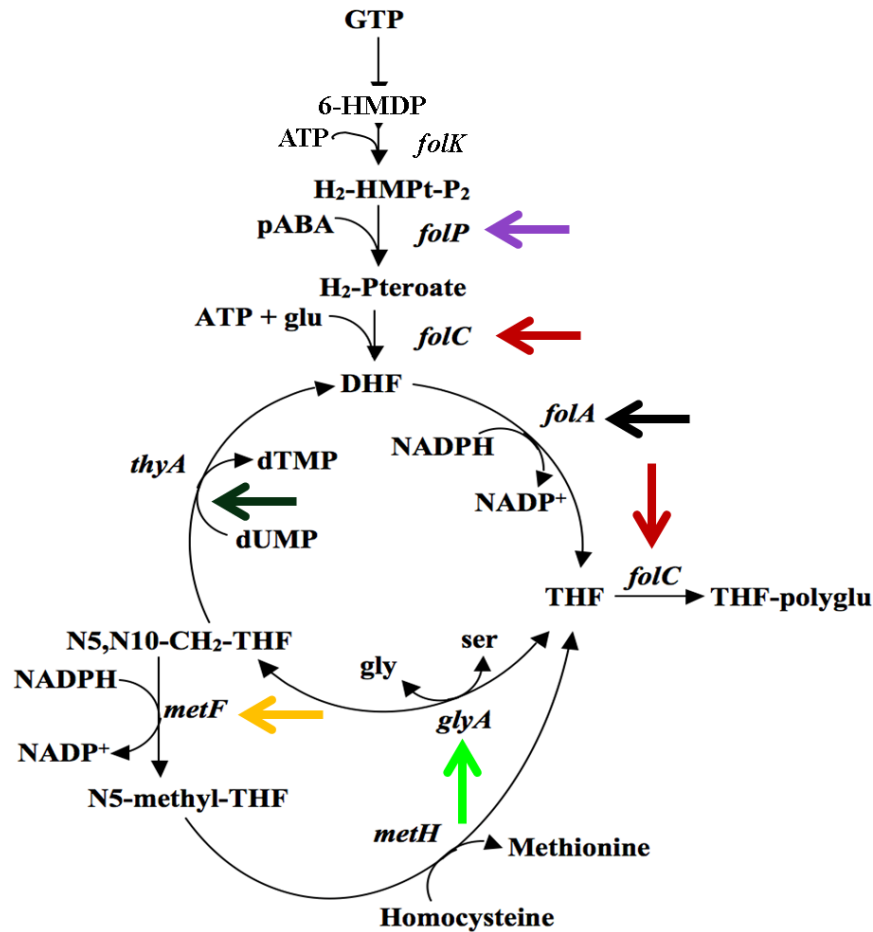
Figure 1-10 Simplified Model of Folate Cycle : Selected enzymes showed in arrows.
