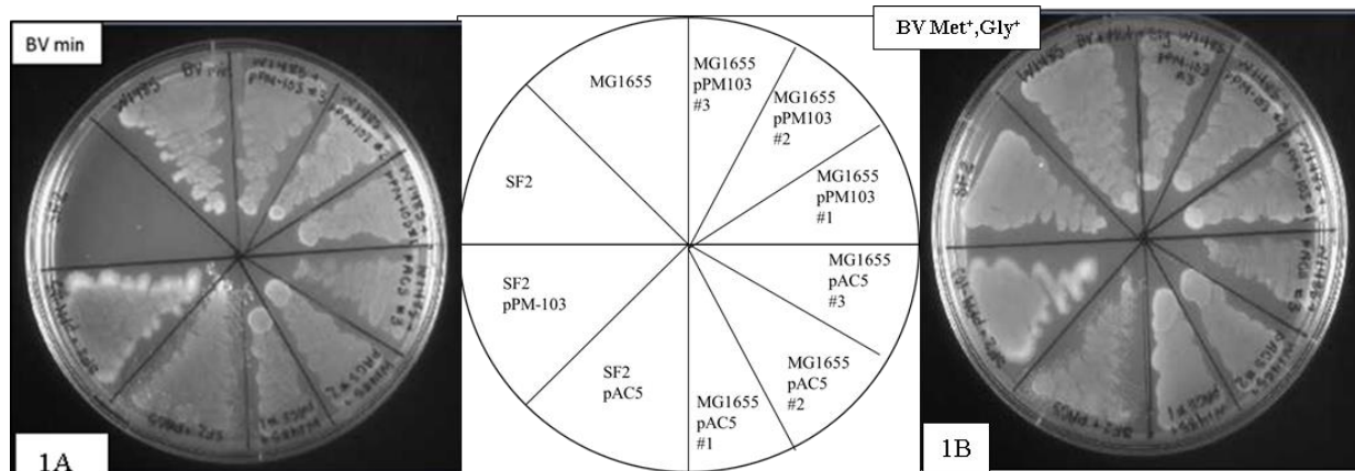
Figure 3-9 The growth pattern of the folC mutant strain, SF2, and its parent strain MG1655. Panel A shows their growth patterns on BV minimal agar while panel B shows the growth of on a BV plate supplemented with 50 µg methionine/ml and 50 µg glycine/ml plates. SF2 did not grow on BV minimal media. However, both SF2 carrying a functional folC gene and the parent strain grew on BV minimal and supplemented plates. The middle panel shows how the various cultures were streaked on the plates.
