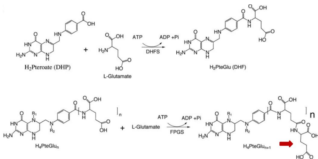
Figure 1-14 Two reactions-one enzyme: bifunctional FPGS.
