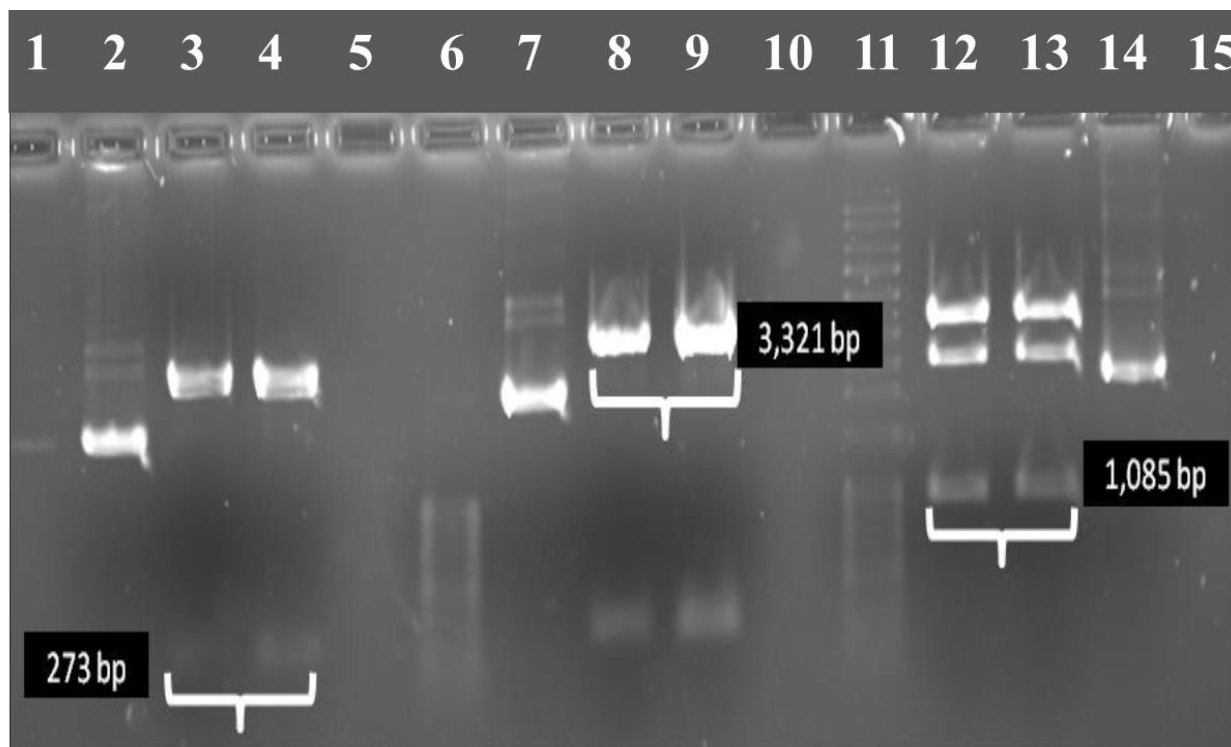
Figure 3-1 Restriction enzyme digested R67 DHFR, pKTS. and pKTS DNA Lane 2: uncut R67 DHFR-pUC57, Lanes 3 and 4: NdeI and XhoI digested clone, insert size = 273bp. Lane7: uncut chorismate mutase-pKTS, Lanes 8 and 9: NdeI and XhoI digested chorismate mutase-pKTS (3,321 bp). Lanes 12 and 13: NdeI and XhoI digested Quad4-pUC75 clone, insert size 1,085 bp, Lane14 uncut Quad4-pKTS. The DNA samples were separated on a 1% agarose gel. DNA ladders are also shown in lane 6 and 11 (100 bp and 1000 bp plus, respectively). Brackets show the bands used in cloning.
