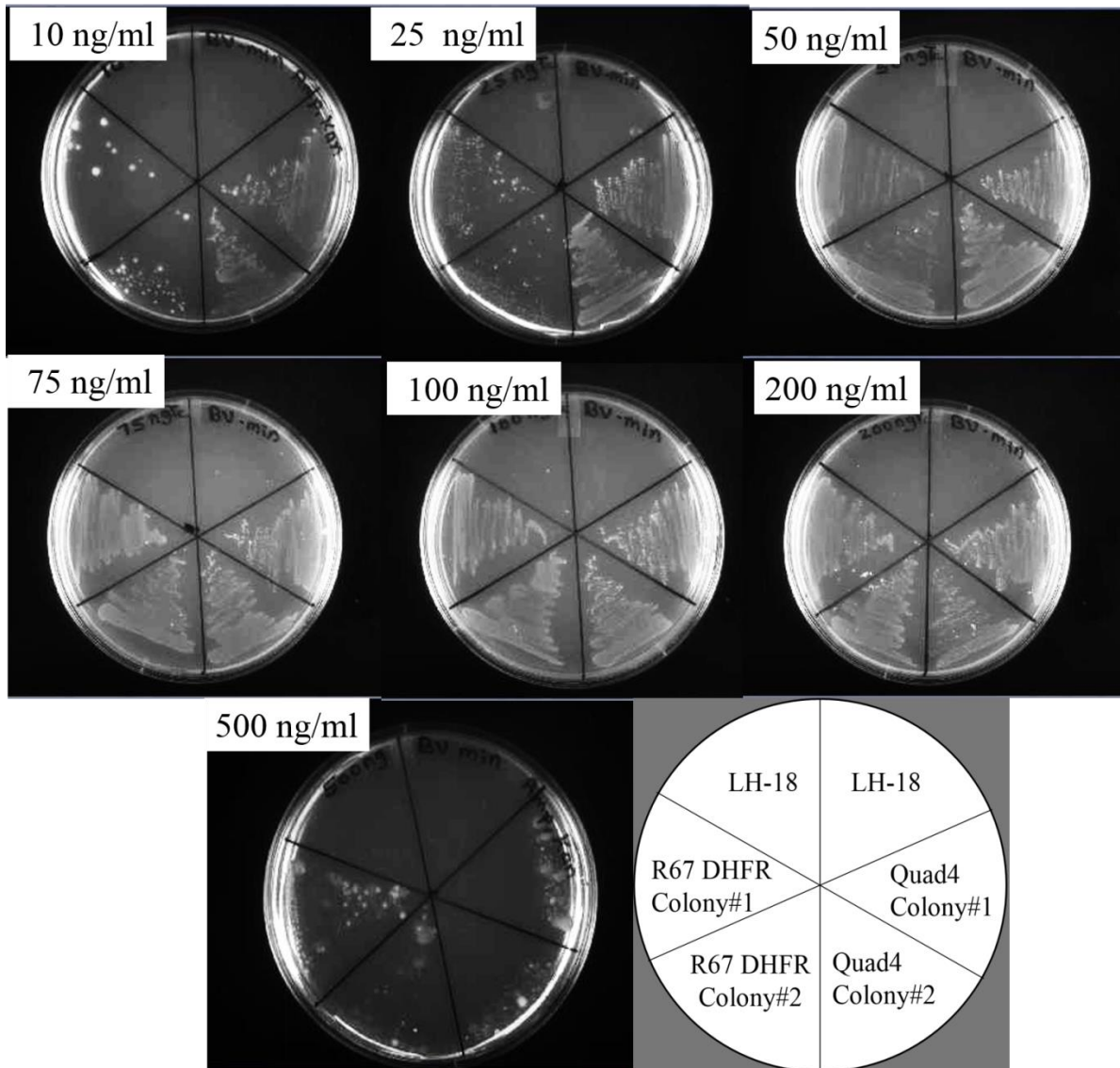
Figure 3-4 Tetracycline dependent E. coli LH-18 growth on BV minimal media The optimal tetracycline concentration required to induce the P_{tet} promoter to support confluent cell growth was determined on BV minimal media containing 200 \mu g ampicillin/ml, 25 \mu g/ml kanamycin and various concentrations of tetracycline. The cartoon on the lower right shows how the constructs are streaked on the plates.
