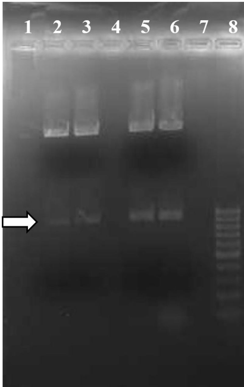
Figure 3-21 NdeI and XhoI digested folP .
