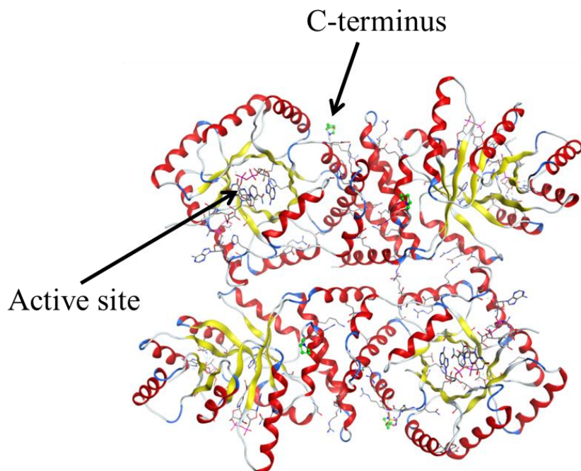
Figure 1-17 Crystal structure methylene-tetrahydrofolate reductase MTHFR MTHFR is a tetramer (PDB:1ZPT), the active site and C-terminus of a monomer is labeled. The distance between the active site and C-terminus is \geq 25 \text{ \AA} [32]. The figure was constructed using MOE version 2012.10 [30]
