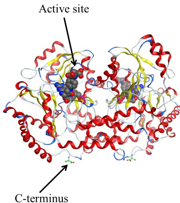
Figure 1-19 Crystal structure Serine hydroxymethyltransferase (SHMT) SHMT is a dimer (PDB:1DFO). One active site and C-terminus (shown in green) are labeled. The distance between the active site and the C-terminus is \geq 25 Å. The figure was constructed using MOE, version 2012.10 [30]
