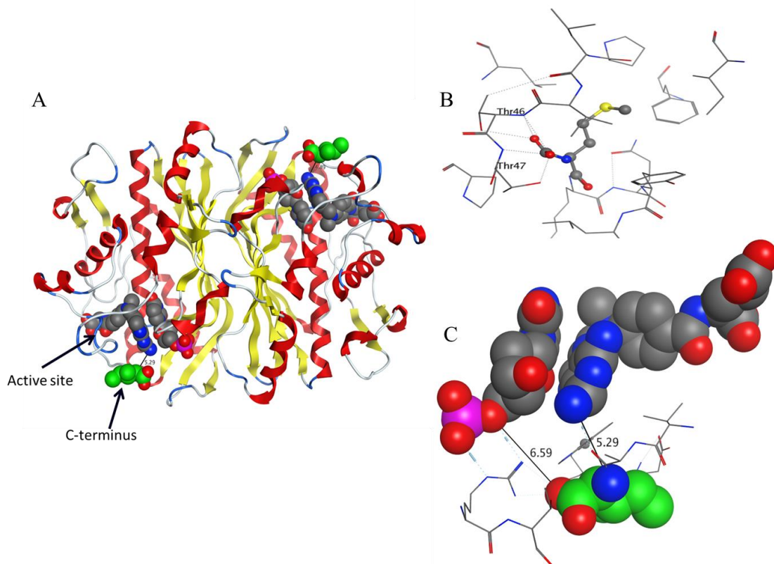
Figure 1-23 Crystal structure thymidylate Synthase (TS)
