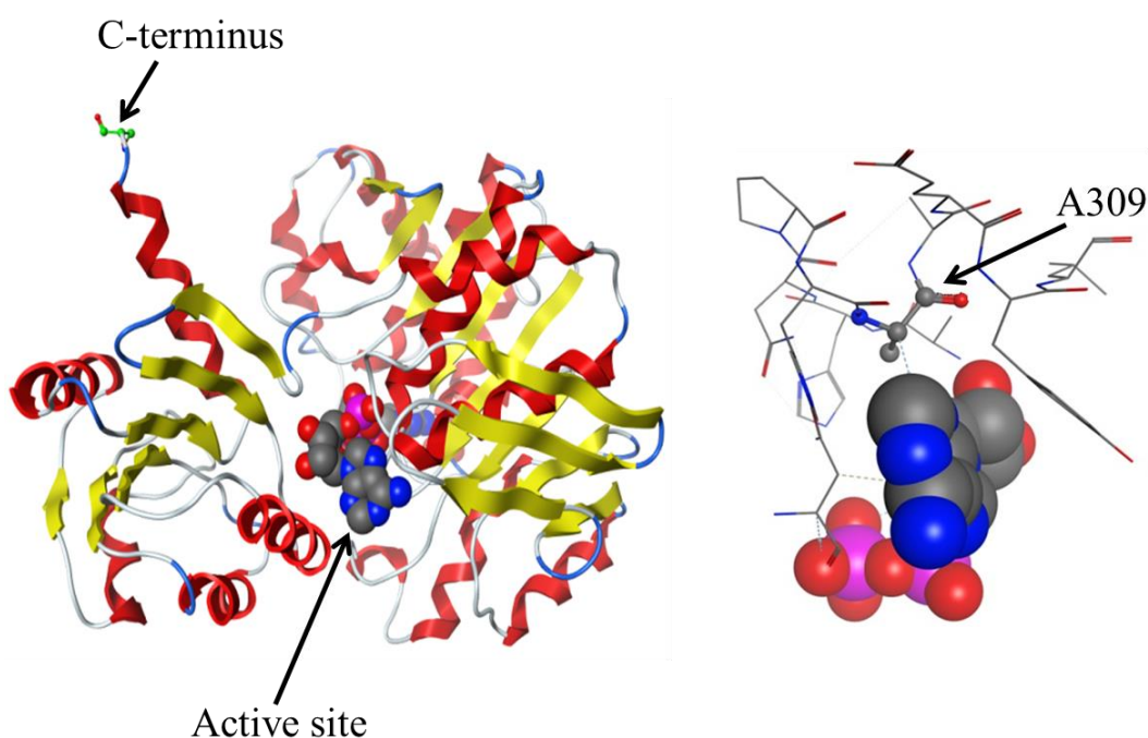
Figure 1-15 The structure of FPGS and the position of SF2 mutation FPGS is a monomer (PDB:1W78) [34]. Left image: the active site and the C-terminus are labeled. The distance between the active site and the C-terminus is \geq 26 Å. Right image: The E. coli SF2 strain contains a G925A mutation in the FolC gene corresponding to an A309T mutation in FPGS. The figure was constructed using MOE, version 2012.10 [30].
