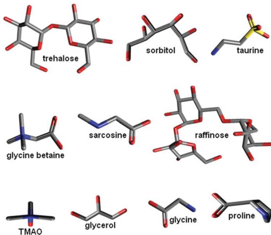
Figure 1-6 Chemical structures of selected naturally occurring osmolytes. Adopted from [11].
