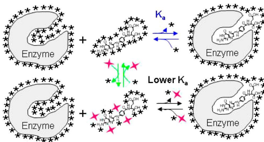
Figure 1-5 Model showing the preferential interaction of osmolytes with free DHF.
