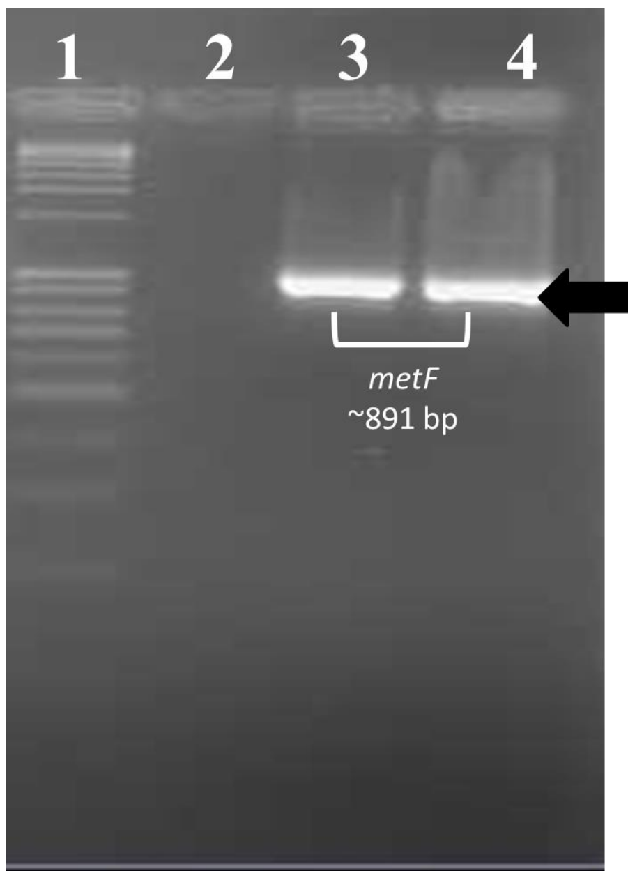
Figure 3-12 PCR amplification of the metF gene.
