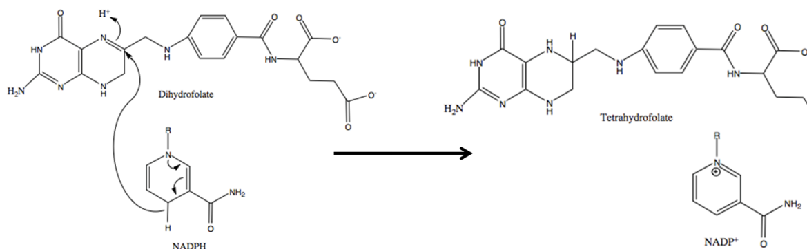
Figure 1-11 R67 Dihydrofolate reductase activity.
