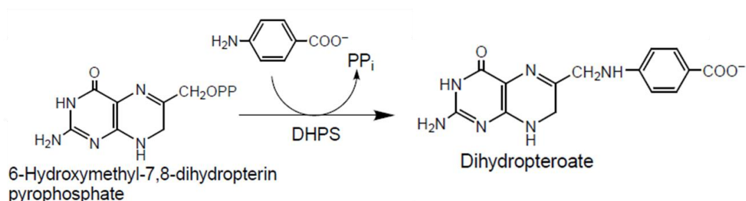
Figure 1-20 Dihydropteroate synthase (DHPS) attached pterin with pABA This enzyme joins the activated 6-hydroxymethyl-7,8-dihydropterin pyrophosphate (DHPPP) with para-amino benzoic acid (pABA) to produce 7, 8-dihydropteroate [57].
