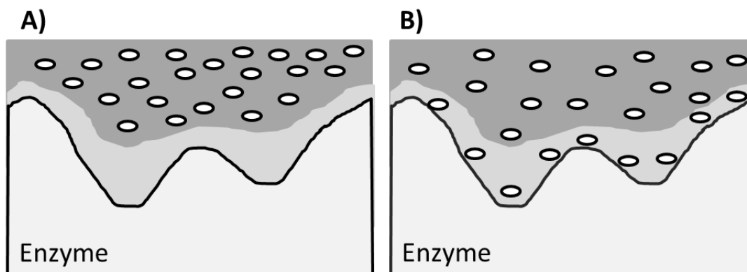
Figure 1-2 Models of preferential exclusion and B. preferential interaction. The enzyme surface layer is shown in light grey, while the bulk solvent is dark grey. Osmolytes are represented by white ovals [7]
