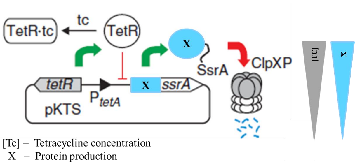
Figure 1-9 pKTS : selection strategies for controlling intracellular [catalyst] The gene of interest, ‘X’, is cloned between the P_{tetA} promoter and a sequence encoding a SsrA tag. The pKTS plasmid permits transcriptional control and limits enzyme half-life. The SsrA sequence is fused to the C-terminus of the protein of interest. Minimizing protein production should allow an in vivo selection of folate pathway enzyme activity [4].
