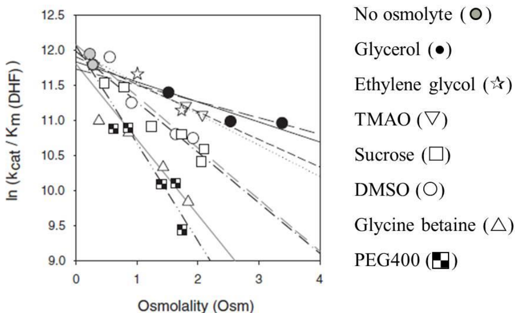
Figure 1-4 A plot of osmolality versus \ln k_{cat}/K_m(DHF) for R67 DHFR. Steady state kinetic data were obtained at saturating NADPH concentration and varied DHF concentrations in the presence of various osmolytes. Michaelis-Menten plots were used to calculate k_{cat} and K_m(DHF) values. The units for k_{cat}/K_M(DHF) are s^{-1} M^{-1} . Adopted from [1].
