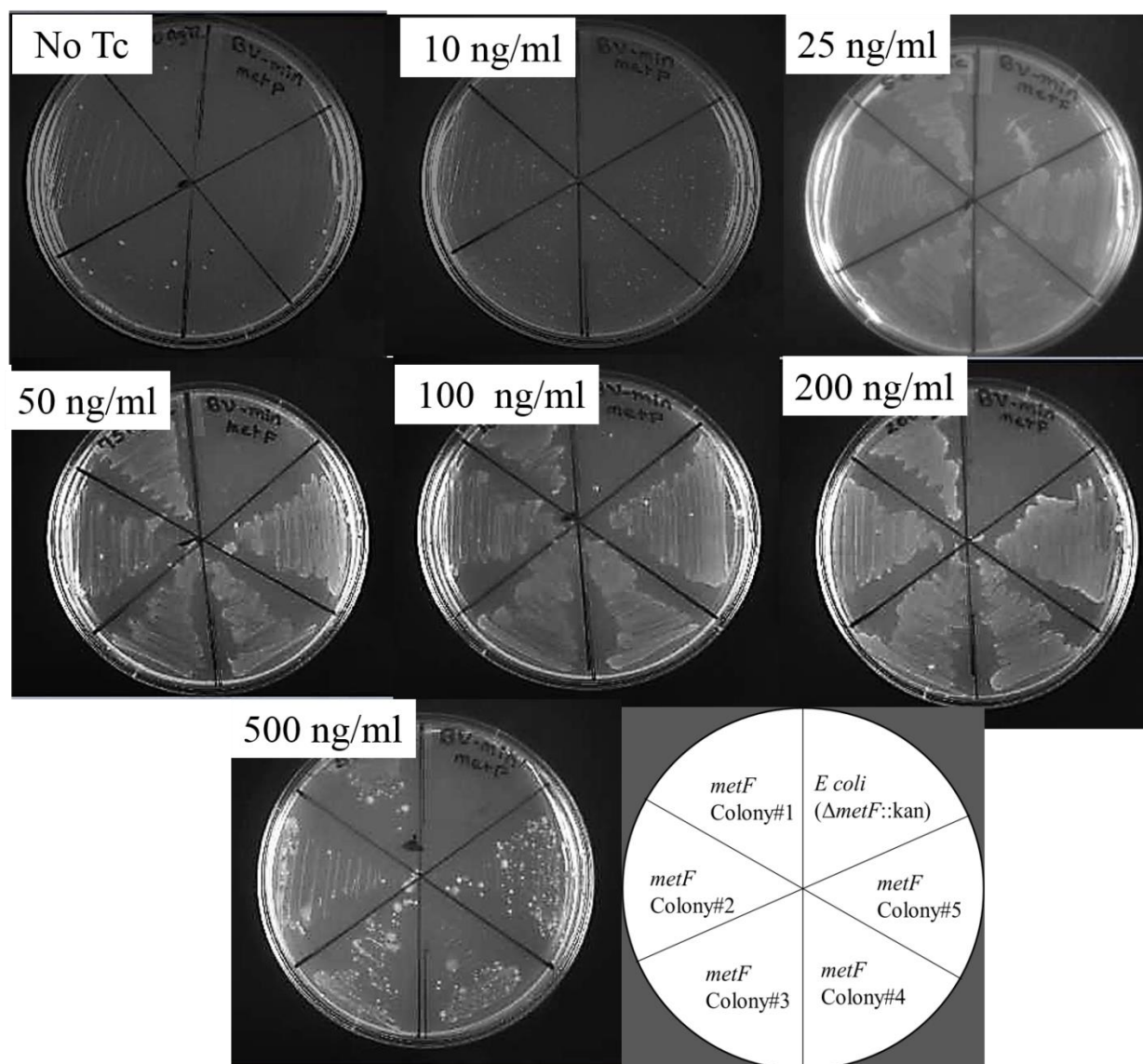
Figure 3-15 Tetracycline dependent metF production rescues JW3913-1 ( \Delta metF::kan ) carrying the metF -pKTS plasmid.
