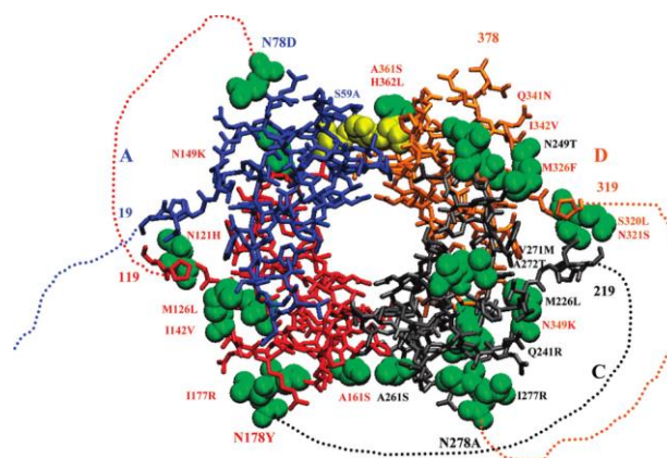
Figure 1-13 Quadruplicated construct of R67 DHFR: Quad4.
