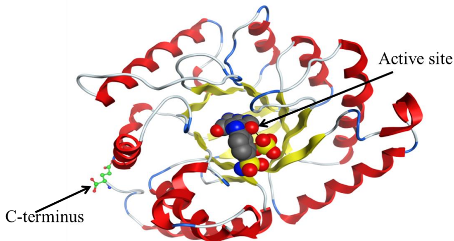
Figure 1-21 Crystal structure Dihydropteroate synthase (DHPS) DHPS is a monomer, the active site and C-terminus are labeled (PDB: 3KUH). The distance between the active site and C-terminus is \geq 22\ \text{\AA} . DHPS is also of interest as it provides resistance to sulfa drugs. The figure was constructed using MOE version 2012.10 [30].
