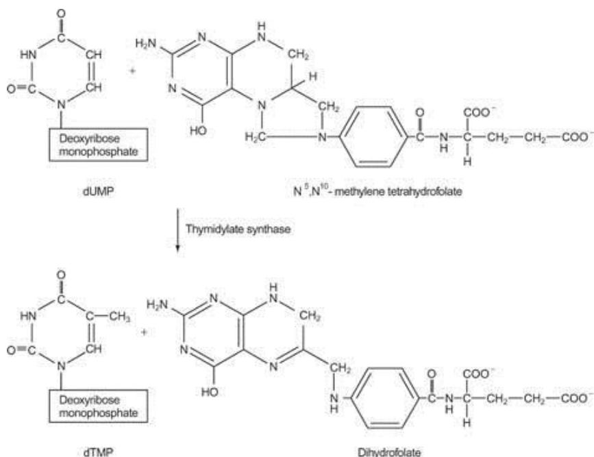
Figure 1-22 Thymidylate synthase (TS) plays a major role DNA synthesis. This enzyme catalyzes the conversion of deoxyuridine monophosphate (dUMP) to deoxythymidine monophosphate (dTMP) using 5,10-methylene tetrahydrofolate (CH 2 THF) as a methyl group donor. From: http://www.cliffsnotes.com/sciences/biology/biochemistry-ii/purines-and-pyrimidines/deoxynucleotide-synthesis
