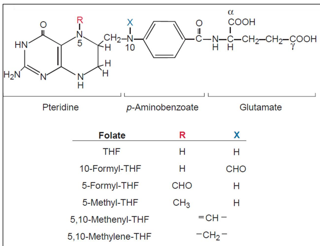
Figure 1-1 Folate contains pterin, pABA and glutamate moieties.
