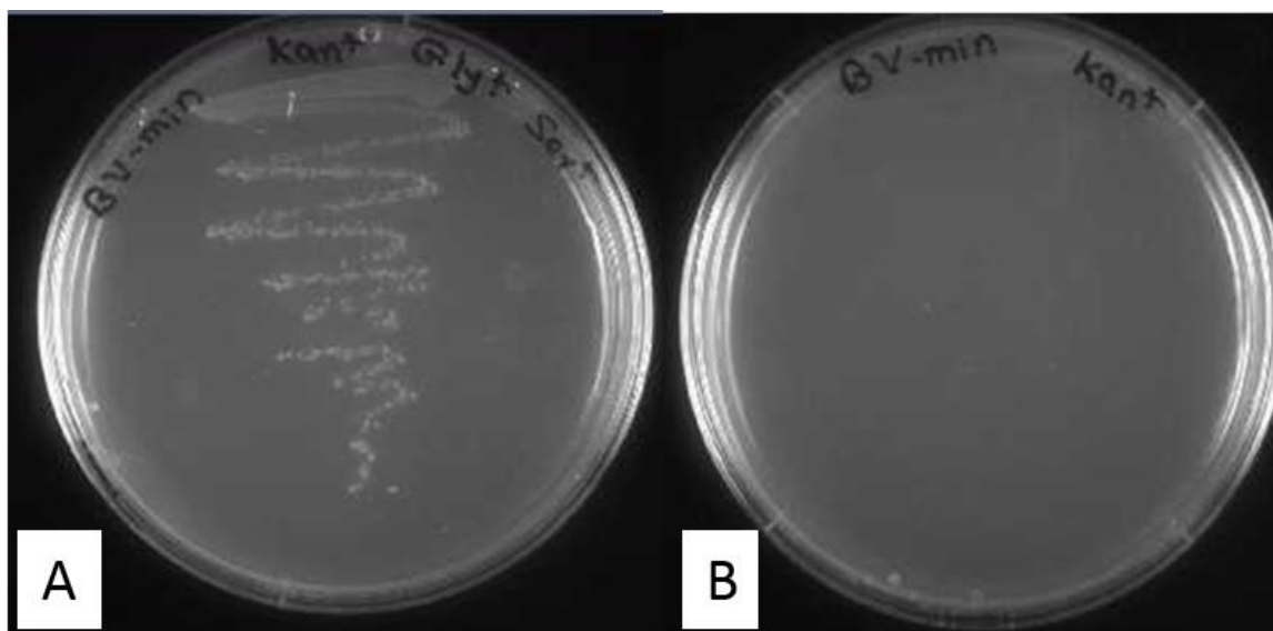
Figure 3-19 The growth pattern of E. coli JW2535-1 ( \Delta glyA::kan).
