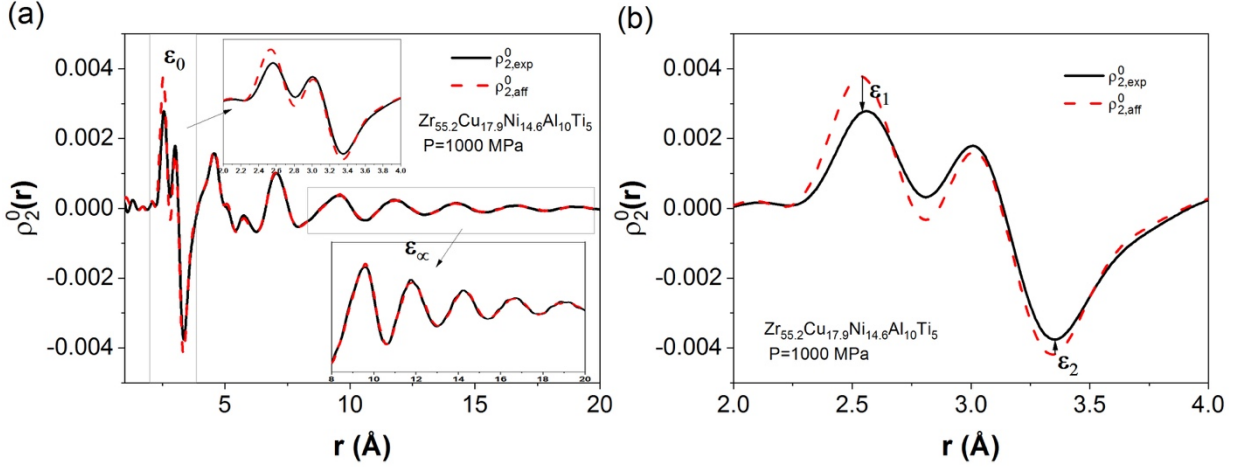
Figure 4.1 (a) The fitting of the experimental anisotropic PDF with the affine anisotropic PDF. (b) local r -dependent strain.
