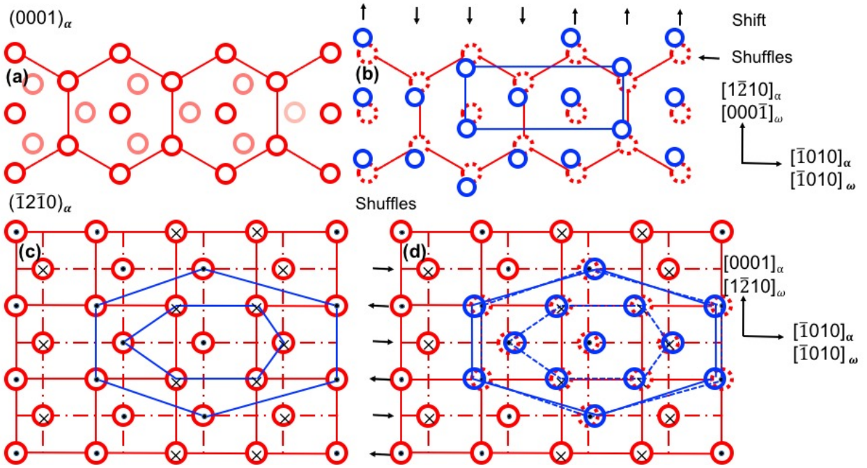
Figure 5.1 Atomistic model of direct \alpha to \omega phase transition in pure Zr proposed by Rabinkim et al. [120]. (a) This shows the two (0002)_{\alpha} stacking planes of the \alpha phase (the light red circles are the Zr atoms on the below (0002)_{\alpha} plane). (b) After the shifts and shuffles, the blue circles are the displaced Zr atoms that formed the (\bar{1}2\bar{1}0)_{\omega} plane from (0002)_{\alpha} plane. (c) The (\bar{1}2\bar{1}0)_{\alpha} plane of the \alpha phase. The dot and cross in the atom shows the shuffle direction of it (outside or inside the paper). (d) The shuffle along the [\bar{1}010]_{\alpha} direction forms a distorted (0001)_{\omega} plane from (\bar{1}2\bar{1}0)_{\alpha} plane.
