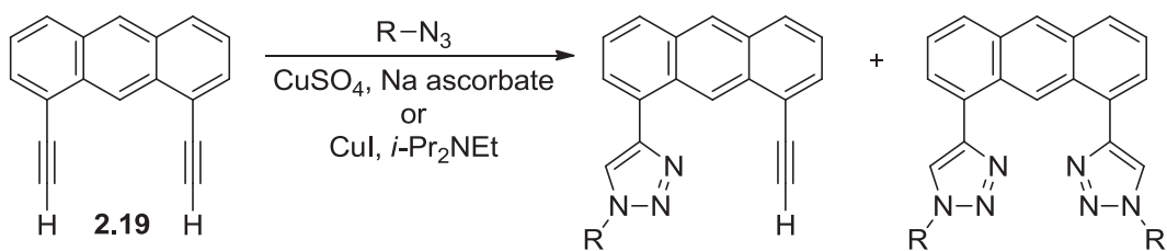
Scheme 2.7. Attempted cycloaddition between 2.19 and various azides.
