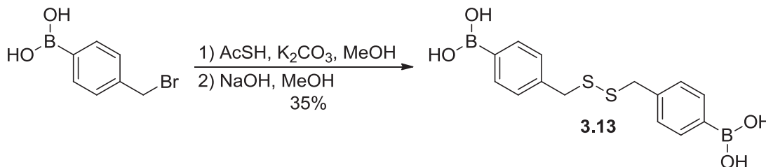
Scheme 3.7. Synthesis of phenylboronic acid disulfide 3.13 .
