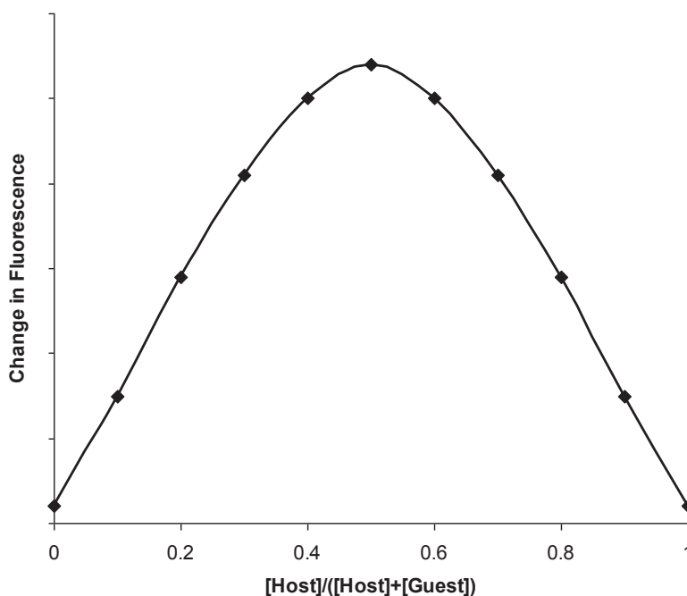
Figure 1.5. Typical Job plot for a 1:1 host–guest complex.
