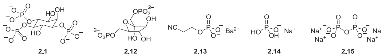
Figure 2.6. Structures of guests used for binding studies.
