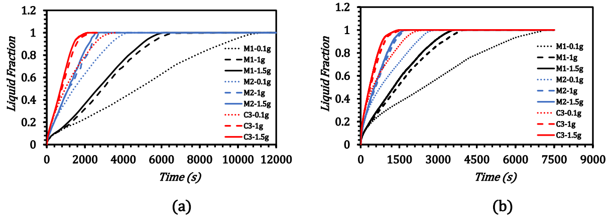
Fig.3.11 Liquid Fraction Comparison v/s time at various gravity conditions for novel configuration 'C3' with m1 and m2 for (a) RT82 and (b) RT35
