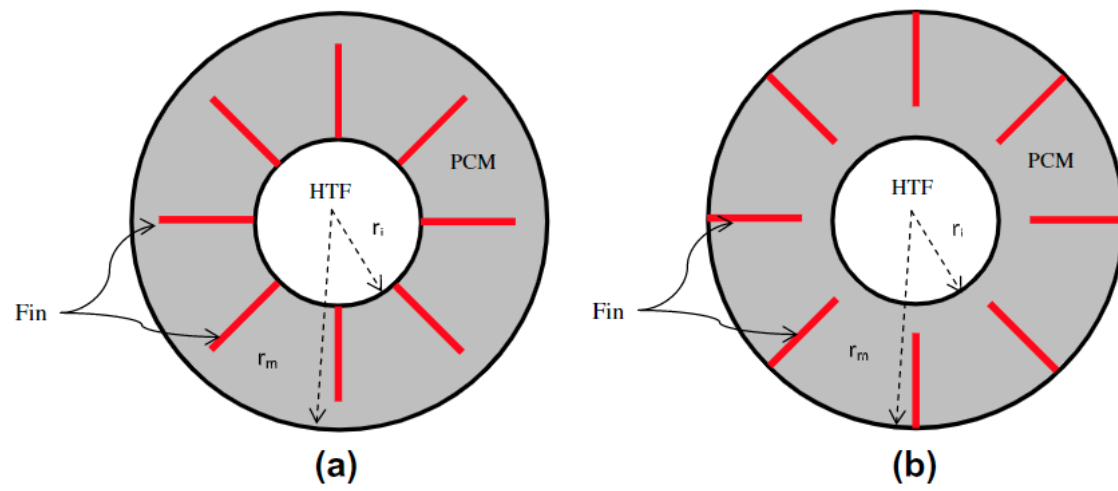
Fig. 1.10 Geometric Configurations in Mat et.al. (a) A Finned Tube and (b) An Internally Finned tube [62]
