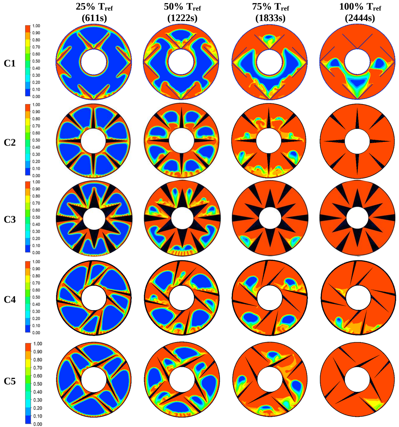
Fig.3.4 Liquid Fraction contours for Novel Configurations C1-C5 at specific time intervals relative to reference time for melting of RT-82
