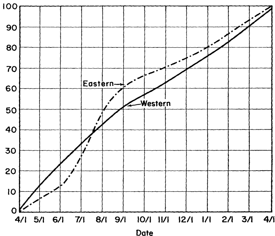
Figure 3. Cumulative monthly distribution of erosion potential in eastern and western Tennessee.
